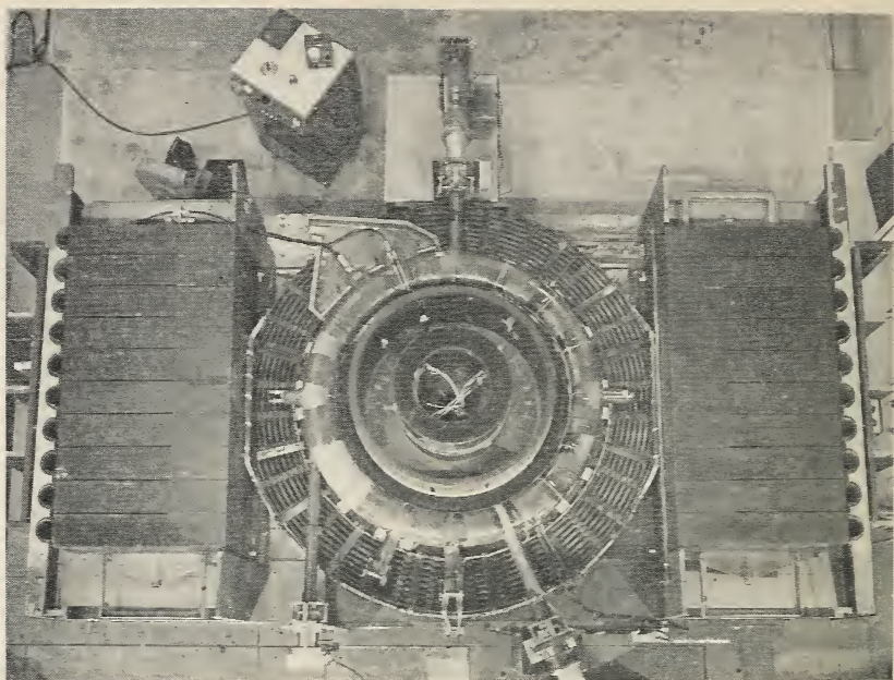
Far ultraviolet light is transmitted through tangential port (left-foreground) of donut resting on magnet of NBS Synchrotron—seen here from above.
