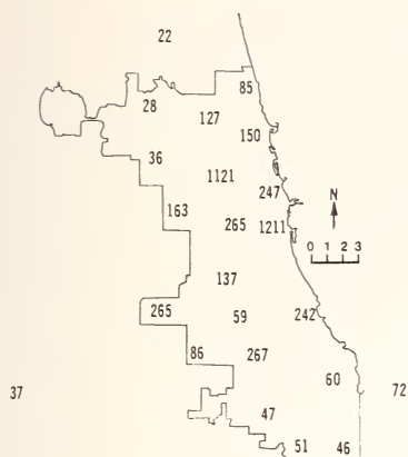
Figure 6. Distribution of vanadium 10^{-10} g/m 3 .
