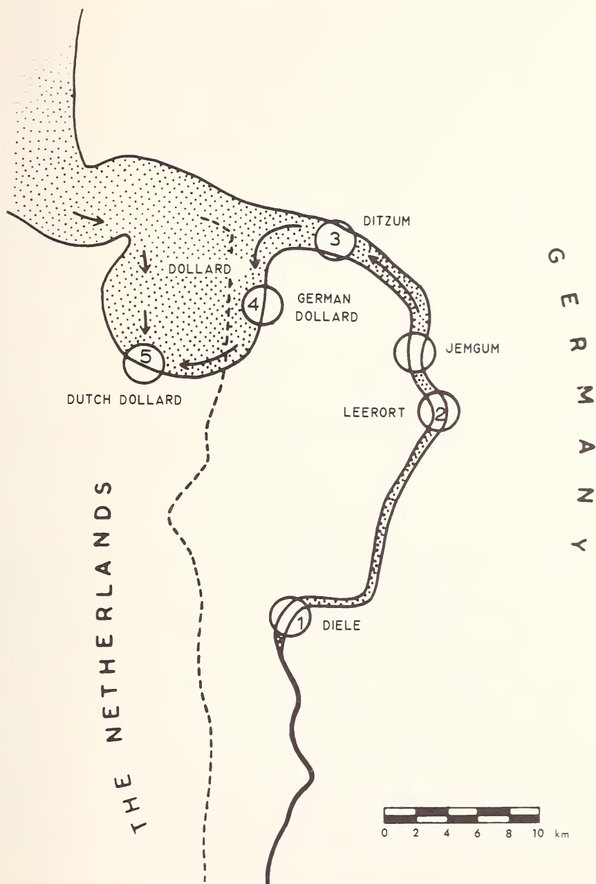
Figure 4. Ems delta (Germany), movement of sediments.
