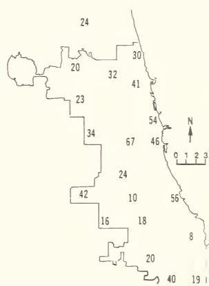
Figure 9. Distribution of sodium 10^{-8} g/m 3 .
