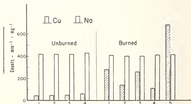
Figure 6. Copper and sodium activities of irradiated skin specimens.
