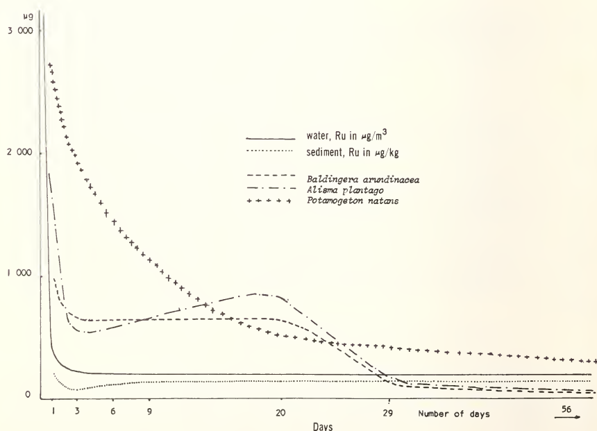
Figure 5. Ruthenium concentration in a plant aquatic ecosystem, after an enrichment in ammonium aquochlororuthenate. (Results in \mu\text{g/kg} of dry matter.)
