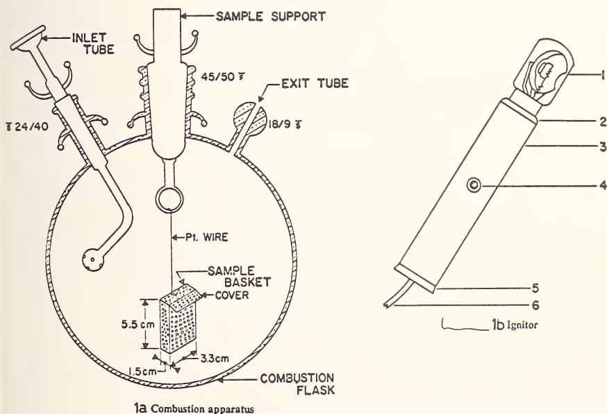
Figure 1. Schöniger-type combustion apparatus (1a) and ignitor (1b). 1. Sylvania DFC. DFN, projector lamp, 2. Amphenol 7854-type standard socket, 3. Plastic tubing, 1 1/8-inch i.d., 7 inches in length, 4. Normally open type push-button switch, 5. No. 6 rubber stopper drilled to accommodate electrical wiring, 6. Electrical wiring. (Reproduced with permission from reference [12])
