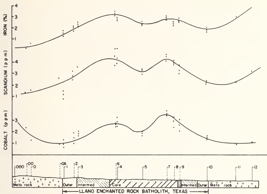
Figure 6. Distribution of iron, scandium and cobalt across the Llano Enchanted Rock Batholith, Texas.
