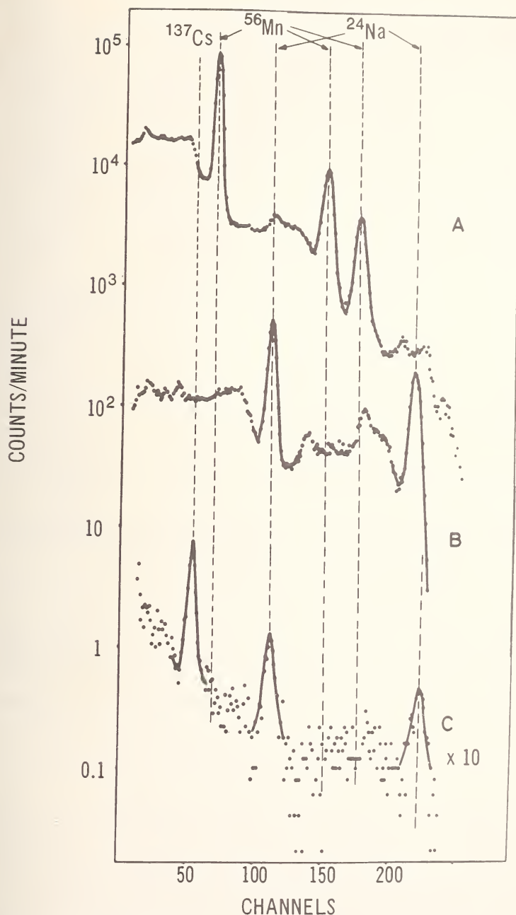
Figure 5. Decontamination obtained on ^{56}\text{Mn} -rich biological specimens. A. Before chemical separation. Trace quantities of ^{137}\text{Cs} have been added. B. After passage on an MDO column. C. After passage on an ammonium phosphomolibdate column.
