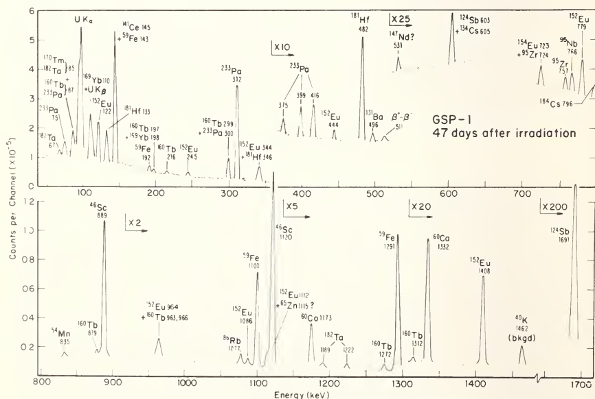
Figure 1. Spectrum of gamma-rays from GSP-1 observed with 30 \text{ cm}^3 Ge(Li) detector 47 days after neutron irradiation.
