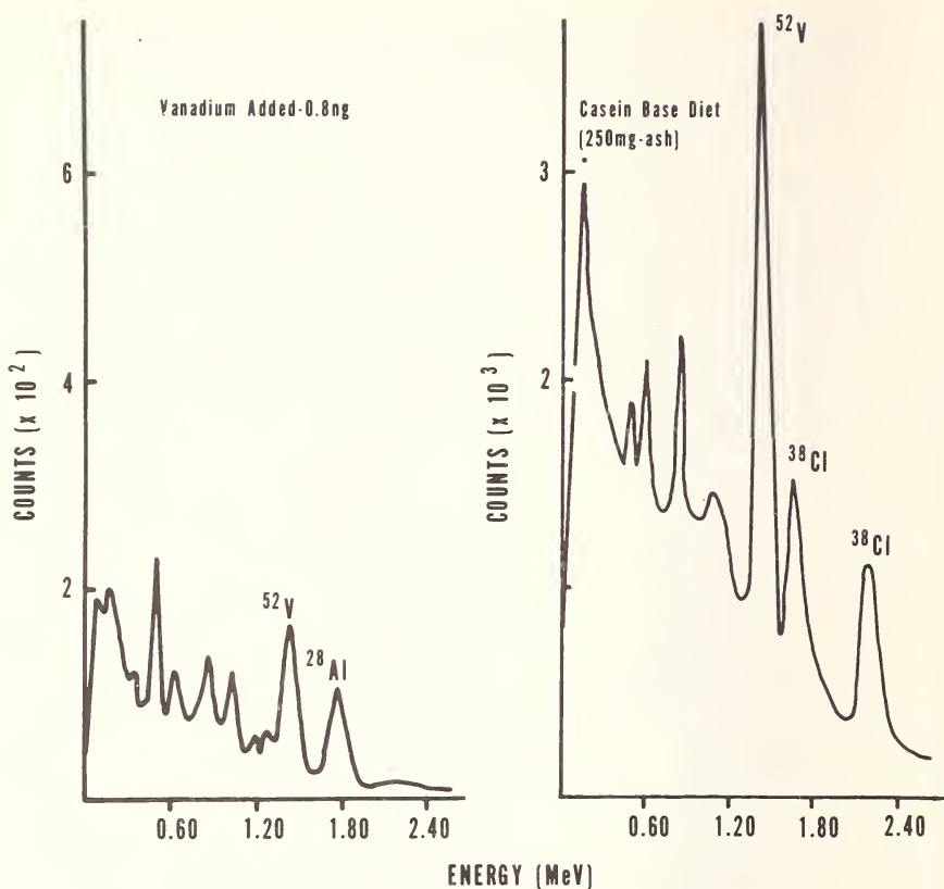
Figure 2. Gamma-ray spectra of 52 V spectral interferences.
