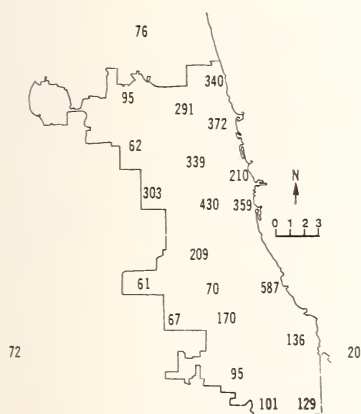
Figure 8. Distribution of chlorine 10^{-8} g/m 3 .
