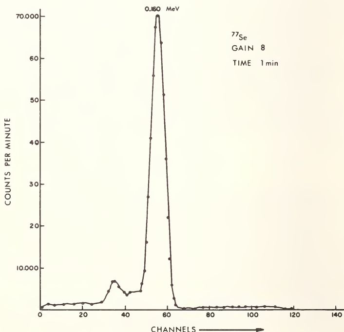
Figure 1. Gamma-ray spectrum of 77 Se.
