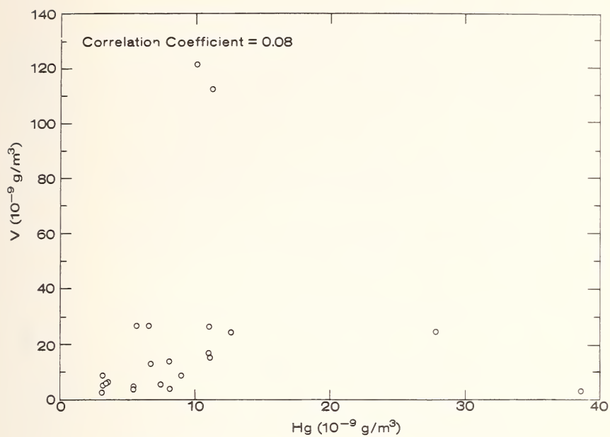
Figure 12. Mercury vs vanadium correlation in air.
