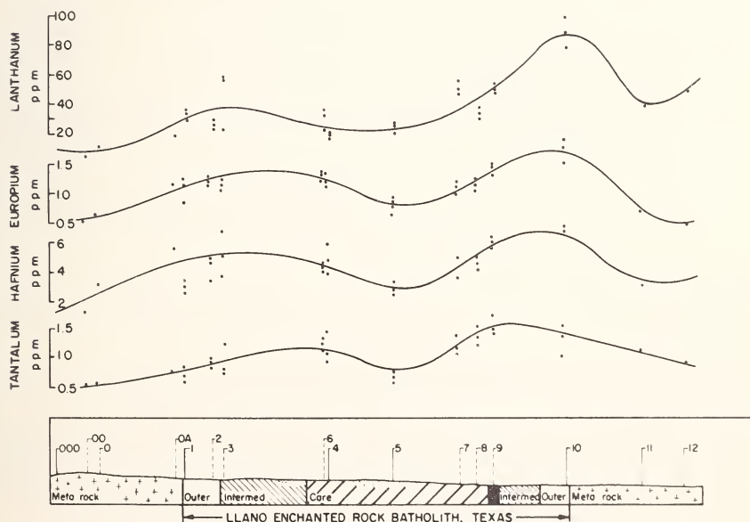
Figure 7. Distribution of lanthanum, europium, hafnium and tantalum across the Llano Enchanted Rock Batholith, Texas.
