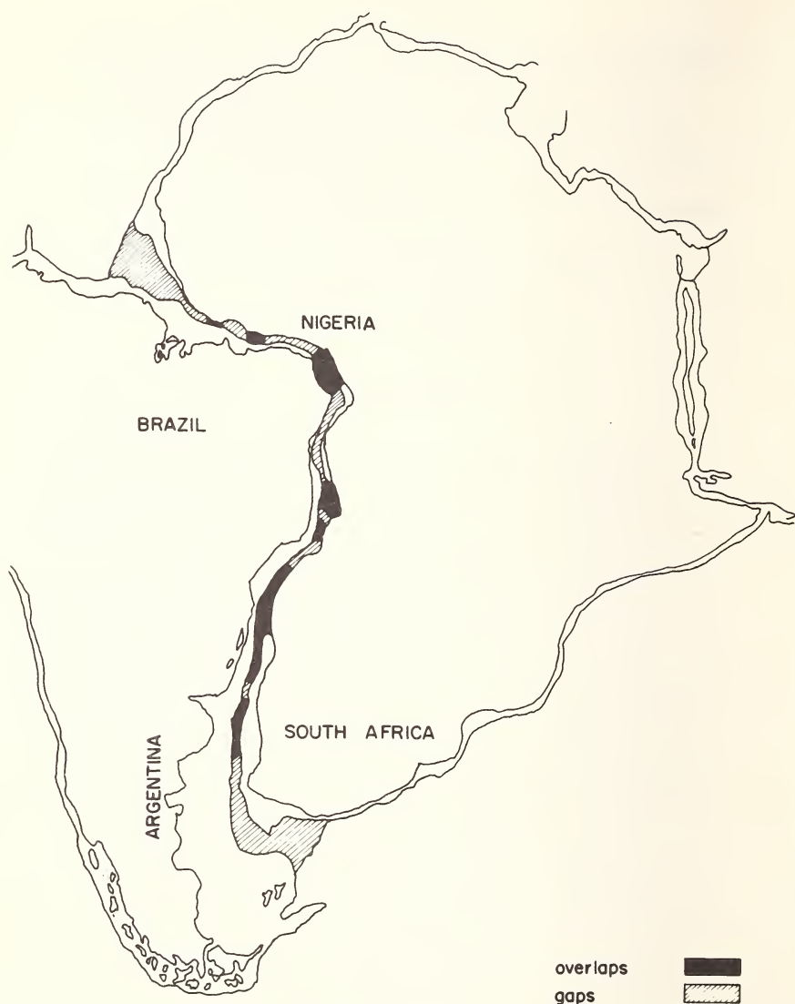
Figure 1. Least squares fit of the shelves of Africa and South America, by Sir E. Bullard.
