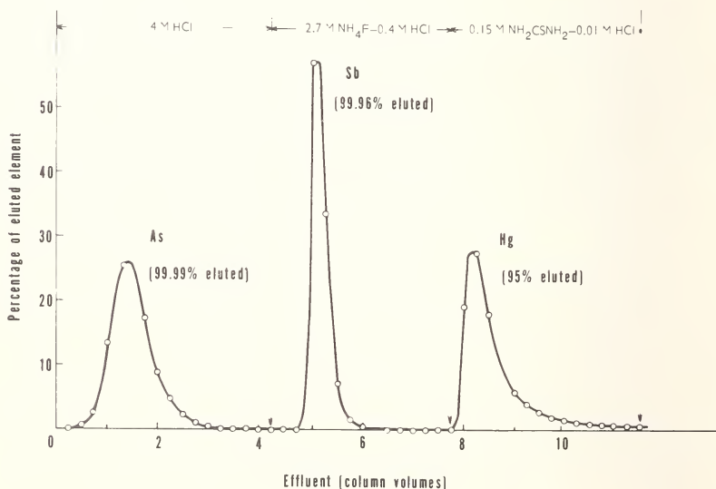
Figure 2. Chromatographic separation of arsenic, antimony, and mercury on column Dowex 1x8 100-200 mesh 1.1 \text{ cm}^2 \times 10 \text{ cm} ; 11 \text{ cm}^3 , flow rate = 1.5 to 2 \text{ ml} \cdot \text{cm}^{-2} \cdot \text{sec}^{-1} .
