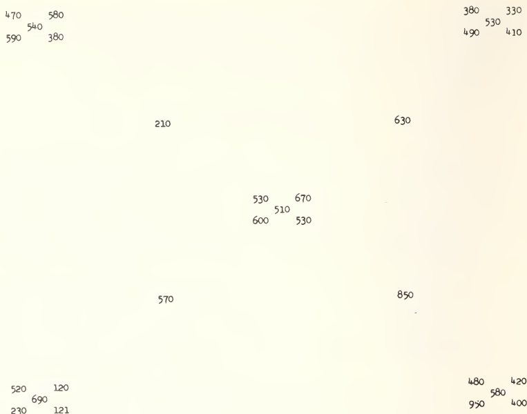
Figure 2. Manganese distribution in Dallas collection grid.
