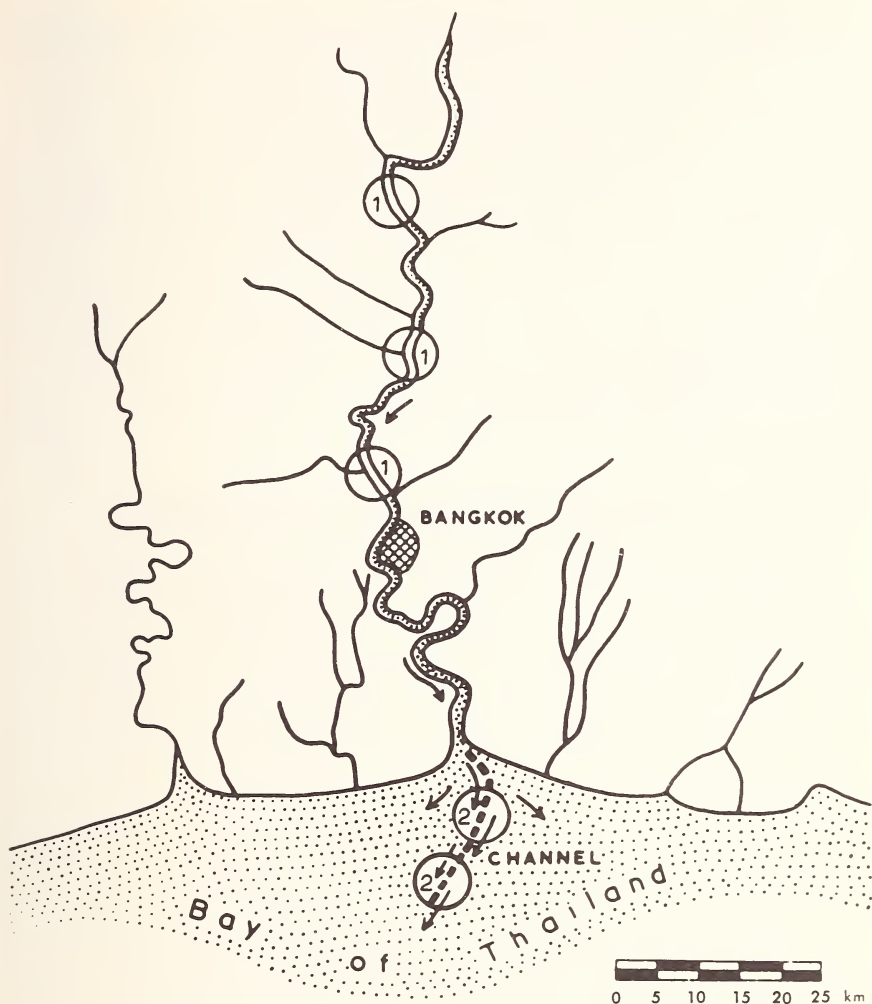
Figure 6. Chao Phya delta (Thailand), movement of sediments.
