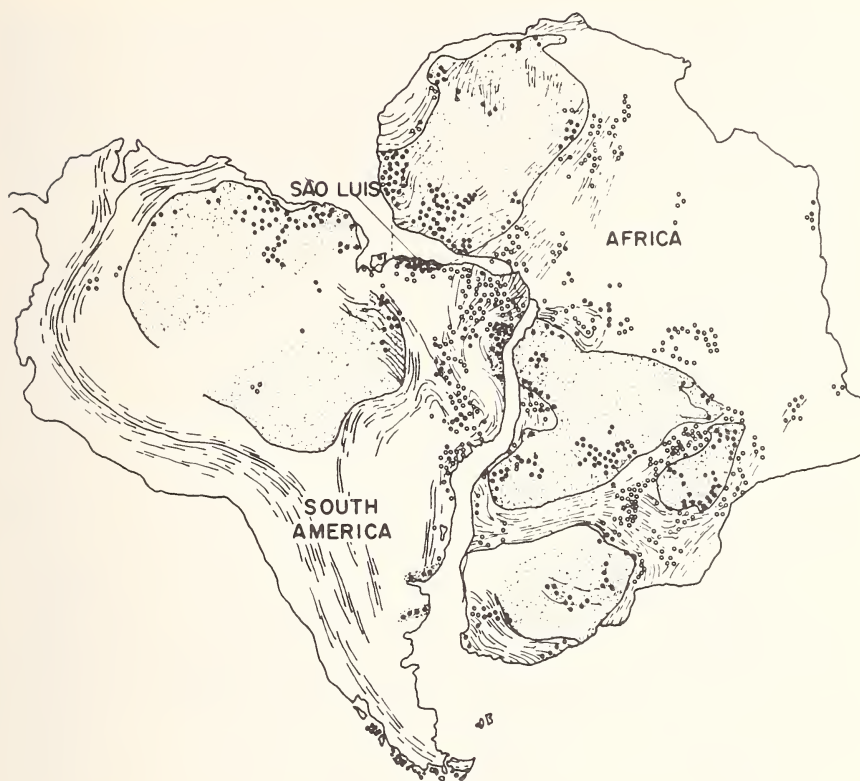
Figure 2. Matching geological age provinces of Africa and South America, by P. M. Hurley (1968).
