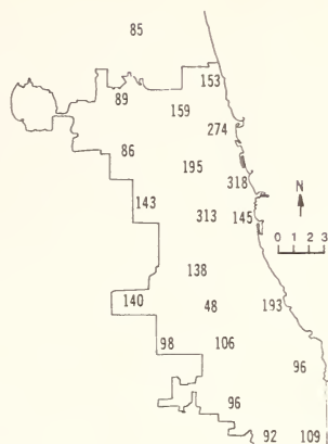
Figure 7. Distribution of aluminum 10^{-8} g/m 3 .
