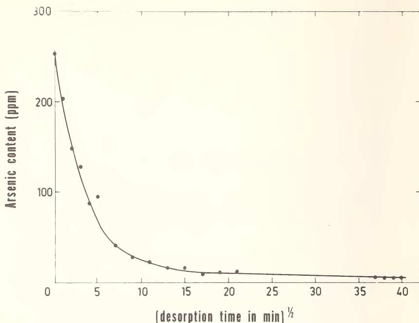
Figure 4. Desorption curve for hair type A after impregnation with a 300 ppm \text{As}^{\text{V}} solution at pH 4.35.
