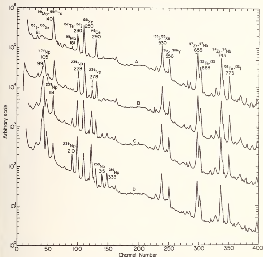
Figure 2. Gamma-ray spectra of NBS Standard Reference Materials with increasing ^{235}\text{U} content. A=5 mg \text{U}_3\text{O}_8 93.27% ^{235}\text{U} 1 min irradiated 24 h AEB 40 min count; B=20 mg \text{U}_3\text{O}_8 10.007% ^{235}\text{U} 5 min irradiated 24 h AEB 40 min count; C=20 mg \text{U}_3\text{O}_8 2.10% ^{235}\text{U} 5 min irradiated 24 h AEB 40 min count; D=20 mg \text{U}_3\text{O}_8 0.72% ^{235}\text{U} 5 min irradiated 24 h AEB 40 min count.
