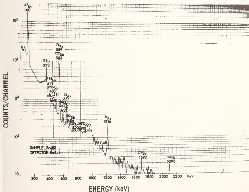
Figure 1. Alloy sample Ge(Li) spectrum.
