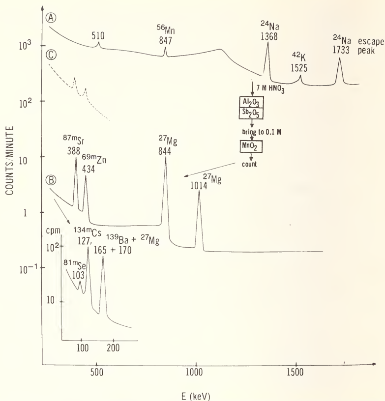
Figure 12. Example of chemical spectrum stripping applied to short-lived radioelements (The dotted spectrum C would be obtained in absence of the Al 2 O 3 column). A. Gamma-ray spectrum of the irradiated sample. B. Gamma-ray spectrum of the effluent after the chemical separation indicated in the figure. C. Gamma-ray spectrum of the effluent omitting the Al 2 O 3 .
