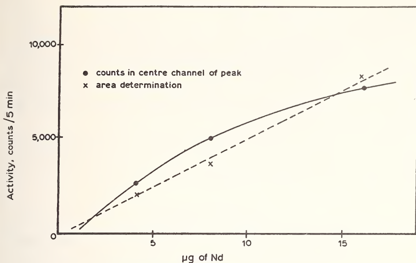
Figure 2. Standard calibration curve for neodymium analysis.
