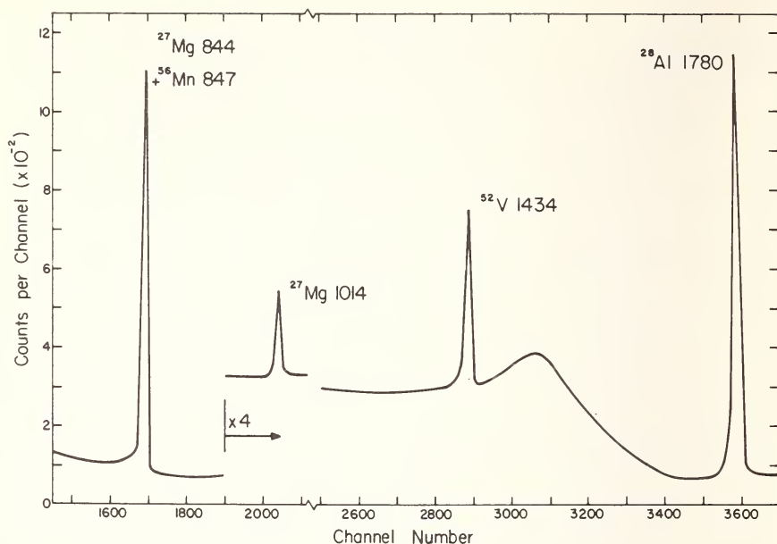
Figure 1. Gamma-ray spectrum of neutron activated meteorite sample observed with a 30 cm 3 Ge(Li) within a few minutes after irradiation. (Numbers attached to peaks are energies in keV.)
