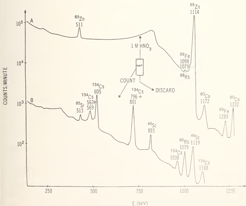
Figure 11. Example of chemical spectrum stripping applied to long-lived radioelements.
