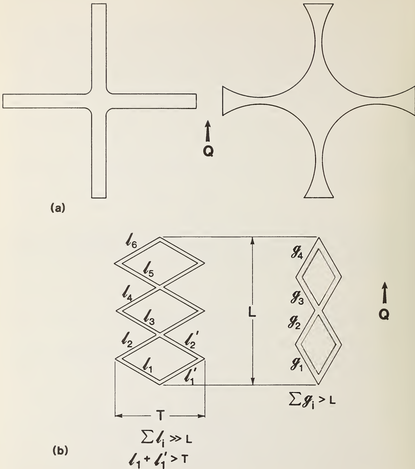
Figure 17. (a) Possible variations of resin distribution in two foams of equal density. (b) Possible heat-flow path lengths as a function of cell geometry for two foams of equal density and for different directions in a single foam.
