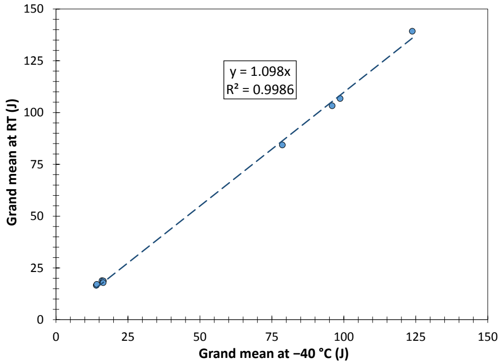
Figure 2 - Relationship between absorbed energy (grand means) at room temperature and -40\text{ }^{\circ}\text{C} .
