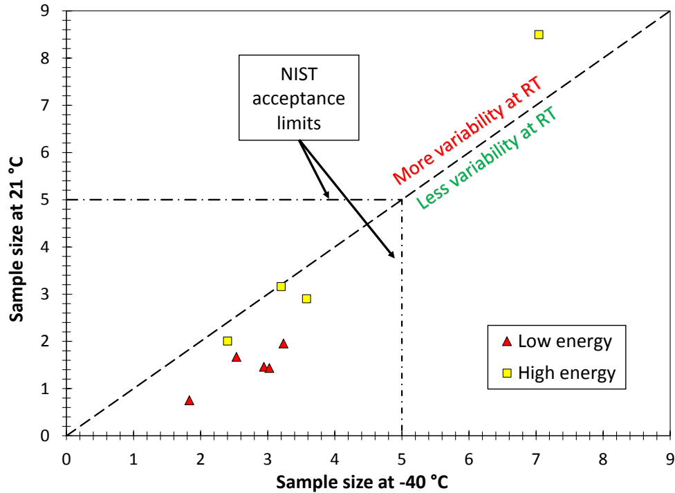
Figure 3 - Relationship between sample size at room temperature and -40\text{ }^{\circ}\text{C} .
