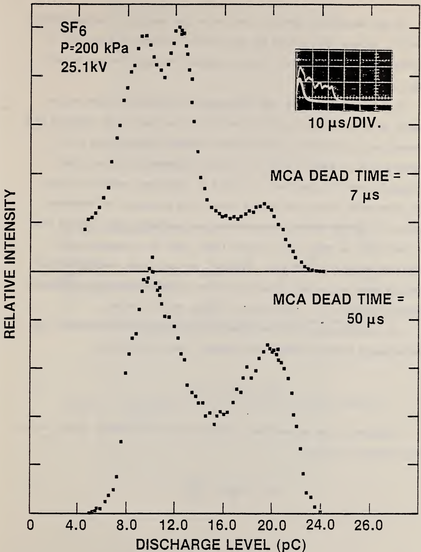
FIGURE 4. Measured partial discharge pulse height distributions in \text{SF}_6 for different multichannel analyzer dead times. Also shown in the inset is an oscilloscope trace displaying pulses from three separate partial discharge events, one of which corresponds to a burst.
