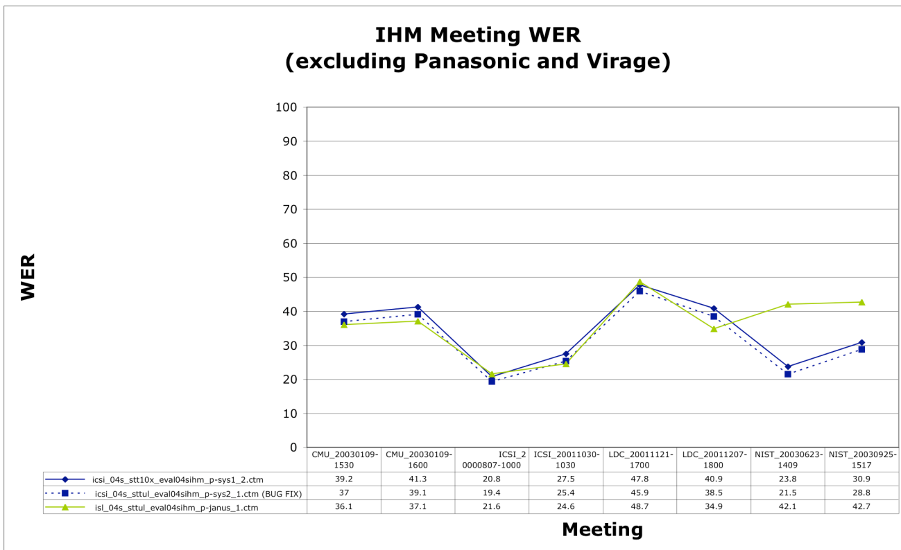
Figure 23 - IHM Meeting WER (excluding Panasonic and Virage)
