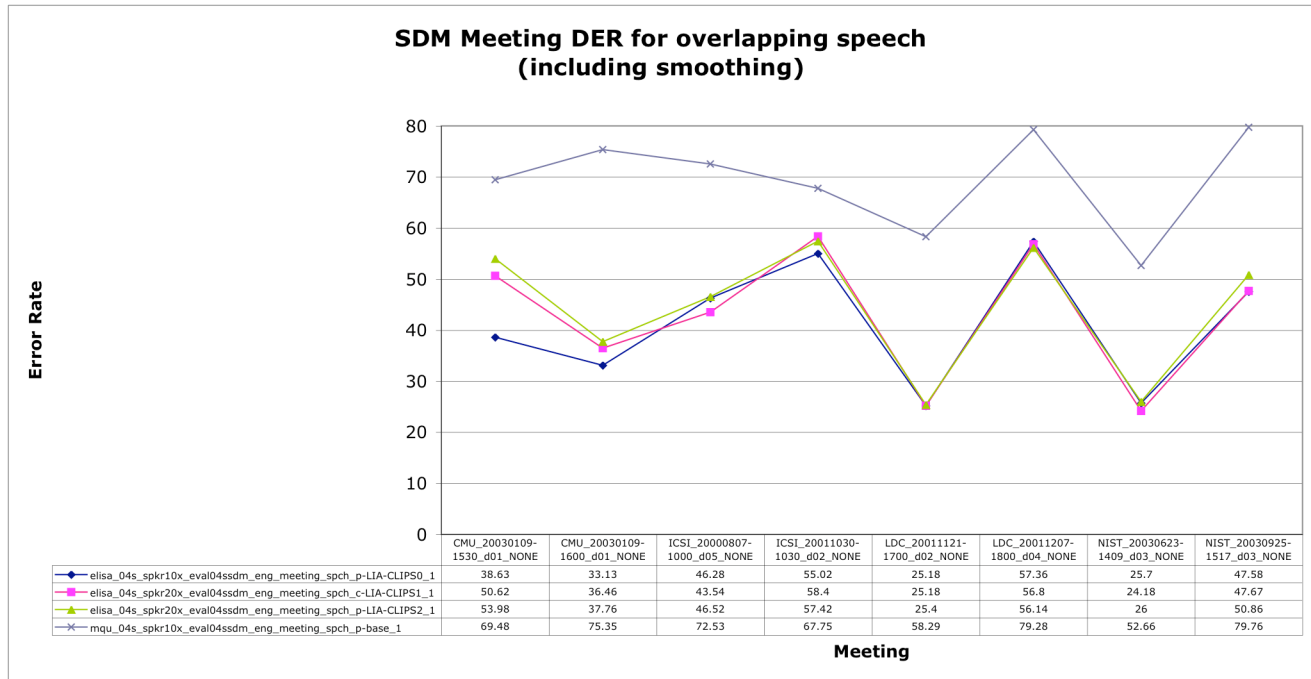
Figure 12 - SDM Meeting DER for overlapping speech (including smoothing)
