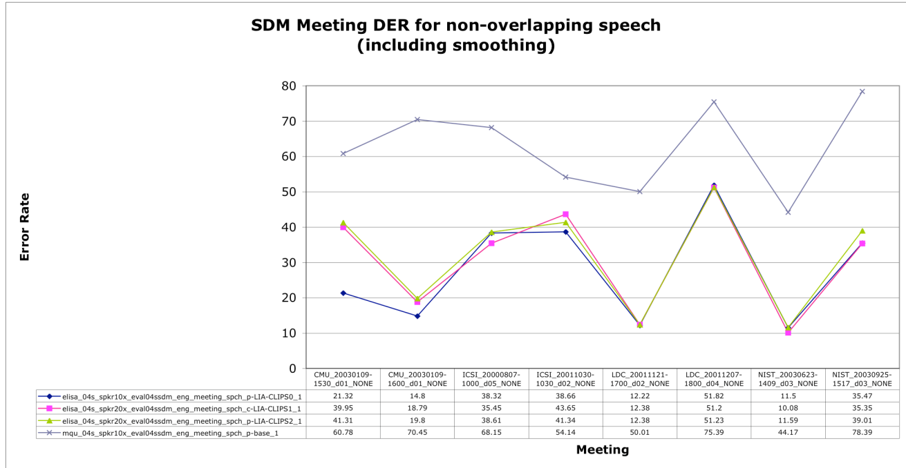
Figure 11 - SDM Meeting DER for non-overlapping speech (including smoothing)
