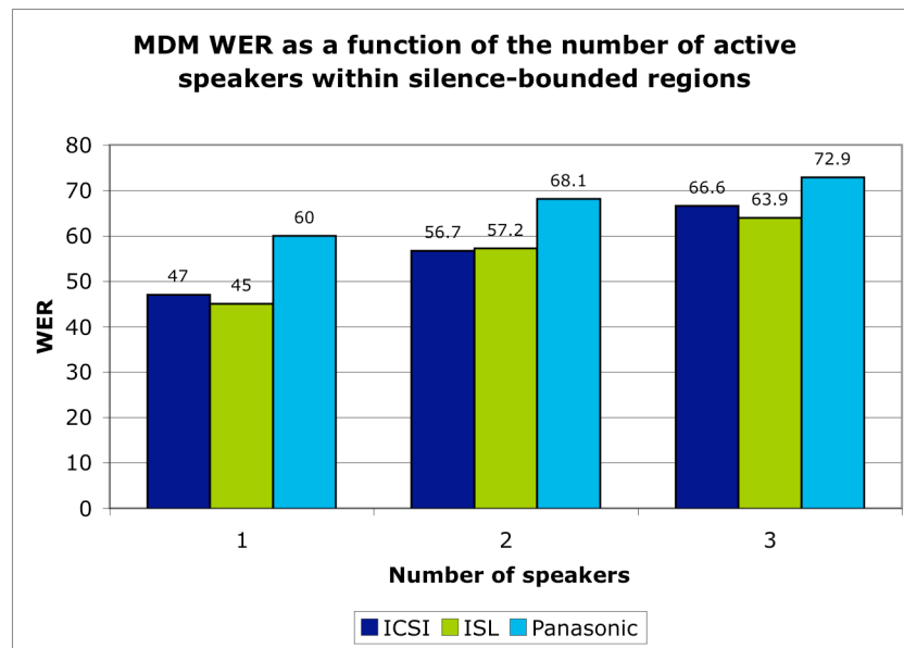
Figure 30 – WER as a function of the number of active speakers within silence-bounded regions
