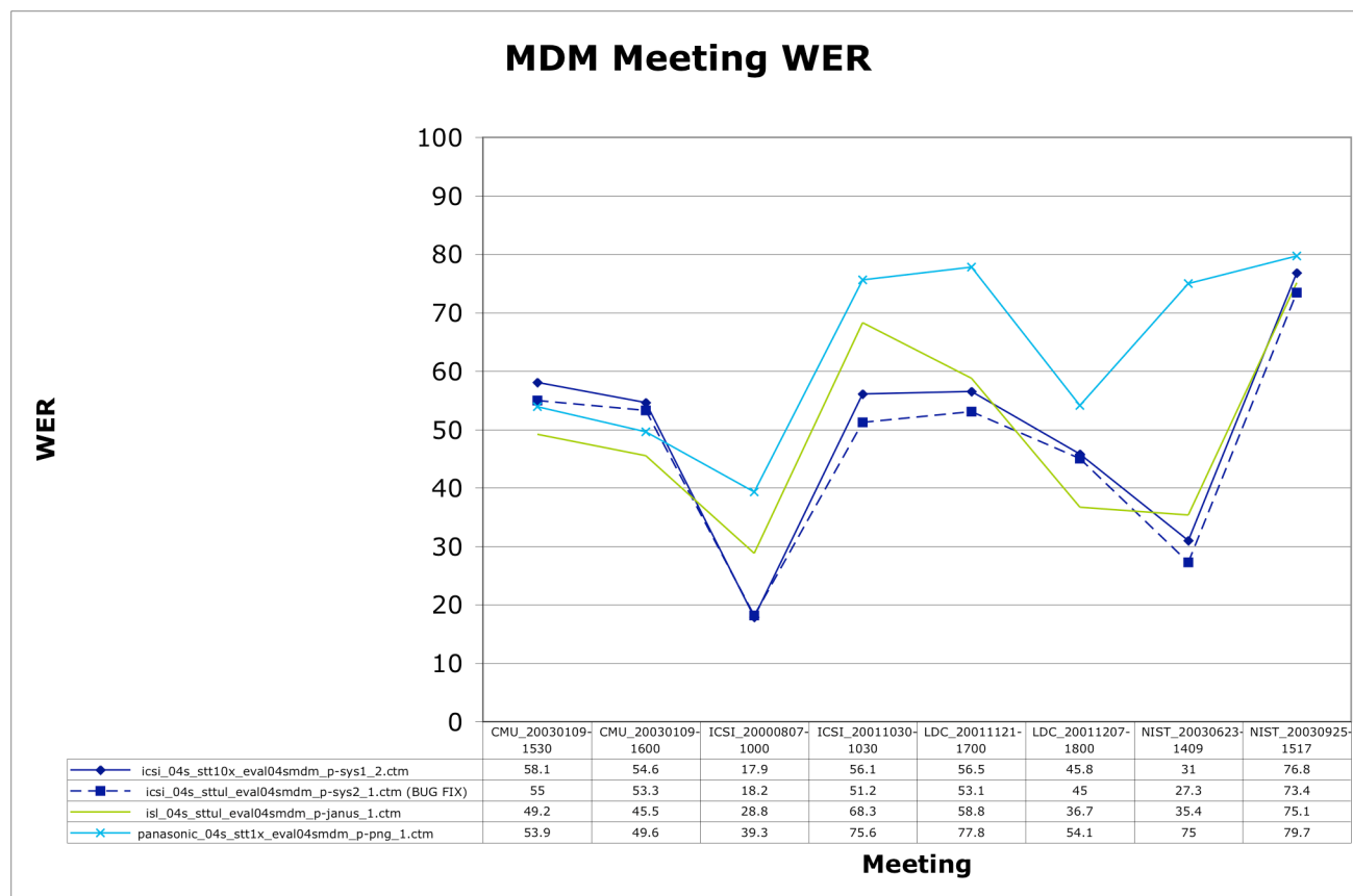
Figure 16 - MDM Meeting WER
