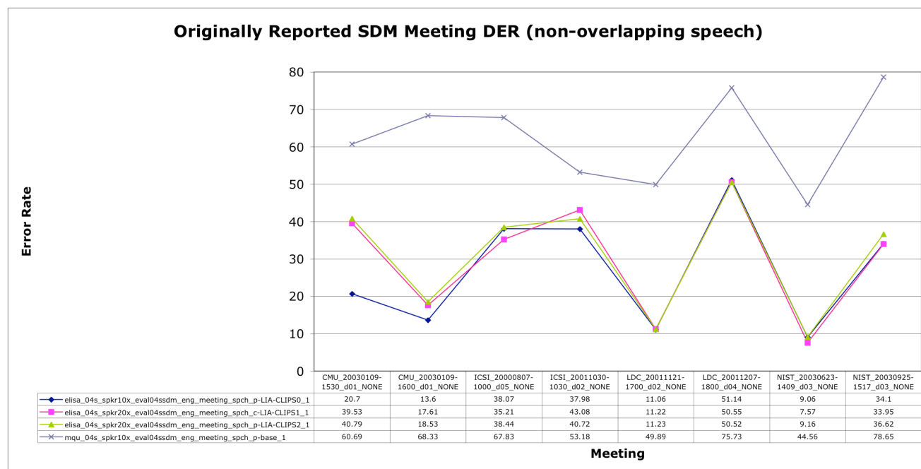
Figure 8 - SDM Meeting DER (non-overlapping speech)
