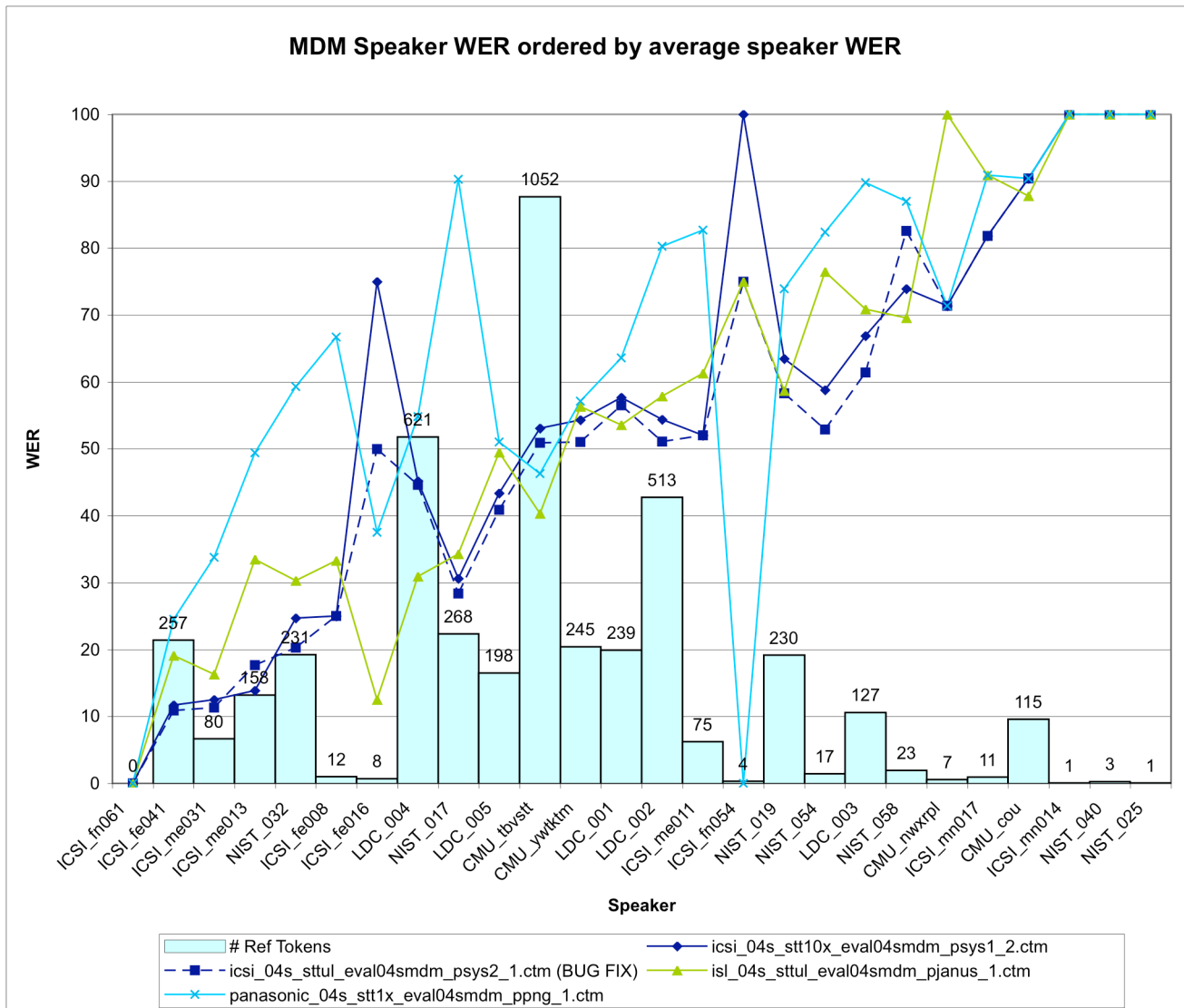
Figure 17 - MDM Speaker WER ordered by average speaker WER
