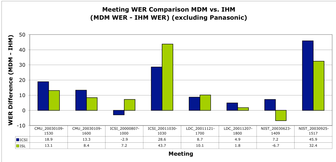
Figure 28 – Meeting WER Comparison MDM vs. IHM (excluding Panasonic)
