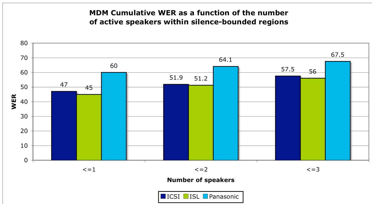
Figure 31 - Cumulative WER as a function of the number of active speakers within silence-bounded regions
