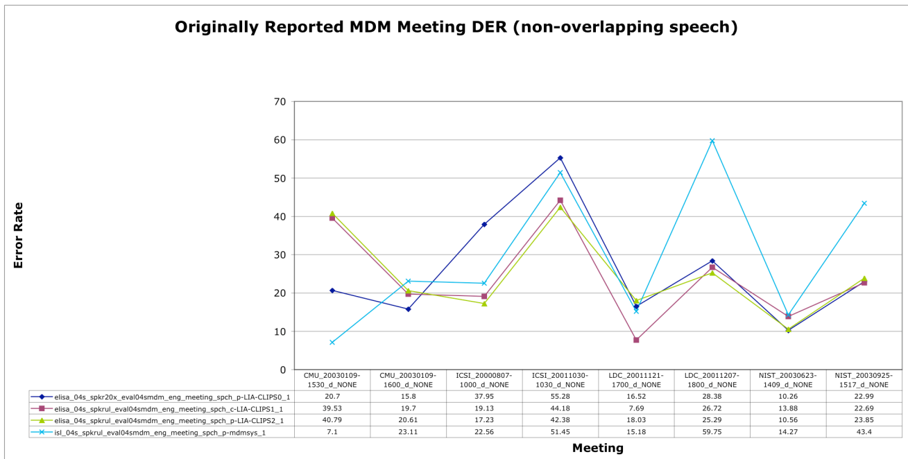
Figure 2 - MDM Meeting DER (non-overlapping speech)
