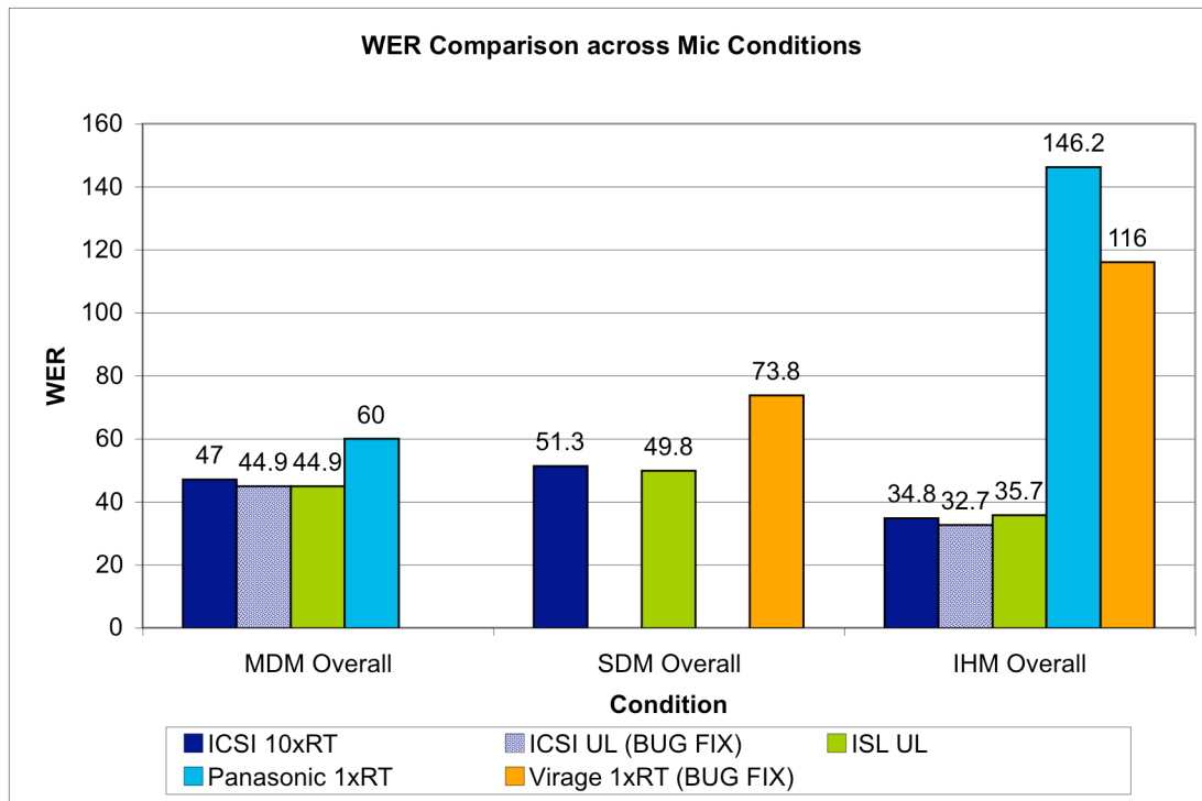
Figure 25 - WER Comparison across Mic Conditions
