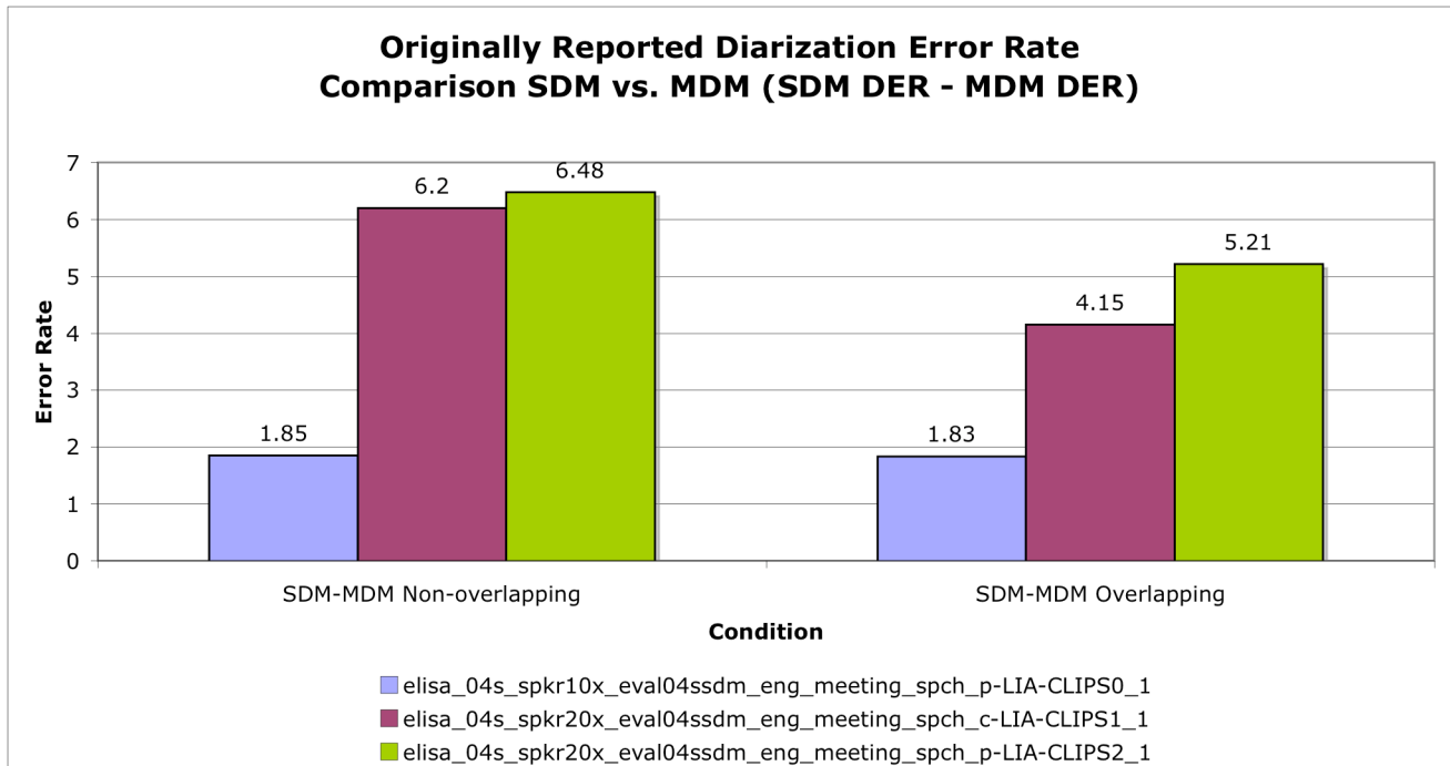
Figure 13 – Originally Reported Diarization Error Rate Comparison SDM vs. MDM
