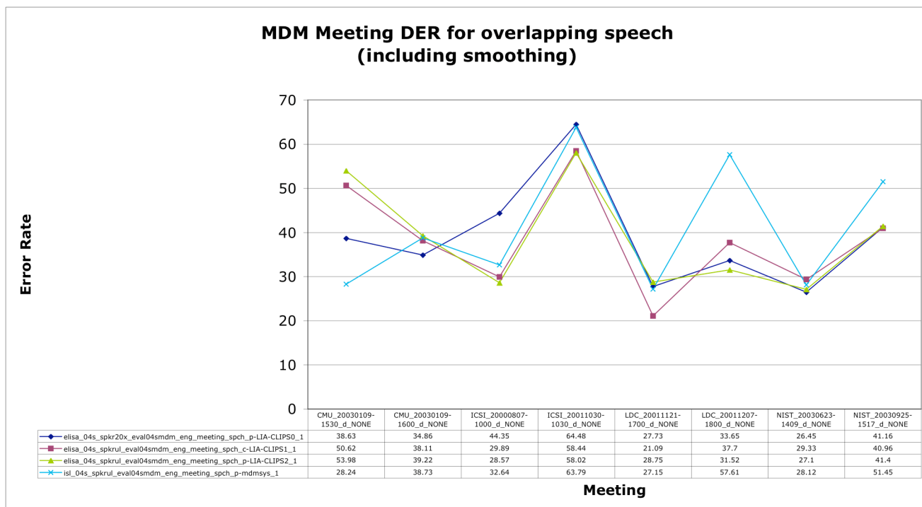
Figure 6 - MDM Meeting DER for overlapping speech (taking smoothing into account)
