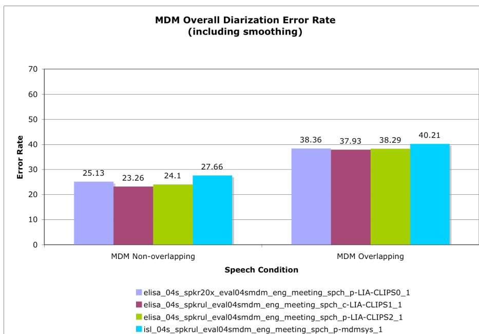
Figure 4 - MDM Overall Diarization Error Rates (including smoothing)
