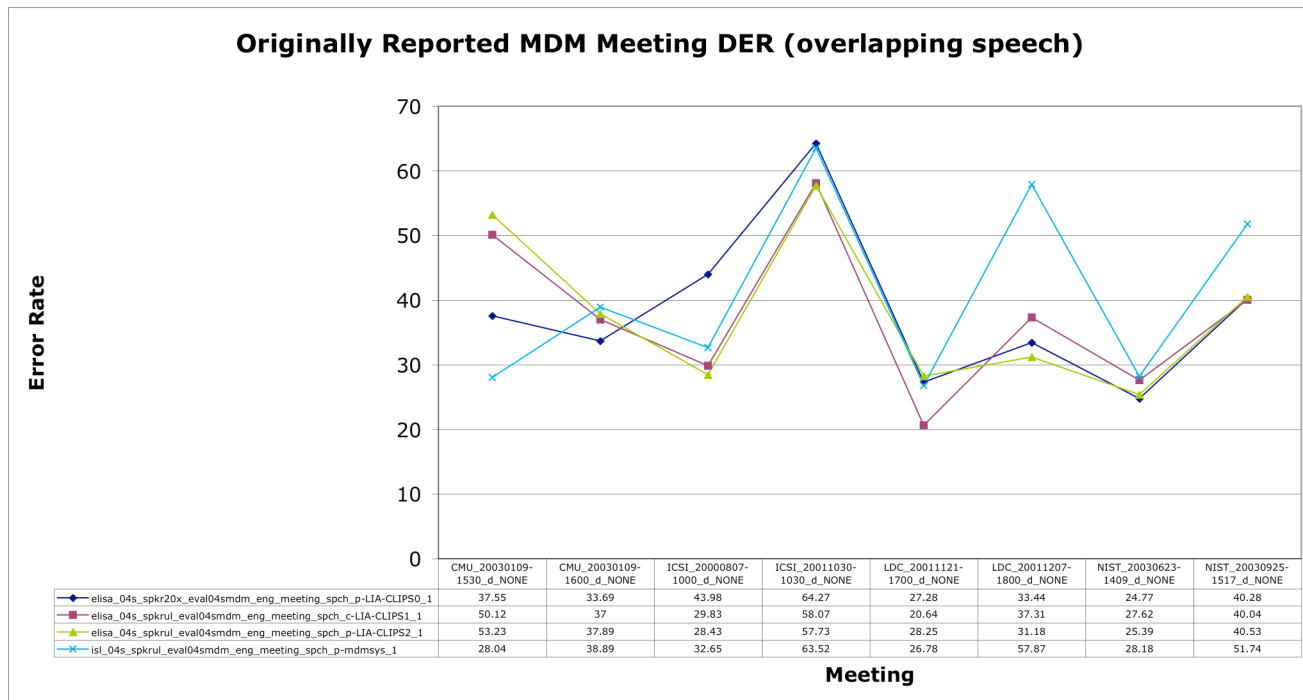
Figure 3 - MDM Meeting DER (overlapping speech)
