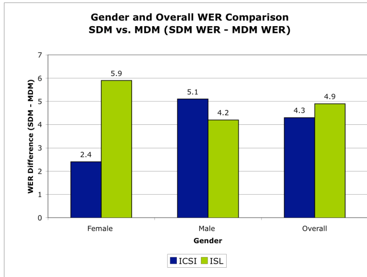
Figure 26 –Gender and Overall WER Comparison SDM vs. MDM
