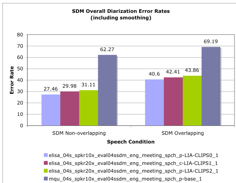
Figure 10 - SDM Overall Diarization Error Rates (including smoothing)
