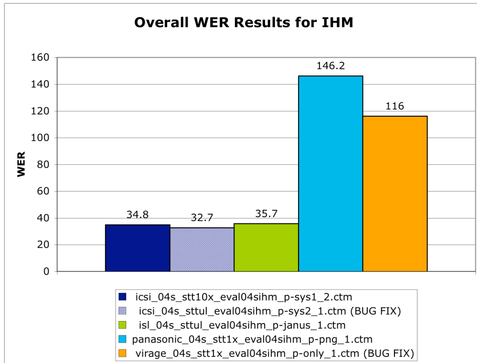
Figure 21 - Overall WER Results for IHM
