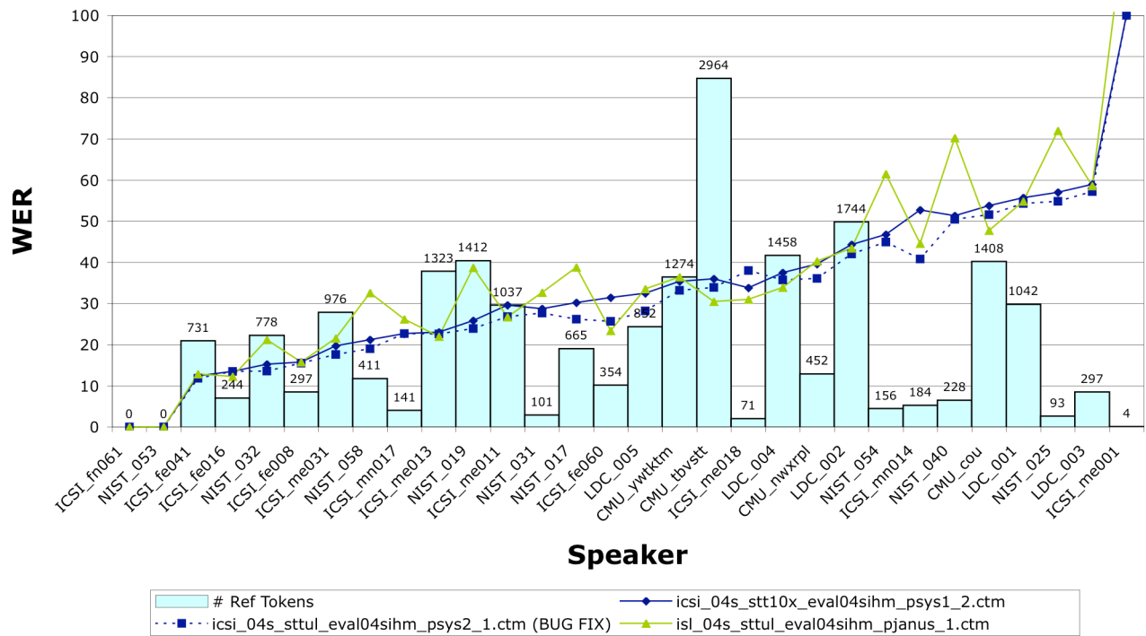
Figure 24 - IHM Speaker WER (excluding Panasonic and Virage)
