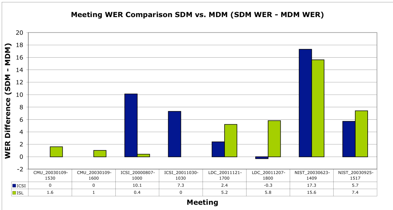
Figure 27 – Meeting WER Comparison SDM vs. MDM
