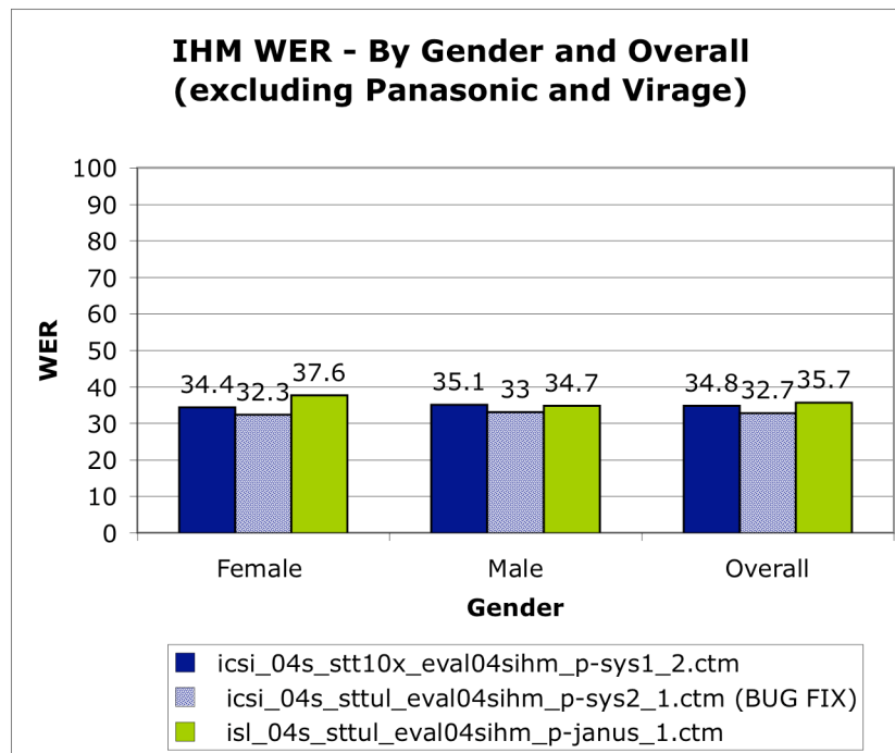
Figure 22 - IHM WER - By Gender and Overall (excluding Panasonic and Virage)
