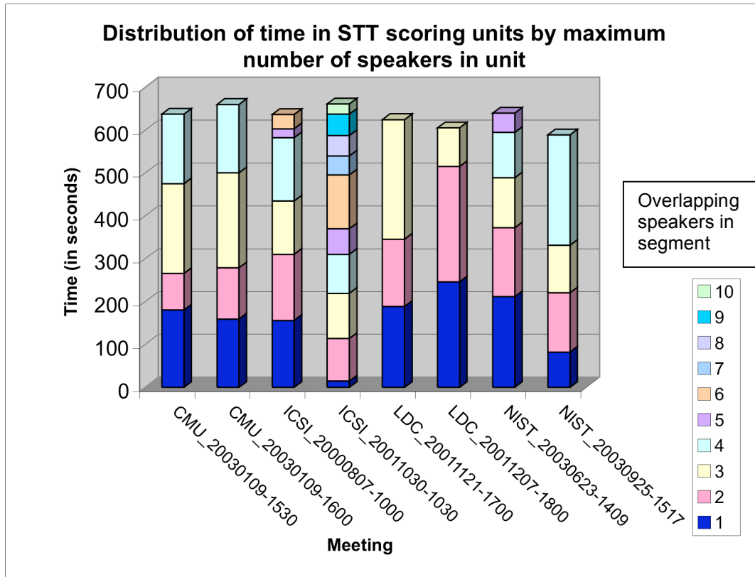
Figure 29 - Distribution of time in STT scoring units by maximum number of speakers in unit
