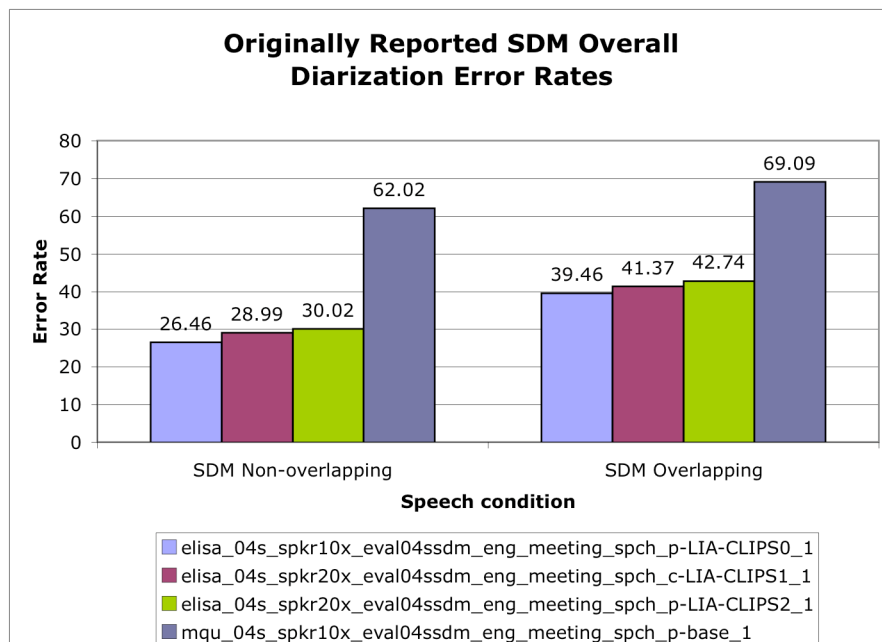
Figure 7 - SDM Overall Diarization Error Rates
