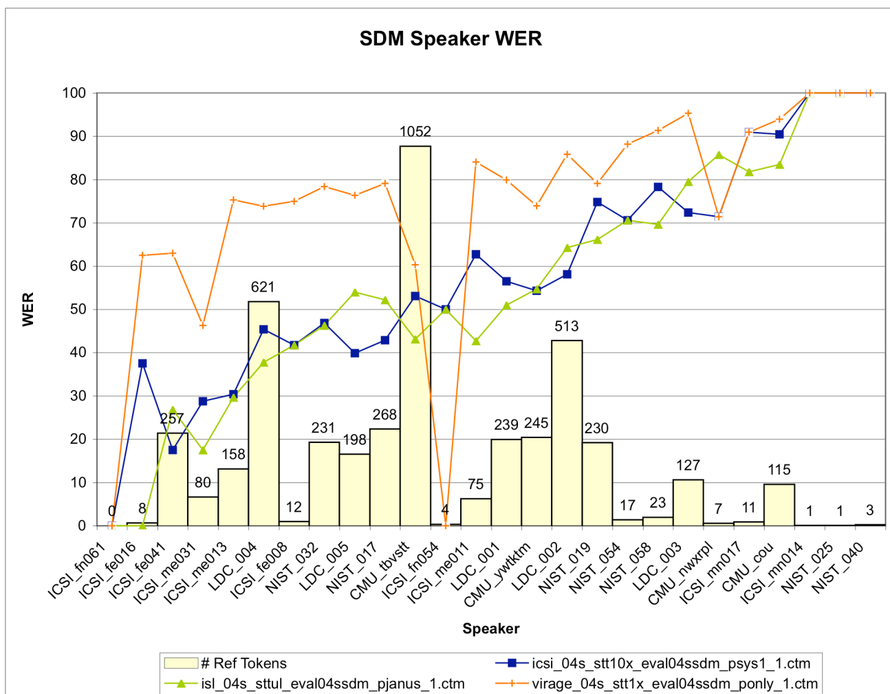
Figure 20 - SDM Speaker WER
