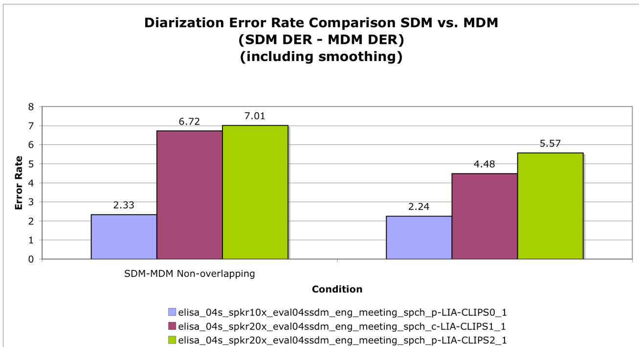
Figure 14 - Diariation Error Rate Comparison SDM vs. MDM (including smoothing)
