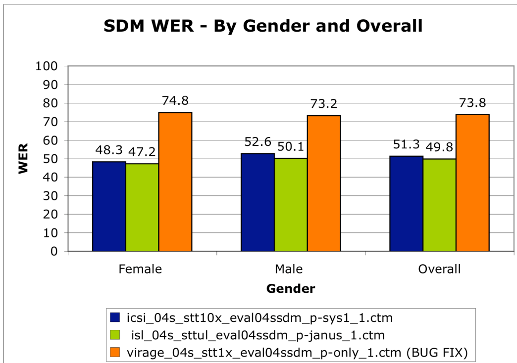
Figure 18 - SDM WER - By Gender and Overall
