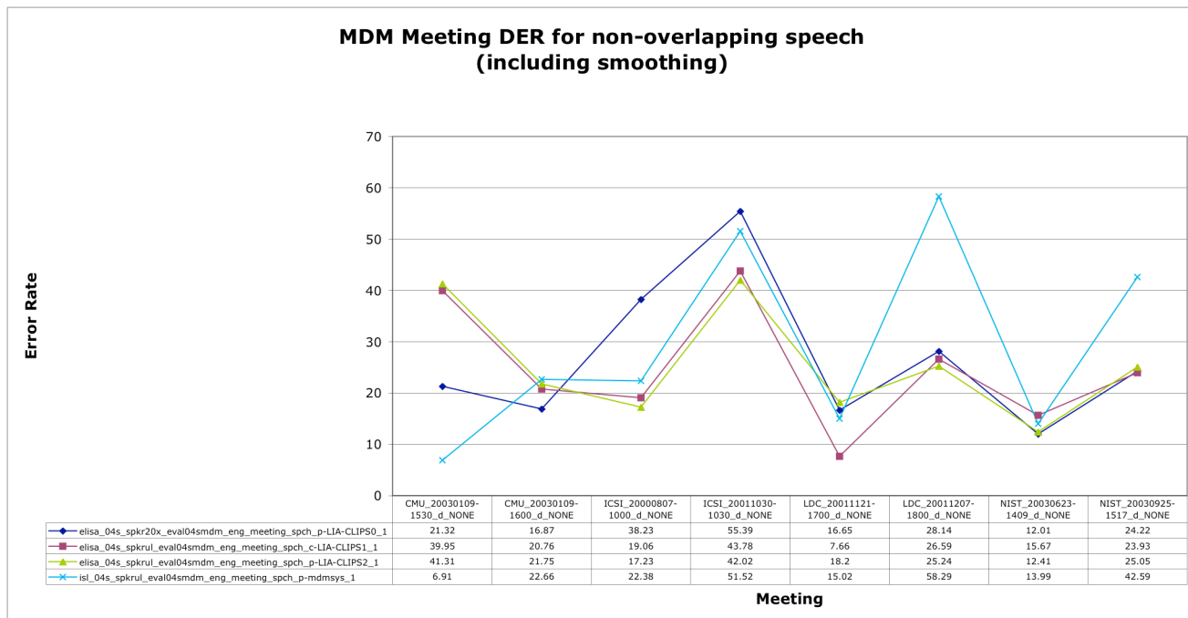
Figure 5 - MDM Meeting DER for non-overlapping speech (taking smoothing into account)
