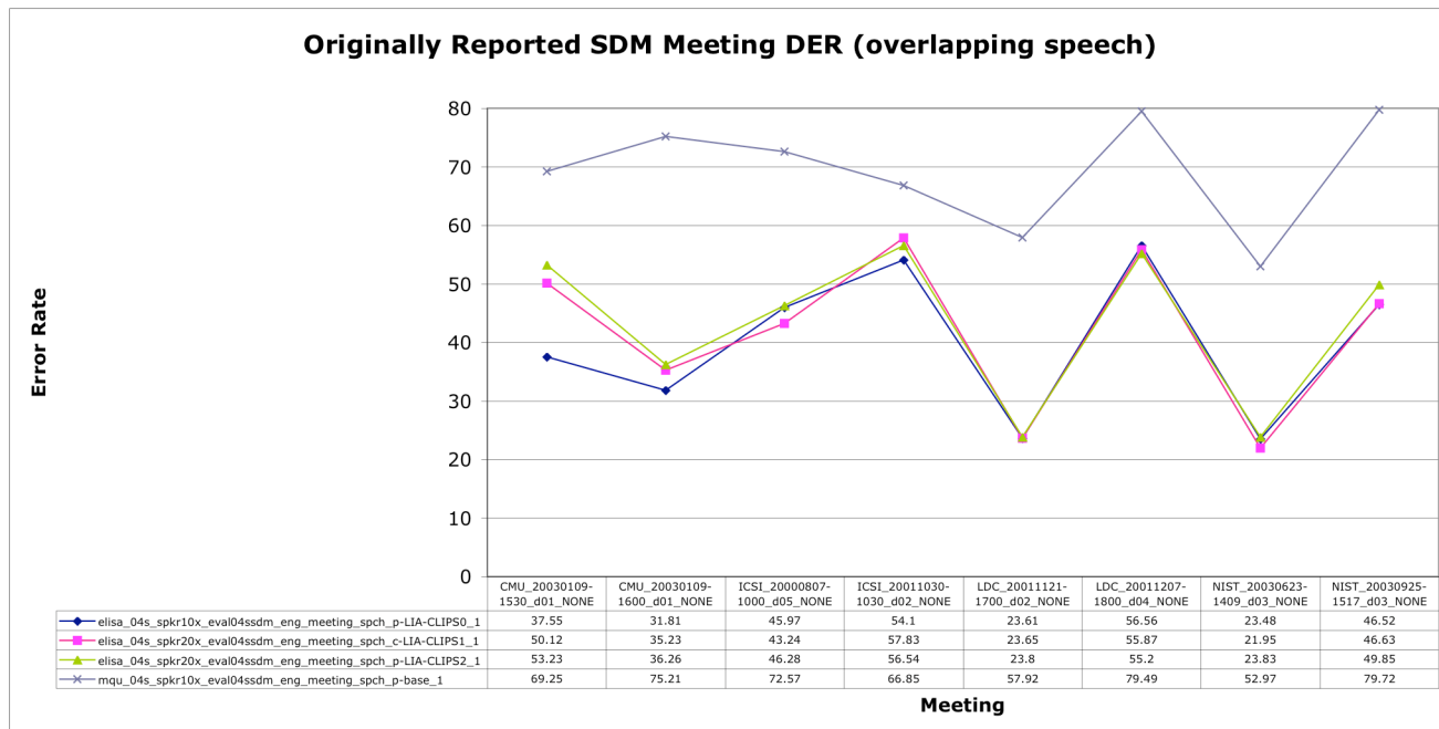
Figure 9 - SDM Meeting DER (overlapping speech)
