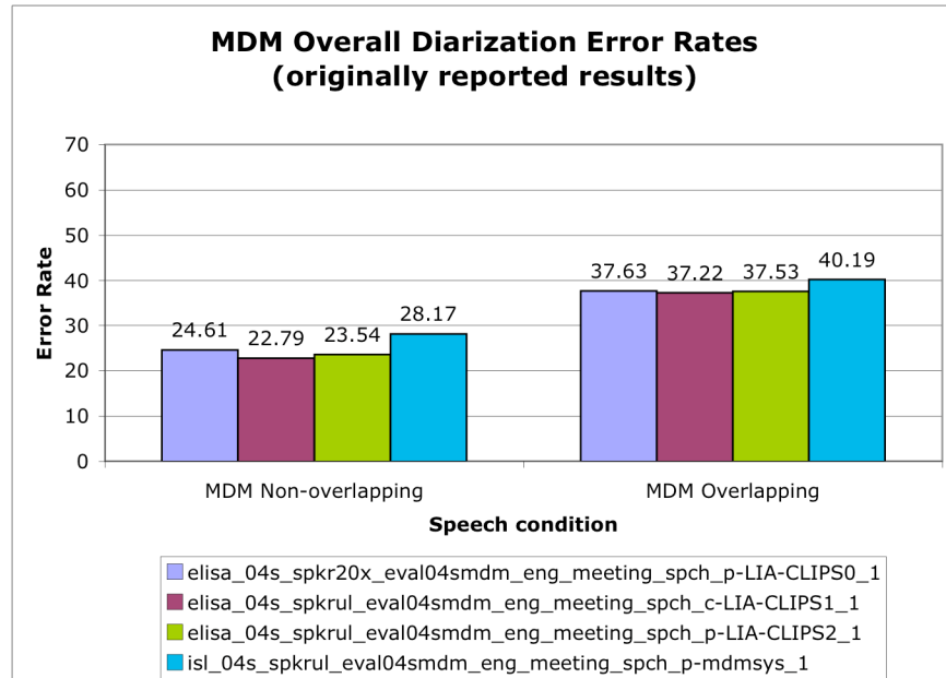
Figure 1 - MDM Overall Diarization Error Rates
