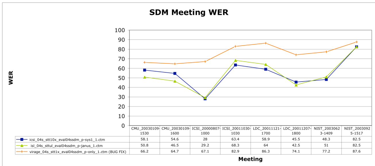
Figure 19 - SDM Meeting WER
