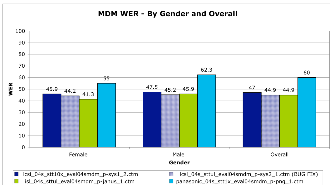
Figure 15 - MDM WER – By Gender and Overall
