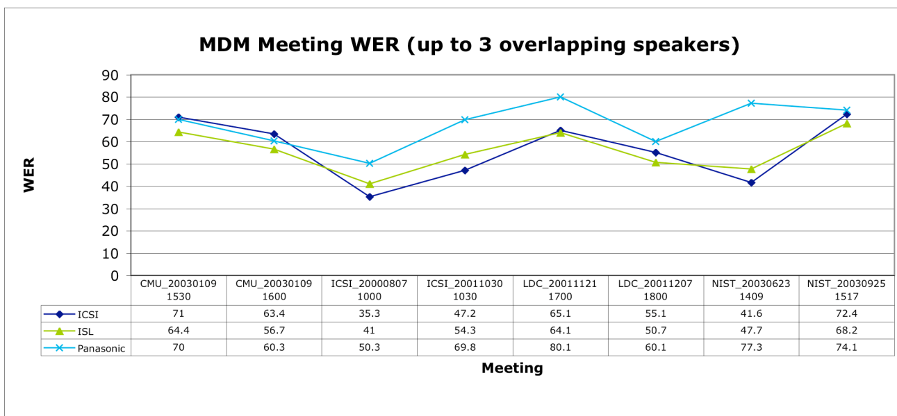
Figure 32 - Meeting WER (up to 3 overlapping speakers)
