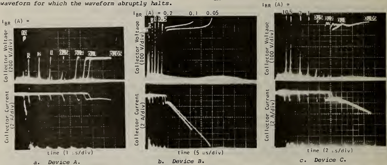
Figure 3. The collector voltage and current waveform for the same devices as in figure 2. RBSB occurs when the voltage waveform appears to halt and discontinuously goes to zero.
