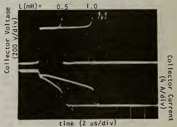
Figure 5. The collector voltage and current waveform for I_{CM} = 10 A, I_{BR} = 0.1 A, and L = 0.5 mH and 1.0 mH.
