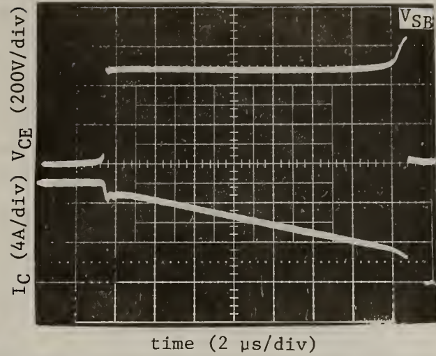
Figure 3. Collector voltage and current waveforms for a device which reaches V_{CEX}(SUS) prior to RBSB. The occurrence of RBSB is noted on the voltage waveform.
