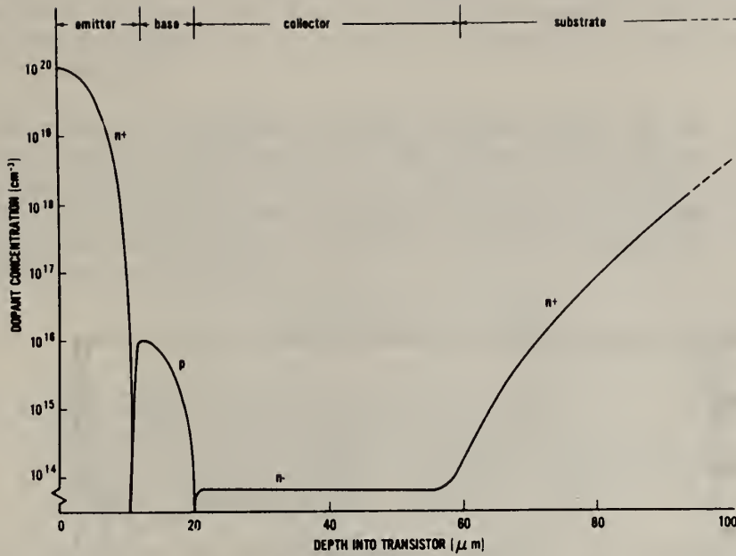
Figure 1. Typical dopant profile as determined from spreading resistance of a high-voltage n^+p-n^-n^+ power transistor.
