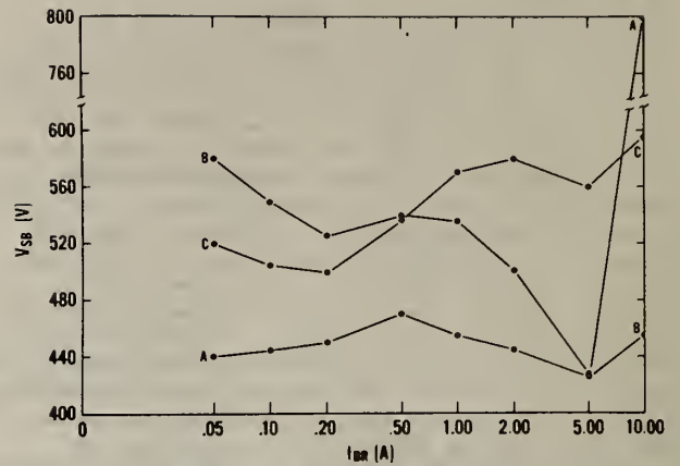
Figure 2. The measured voltage at which RBSB occurred, V_{SB} , for a collector current of 10 A for various values of reverse-base current, I_{BR} , for three devices, A, B, and C.
