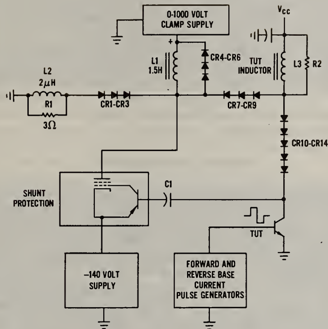
Figure B-1. Simplified diagram for a circuit used to test transistors for reverse-bias second breakdown.
