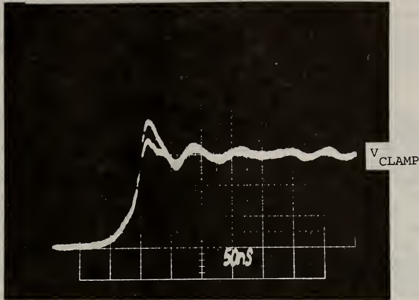
Figure B-2. Examples of voltage overshoot using solid-state diode and vacuum tube diode. The overshoot is 100 V for solid-state diode and 50 V for the tube diode. The vertical scale is 100 V per division and the horizontal scale is 50 ns per division.
