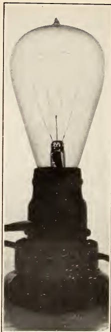
FIG. 31.— Standard of total radiation (Radiant energy)
