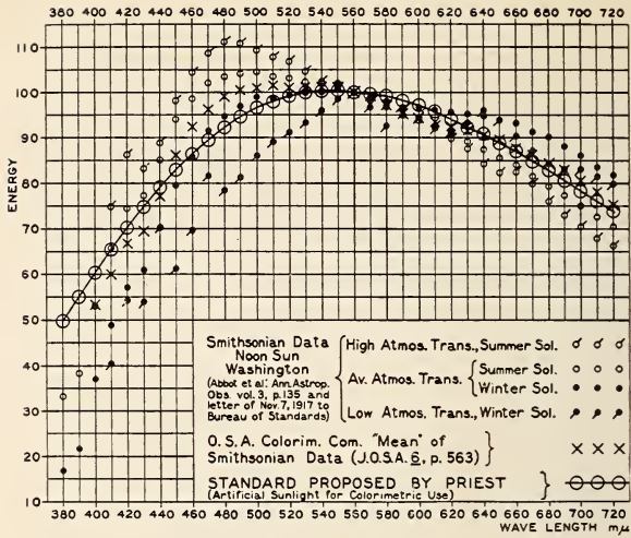
FIG. 4.— Standard of color (Standard sunlight)
