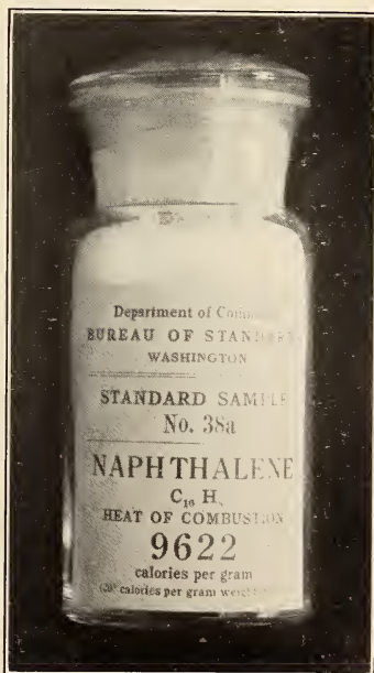
FIG. 3.—Standard for heat of combustion
