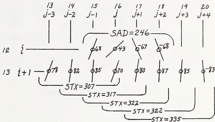
Figure 4. Locating Core Area
