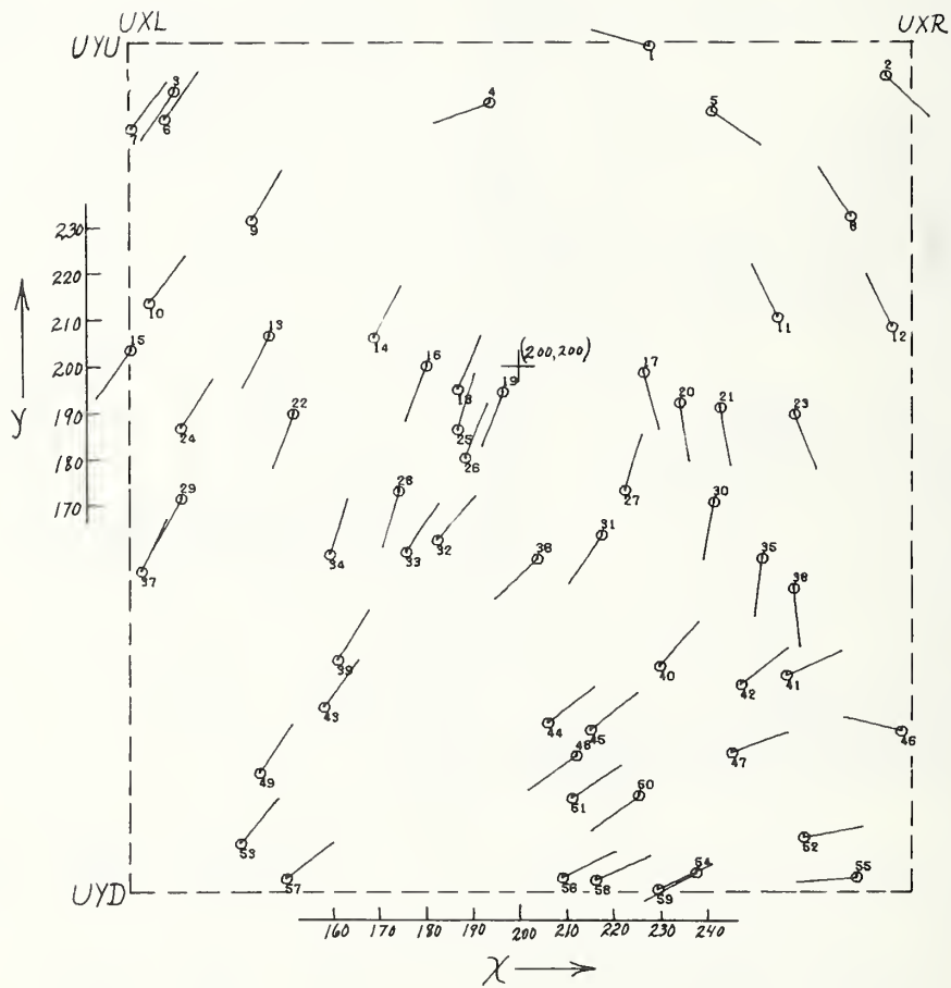
Figure 20. Minutia Data Ready for File or Search
