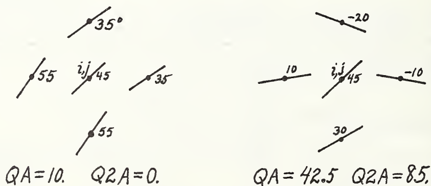
Figure 18. Ridge Quality Measures Around (i,j)
