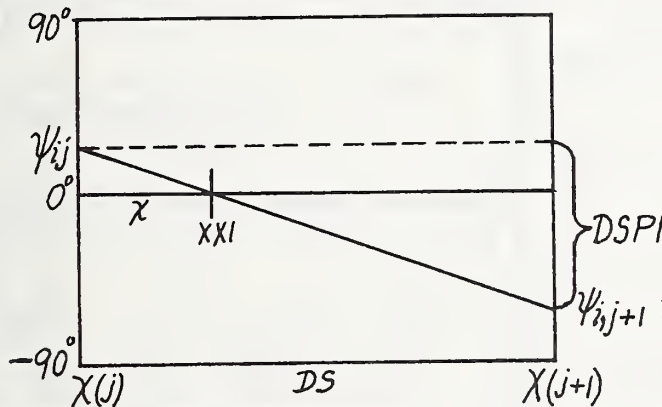
Figure 10. Computation of XXI for Loops, Whorls, and Arches
