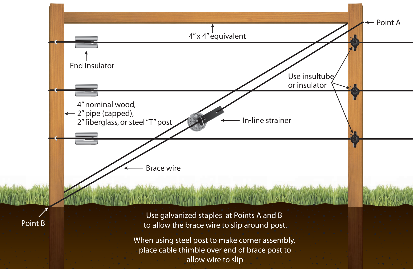
Drawing 8c "H" Brace
