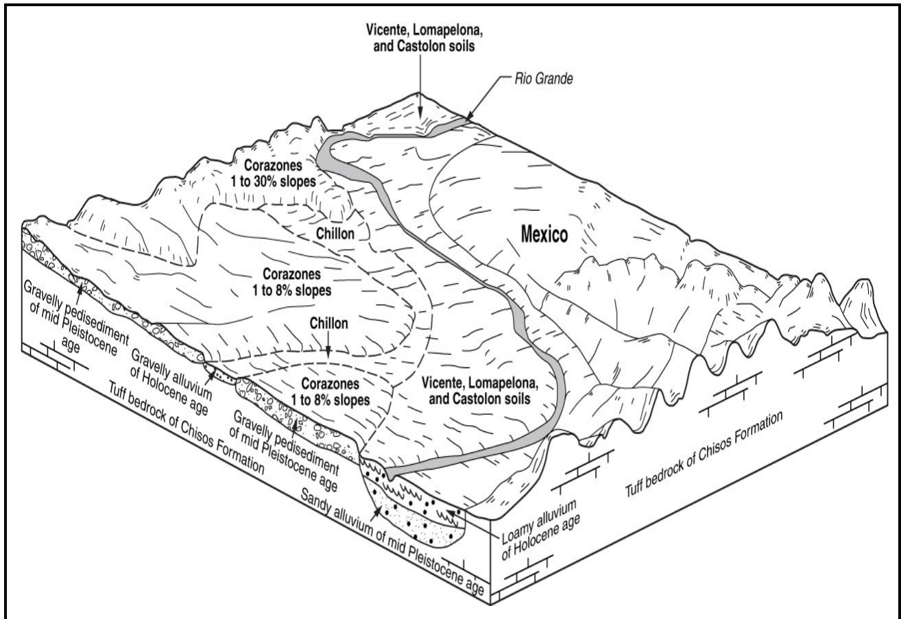
Figure 75.—Relationship of detailed soil map units and Holocene age sediments.
