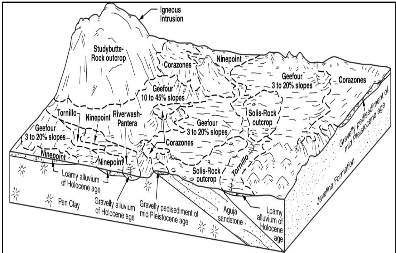
Figure 79.—Relationship of soil mapping units, geologic formations, and landscape positions of the Pen Clay, Aguja sandstone, loamy alluvium, and Javelina Formations.
