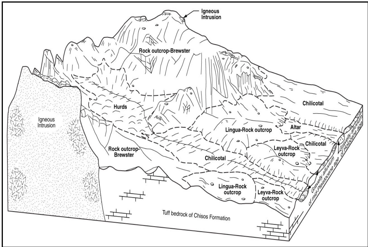
Figure 80.—Relationship of soil mapping units, geologic formations, and landscapes of the Chisos Formation, igneous intrusions, and gravelly alluvium of both mid-Pleistocene and Holocene ages.
