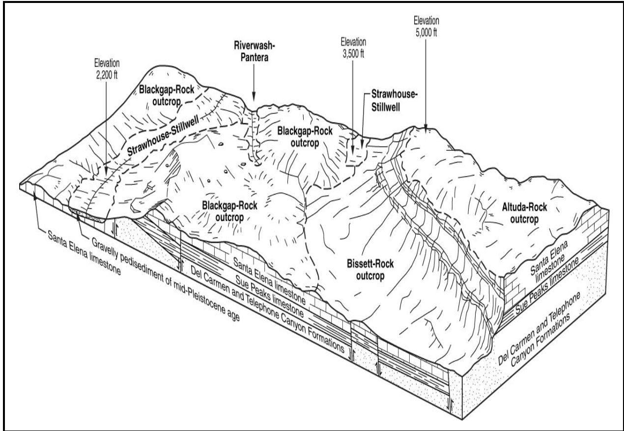
Figure 77.—Relationship of soil mapping units to elevation, geology, and landscape positions. Altuda soils are at elevations around 5,000 feet, and formed from the Santa Elena limestone. Blackgap and Bissett soils formed in residuum and colluvium.
