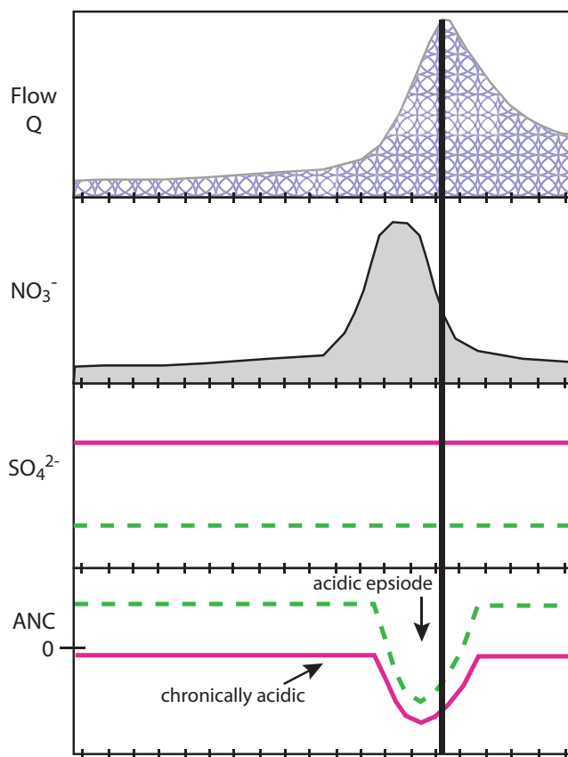
Figure 18.2—Conceptual diagram of changes in surface water chemistry of two contrasting upland streams impacted by atmospheric deposition in response to a hydrologic event. The upper two panels are discharge ( Q ) and nitrate ( \text{NO}_3^- ) during the stream event; the pattern is identical for both streams. The two streams have two different concentrations of \text{SO}_4^{2-} in the third panel; the solid line represents a stream with high \text{SO}_4^{2-} and the dashed line is a stream with low \text{SO}_4^{2-} . The fourth panel is acid neutralizing capacity (ANC). The stream with the higher \text{SO}_4^{2-} (solid line) has a lower ANC during baseflow, and is chronically acidic. During the episodic event, ANC values decrease somewhat from low baseflow values, due to the pulsed input of \text{NO}_3^- . The low \text{SO}_4^{2-} stream (dashed line) has low, but positive ANC during baseflow. At this site the pulse of \text{NO}_3^- during the event causes a short-term decrease in ANC to acidic conditions ( \text{ANC} < 0 \mu\text{eq/L} ).
