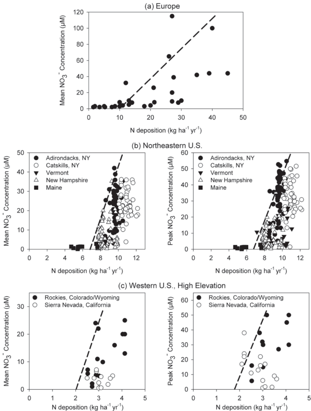
Figure 18.3—Relationship between mean and peak annual nitrate concentration ( \mu\text{M} ) and nitrogen deposition ( \text{kg N ha}^{-1} \text{ yr}^{-1} ) in (a) forested catchments in Europe; (b) forested catchments in the northeastern United States; and (c) high elevation catchments in the western United States. European data from (Wright et al. 2001). Northeastern United States data are from Aber et al. (2003). Western \text{NO}_3^- data are from Sickman et al. (2002) and Burns (2004). Western deposition was estimated from modeled \text{NO}_3^- deposition (Nanus et al. 2003) and \text{NH}_4^+ deposition from the nearest NADP station. Lines are drawn by eye to estimate the x- intercept, the value of N deposition at which significant \text{NO}_3^- leaching begins to occur.
