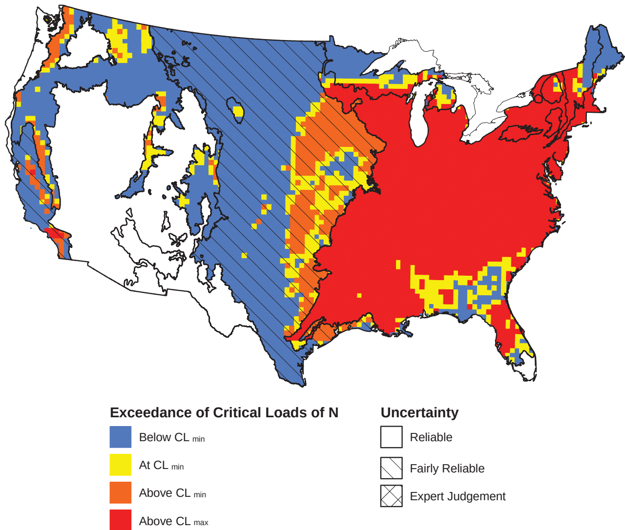
Figure 19.10—Map of exceedance of critical loads (CL) for \text{NO}_3^- leaching by ecoregion in the continental United States. Exceedance was calculated by subtracting critical loads from CMAQ nitrogen deposition. Exceedance (critical load - deposition) is shown for several categories: (1) No exceedance (Below CL), when deposition is lower than the CL range, (2) At CL, when deposition is within \pm 1 of the CL range, (3) Above CL min , when deposition is above the lower end of the CL range, but lower than the upper end of the range, (4) Above CL max , when deposition is above the upper end of the CL range. CMAQ deposition data were not available for Alaska, so we were not able to calculate exceedance for Alaska. White areas lack data for critical loads determination for nitrate leaching.
