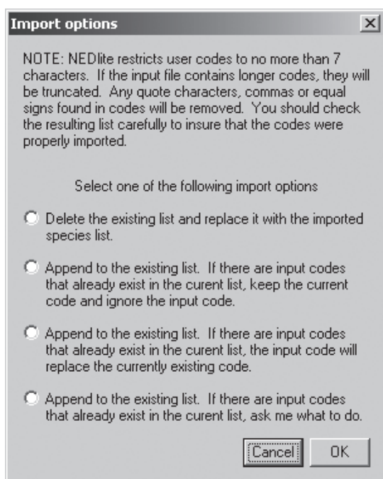
Figure 8.—Available options when importing species using the species codes program.
