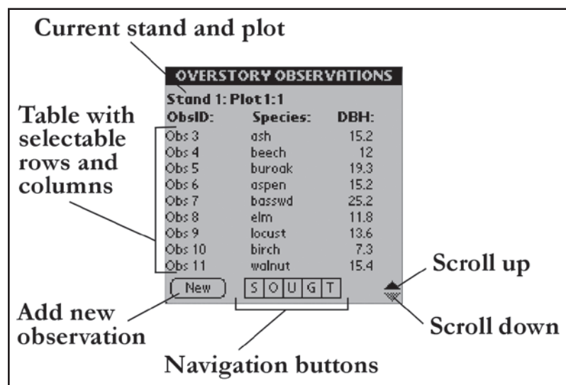
Figure 3.—Example table of overstory observations in NEDLite, with tools for navigating through data.
