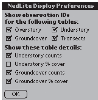
Figure 16.—Display preferences for observation tables in NEDLite.
