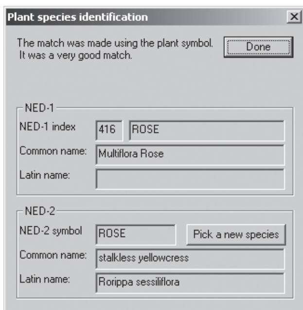
Figure 10.—Correcting the identity of a NED-1 species using the species codes program.
