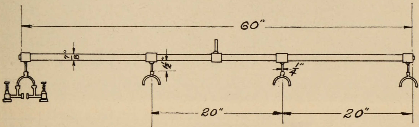
FIG. 18.—Four-row attachment for beet sprayer. (Original.)
