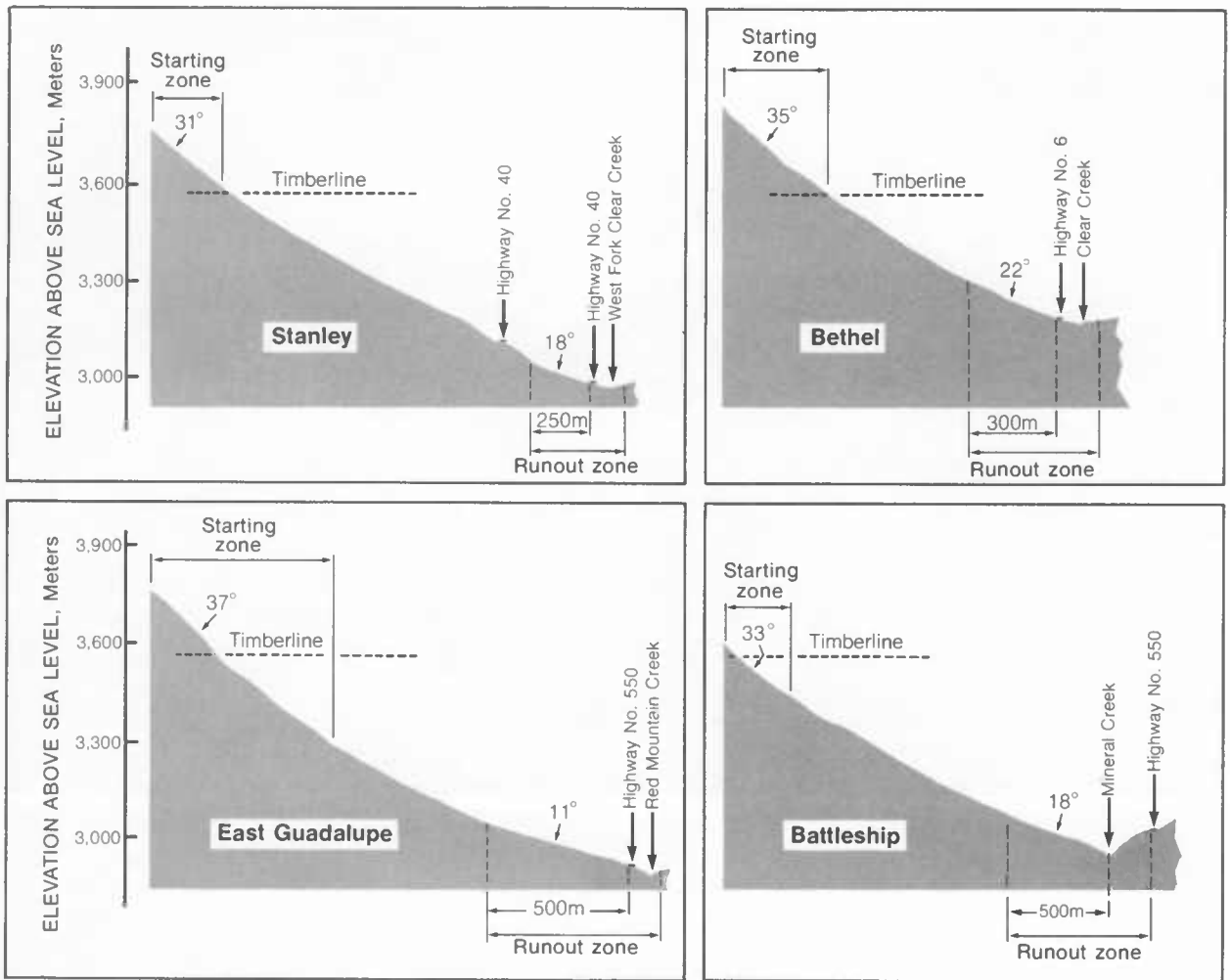
Figure 106.—Longitudinal profiles of four avalanche paths in Colorado.
