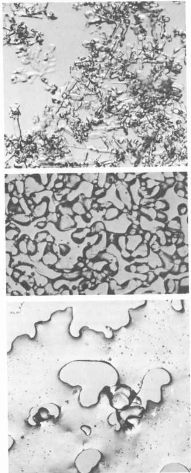
Figure 56.—Microscopic photographs of thin sections of snow and ice layers: Top, newly fallen snow a few hours old; middle, old, dense snow; and bottom, thin ice crust. Note the random arrangement of the ice skeleton and the general decrease in pore space with age.
