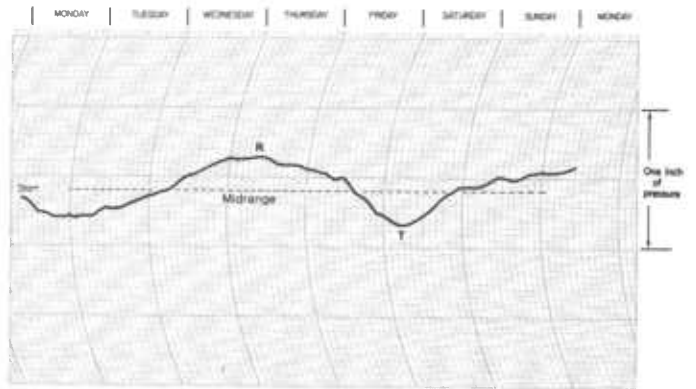
Figure 11.—Left, microbarograph and right, microbarograph chart from Berthoud Pass, Colo., for the week beginning December 13, 1973. Midrange position and trough and ridge periods are identified on the chart.
