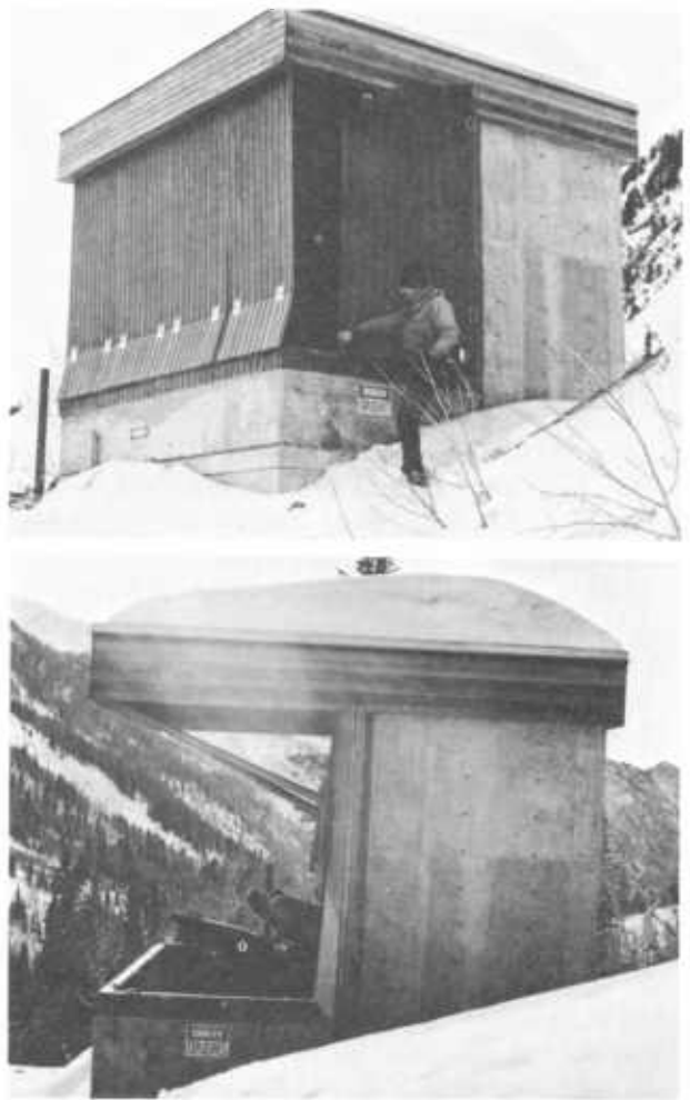
Figure 157.—Reinforced concrete enclosure used to protect a 75-mm howitzer at Snowbird, Utah. The howitzer pivots on a large steel plate.
