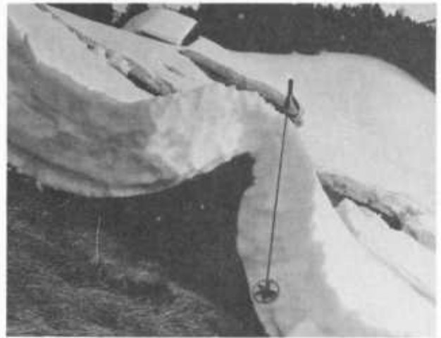
Figure 78.—Dramatic evidence of glide on a grass-covered mountain slope. (Photo by Frutiger)
