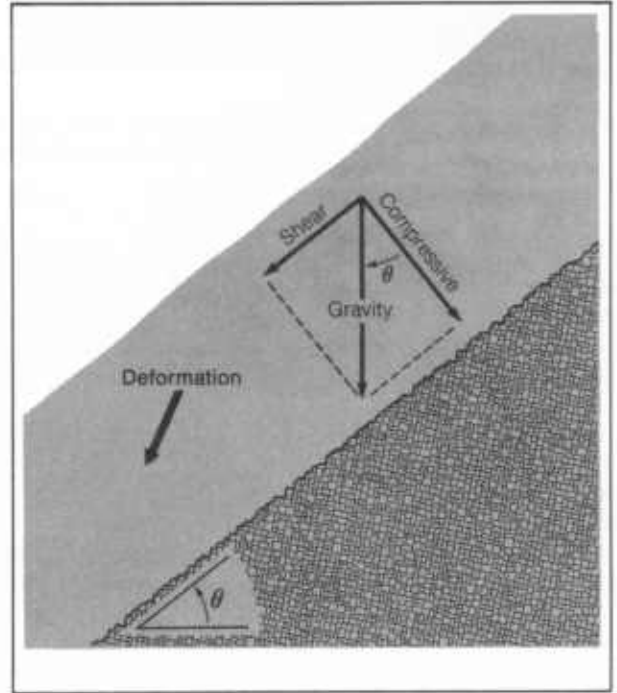
Inclined snowpack
