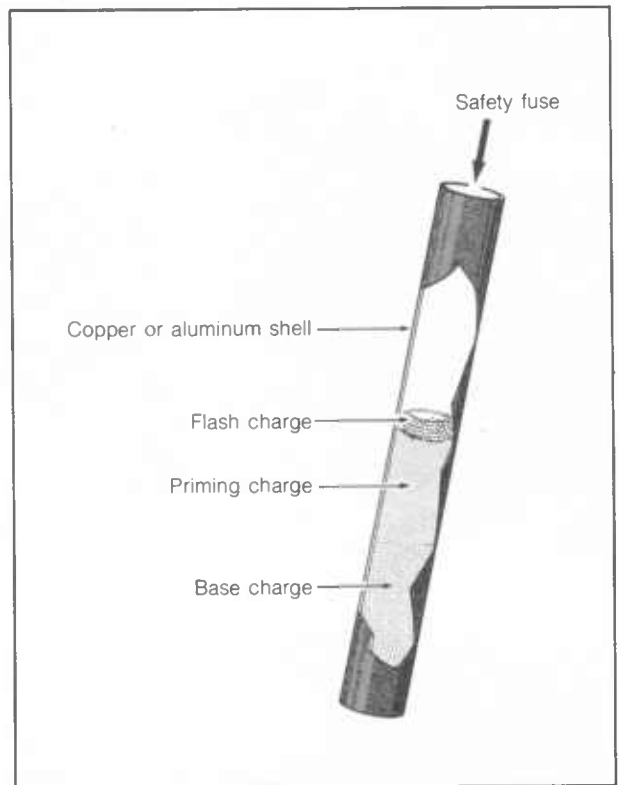
Figure 142.—Typical construction of a blasting cap.
