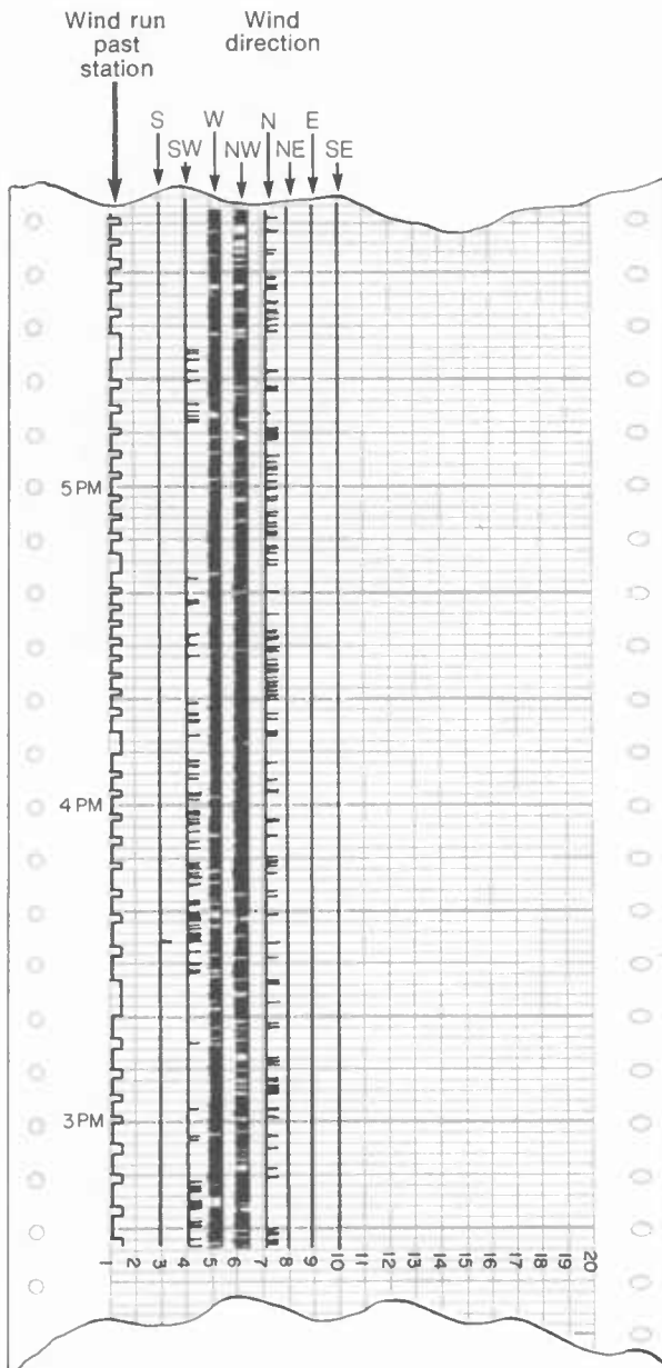
Figure 46.—Digital wind-direction and speed record. Each small notch in the left trace indicates 1 mile of wind travel. Each of the large notches indicates 10 miles of travel. Wind direction is determined from the other traces, by the relative number of marks from each direction. For example, at 4 p.m. the wind was from the west-northwest.
