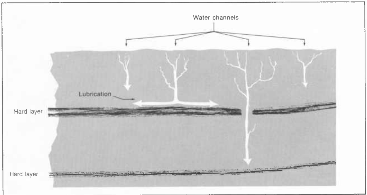
Figure 69.—Free water penetrating the snowpack tends to spread out on top of hard layers and melts or erodes the attachment between the hard layer and the layer above. This effect is known as “lubrication.”
