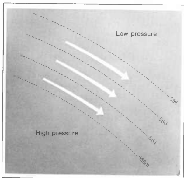
500mb SURFACE
