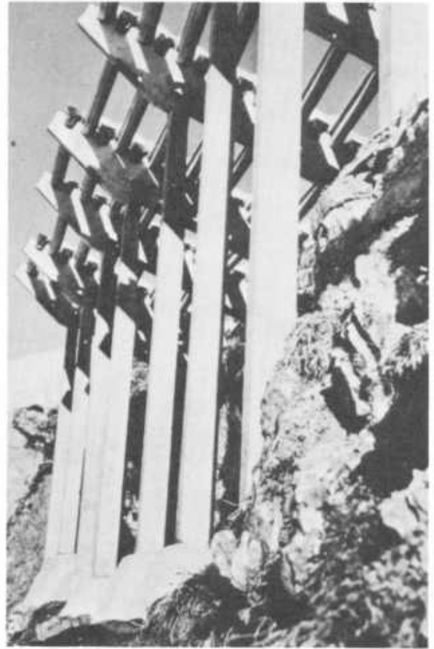
Figure 167.—Rigid supporting structures in the starting zone can be made from a variety of materials: Top left, aluminum frame and braces with wood crossbeams on the grate. Single snow bridges are no longer used; a continuous line of bridges is better. Mattstock Avalanche, near Amden, Switzerland (Wagner and Hopf 1959). Bottom left, aluminum snow bridges. Mattstock Avalanche, near Amden, Switzerland (Wagner and Hopf 1959). Top right, prestressed concrete snow bridge. Kühnihorn, near St. Antonien-Castels, Switzerland (Frutiger and Martinelli 1966).
