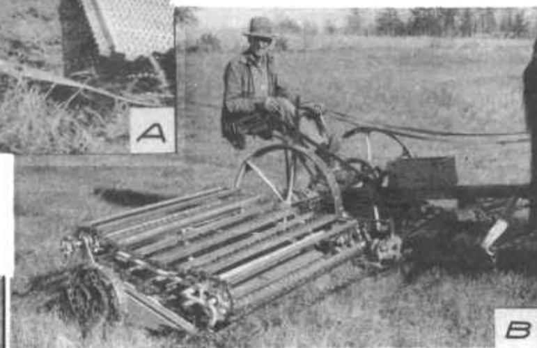
Figure 9. Types of lespedeza seed harvesters. A, Seed pan (open) attached to a mower bar. B, A harvester that has a slatted endless reel to shatter the pods off the stems. C, A harvester that uses spiked slats to push seed hay across the screen.
