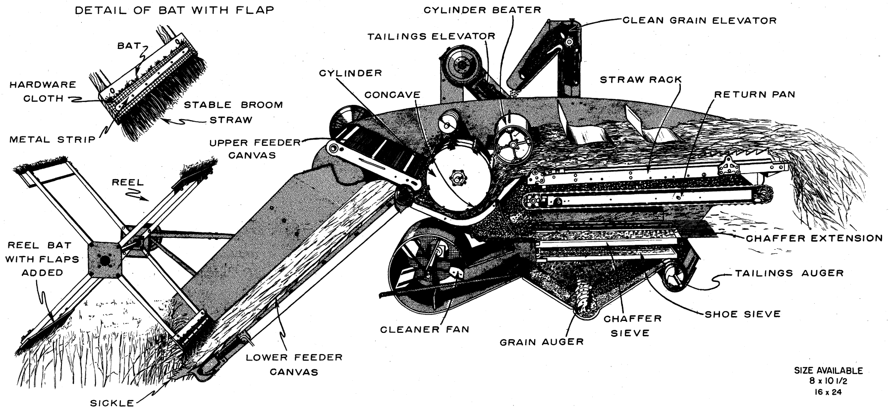
CUTAWAY VIEW SHOWING GENERAL ARRANGEMENT OF VARIOUS UNITS OF A COMBINE
