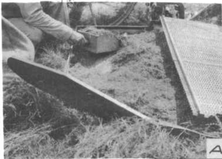
Figure 8. Using a buncher or sweep rake to carry hay to the machine.
