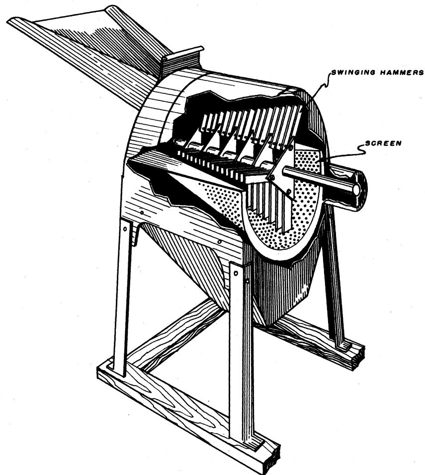
Cut away view of hammer mill showing hammers and screen.
