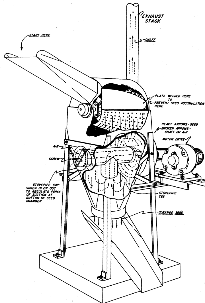
Hammer mill showing air exhaust system for removal of dust and chaff.
