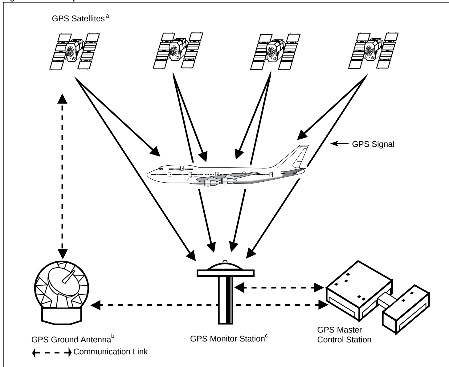
Figure 1: GPS' Components
