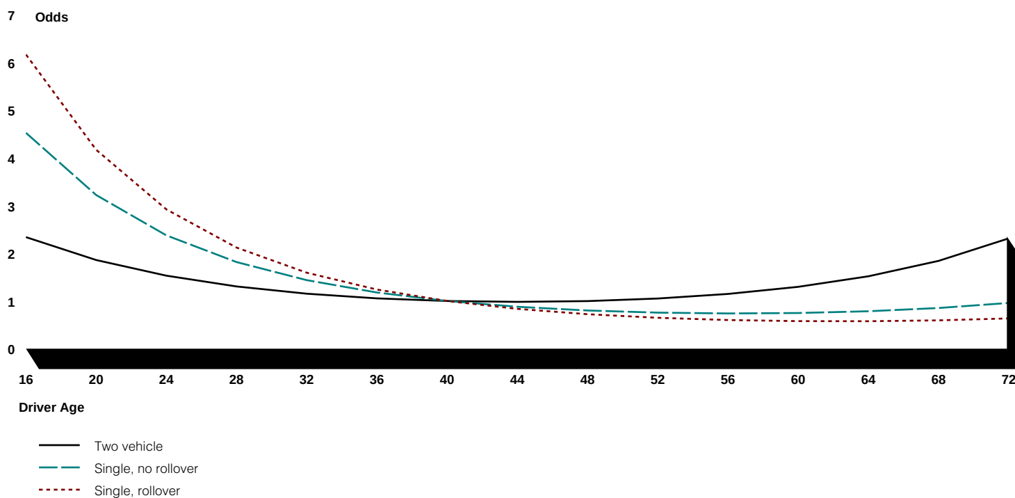
Figure 1: Adjusted Odds Ratios Comparing Crash Involvement by Driver Age a
