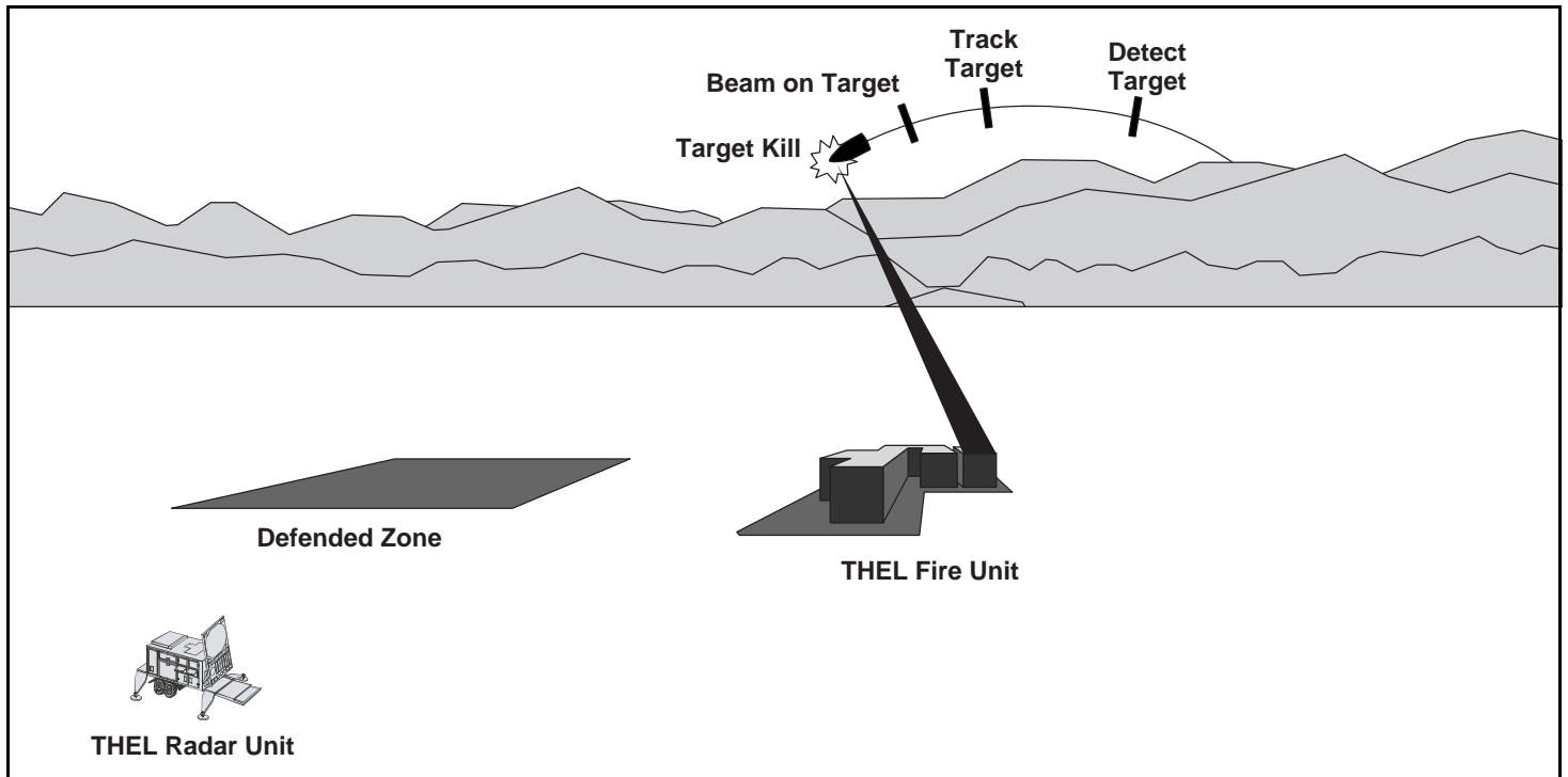
Figure 2.3: THEL Rocket Engagement
