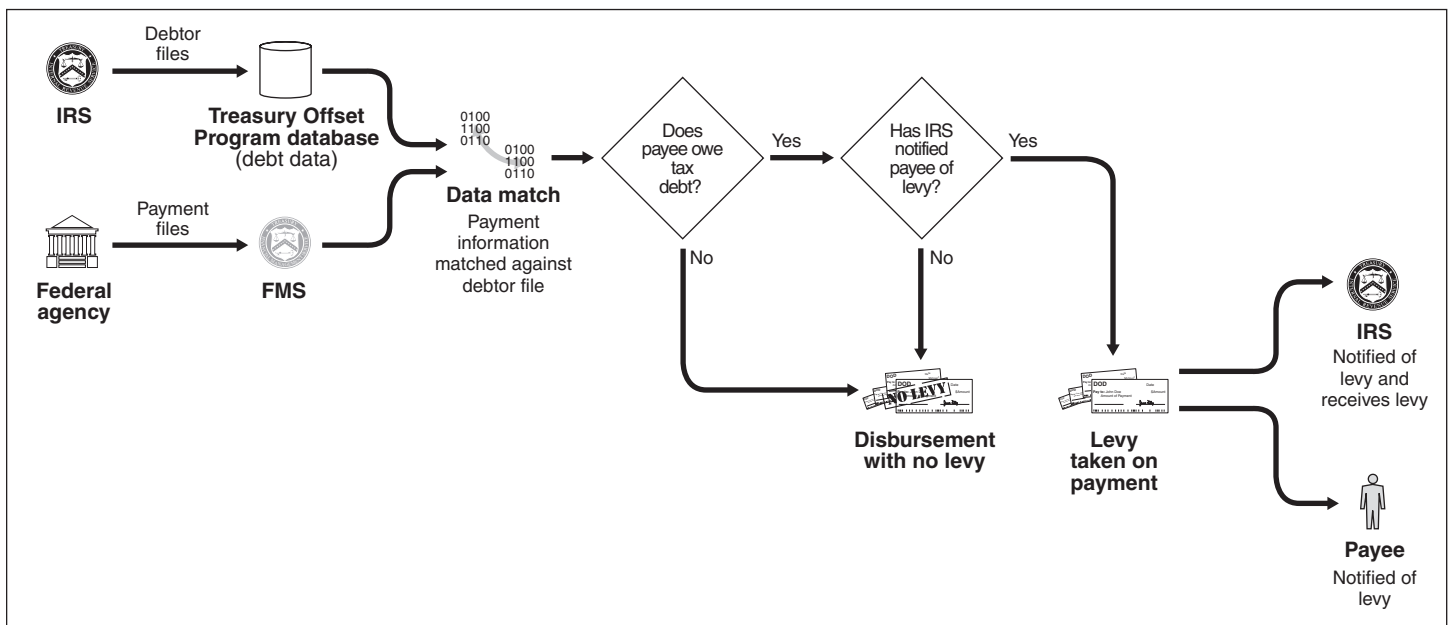
Figure 1: Levy Process
