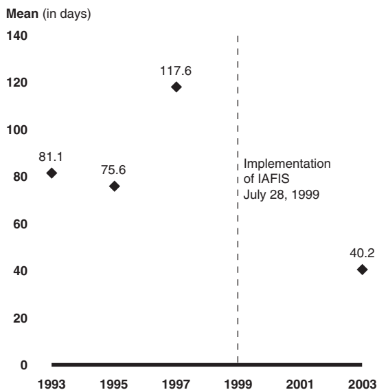
Figure 4: Average Number of Days between the Date of Arrest and the Date That the Criminal Fingerprints Were Received by the FBI or Entered Into IAFIS (for Specific Periods in 1993, 1995, 1997, and 2003)
