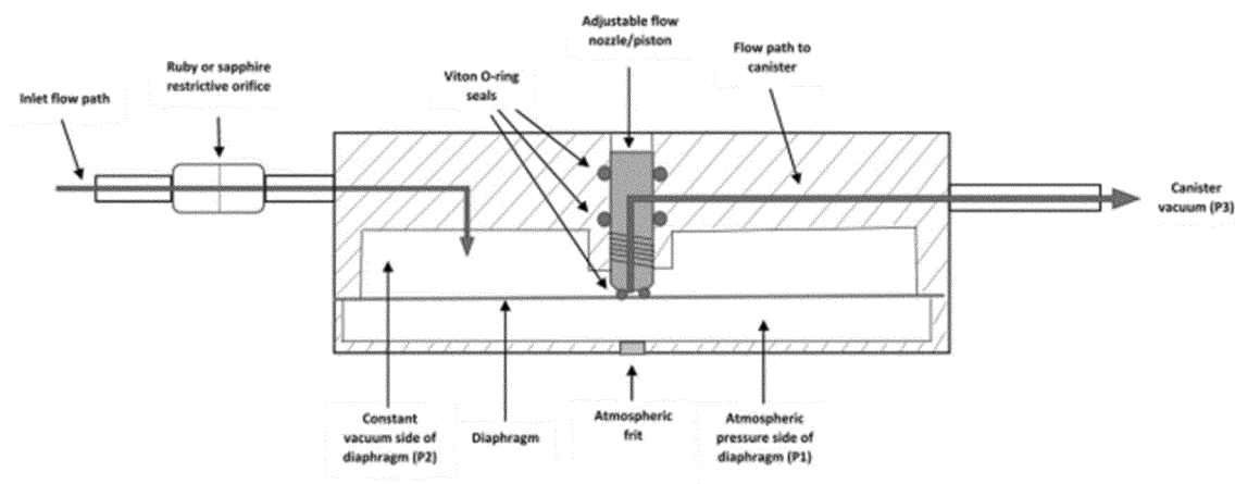
Figure 2. Mechanical Flow Control Device
