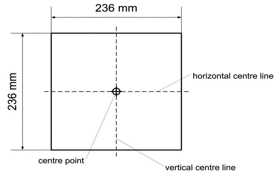
Figure 10: Bumper Corner Gauge 103
