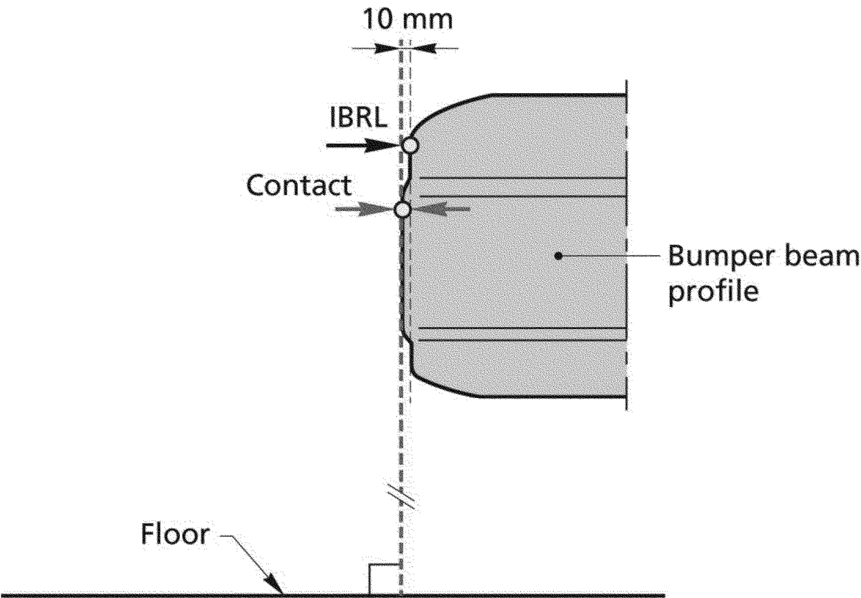
Figure 6: Internal Bumper Reference Line (IBRL) 77
