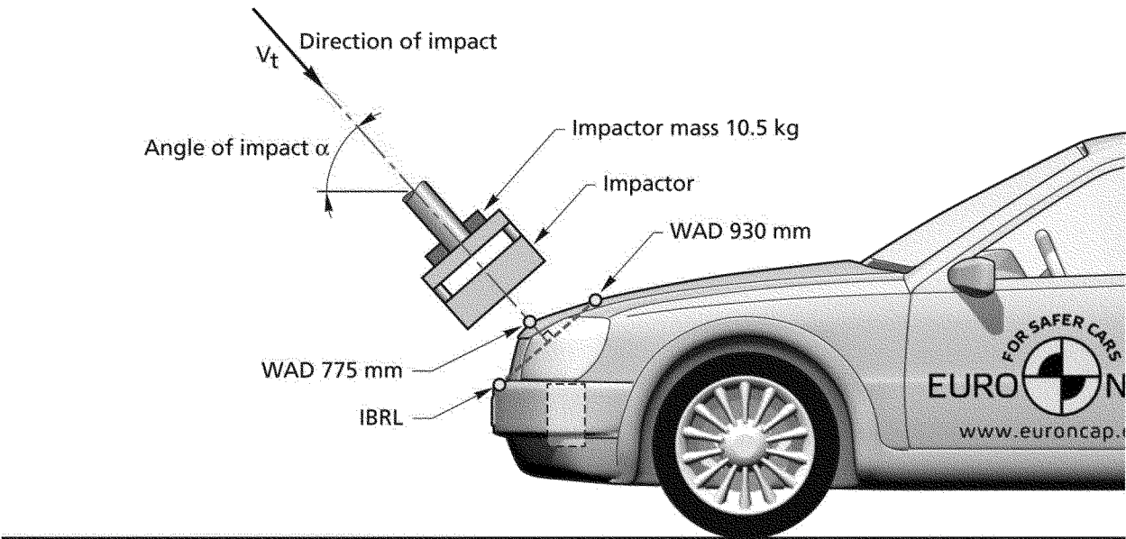
Figure 7: Upper Legform to WAD775 Test Setup 78
