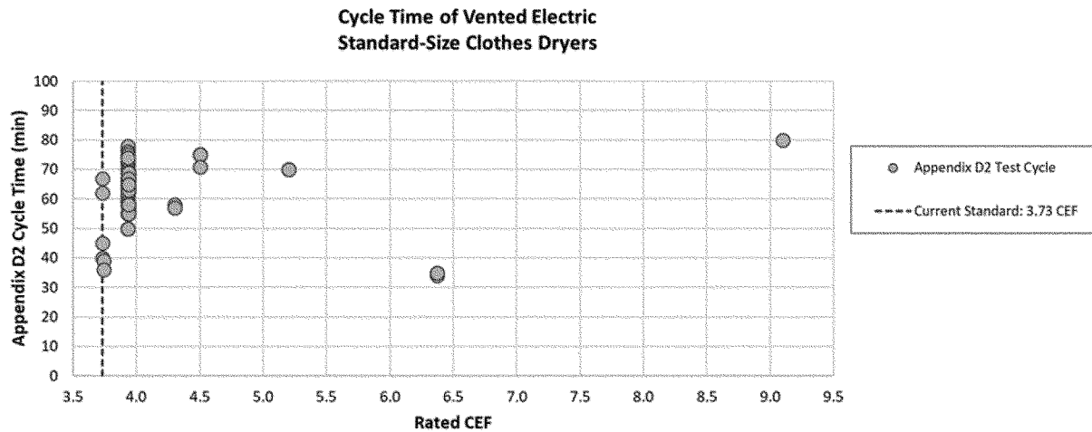
Figure II.3 DOE Cycle Time Data for Vented Electric Standard-Size Clothes Dryers Using Appendix D2
