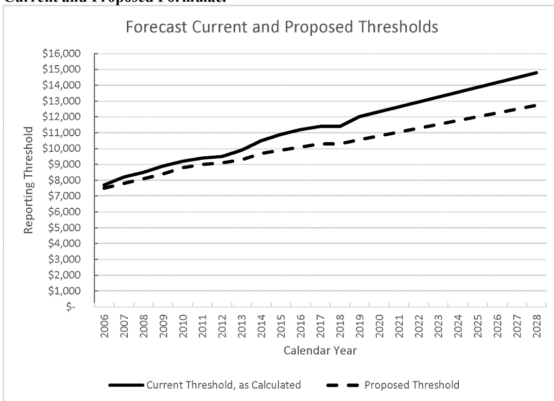
Figure 4: Forecast from 2019 to 2028 of Reporting Thresholds Calculated Using the Current and Proposed Formulae.
