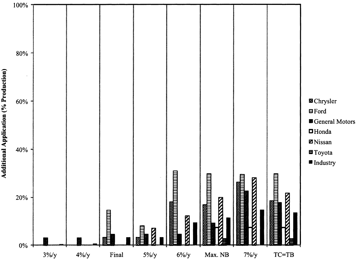
Figure IV.F-6 Additional Application of CISG and Strong HEV Systems (MY 2016)
