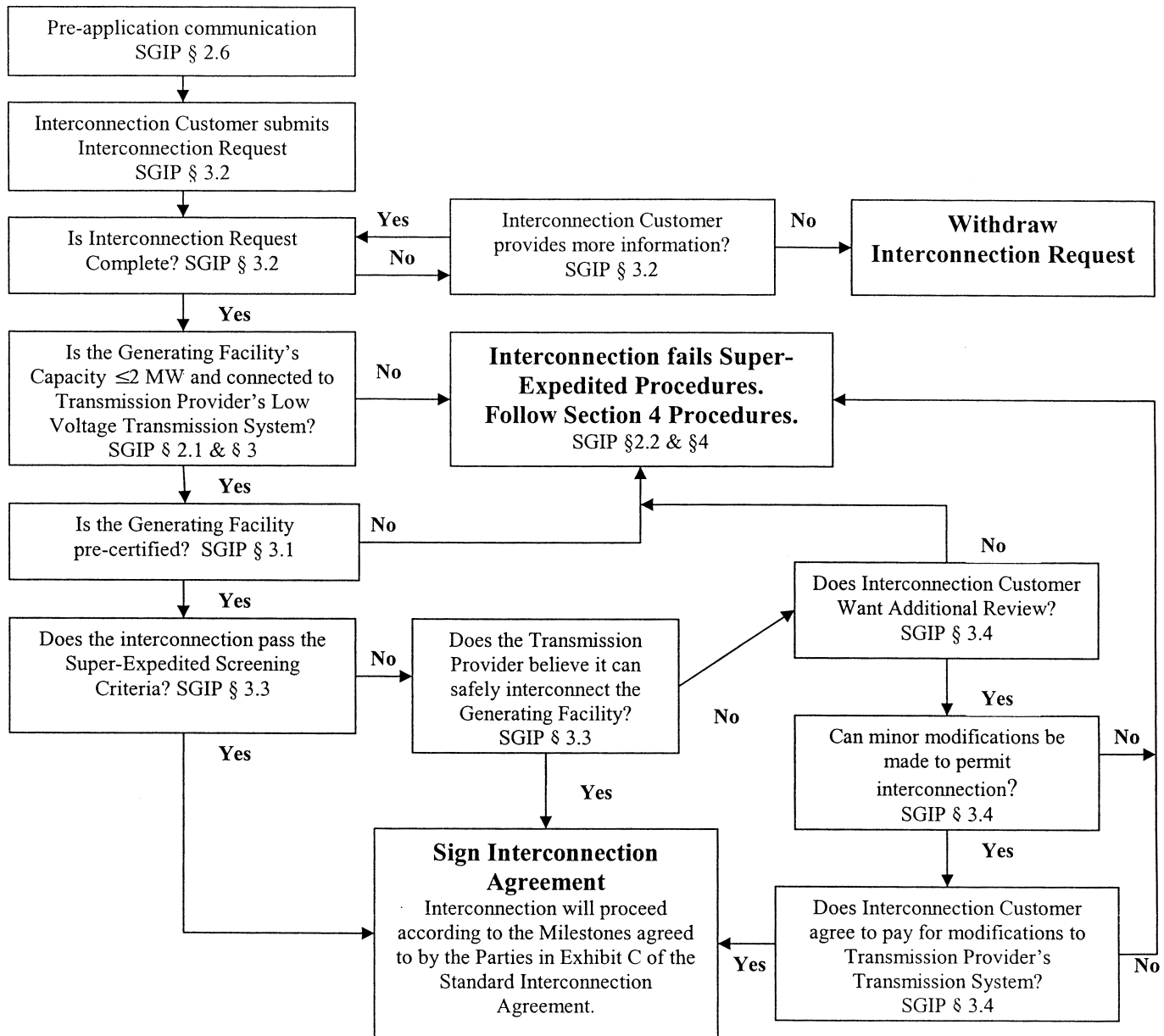
Flow Chart of Super-Expedited Procedures for Interconnecting a Small Generating Facility No Larger than 2 MW to a Low-Voltage Transmission System
