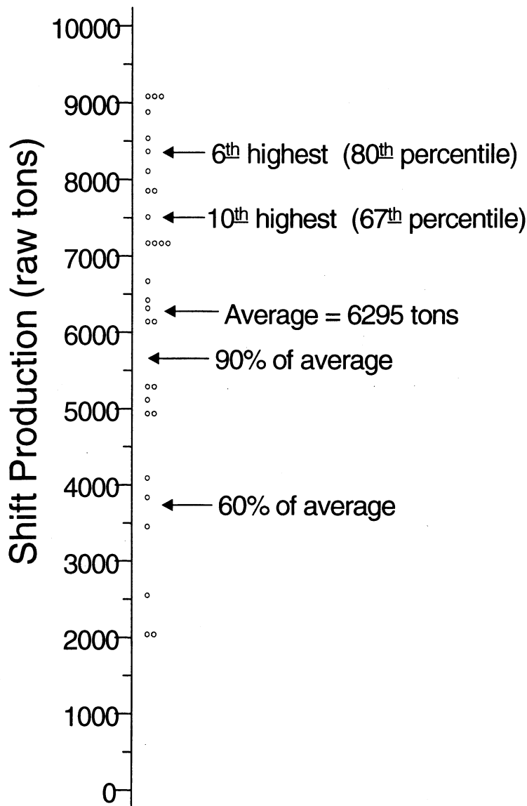
Figure 1. Example of a typical distribution of 30 shift production levels achieved at a longwall MMU.
