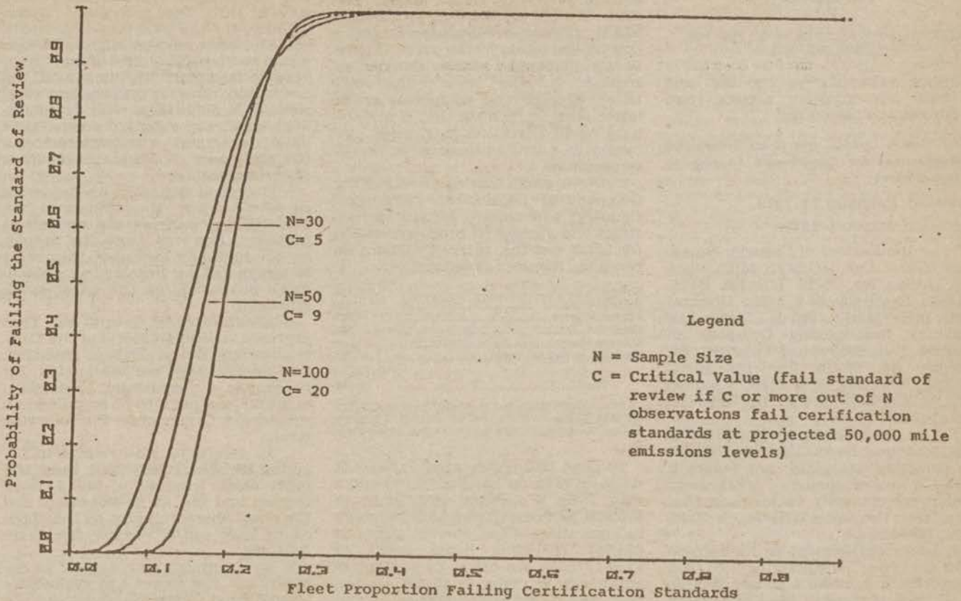
Probability of Failing the Standard of Review for Different Sample Sizes and Critical Values versus the True Proportion in the Fleet Failing Certification Standards
