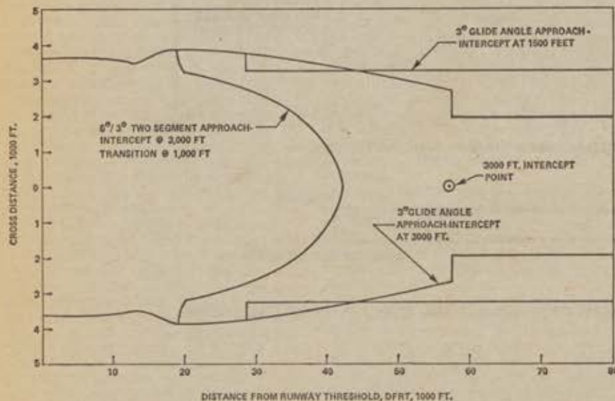
FIGURE 3. 90 EPNdB CONTOURS FOR VARIOUS APPROACHES: 707 AIRPLANE [FR Doc.74-30539 Filed 12-31-74;3:59 pm]
