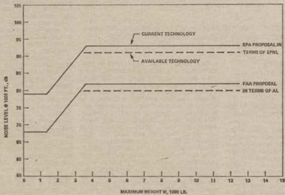
FIGURE 3. NOISE COMPLIANCE LEVELS IN TERMS OF EFFECTIVE PERCEIVED NOISE LEVEL (EPNL) AND A-WEIGHTED LEVEL (AL)
