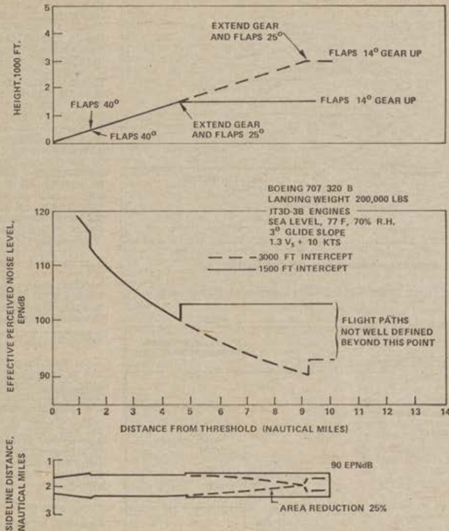
FIGURE 1. NOISE DATA FOR 1500 AND 3000 FT INTERCEPT ALTITUDES
