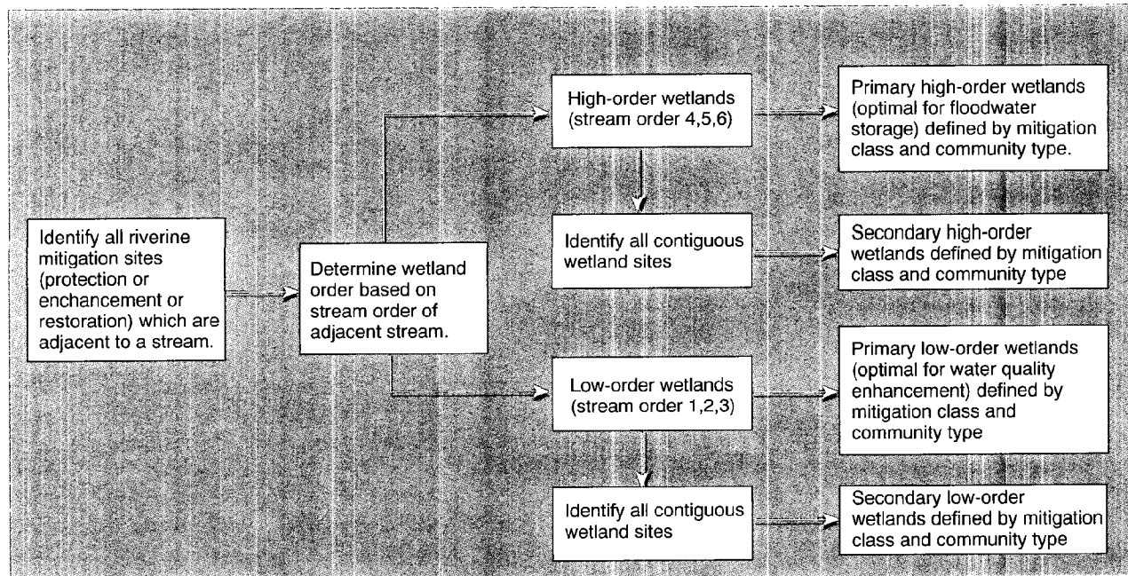
Figure 2. Steps in water quality and floodwater storage analyses
