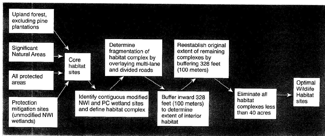
Figure 1. Steps in wildlife habitat analyses
