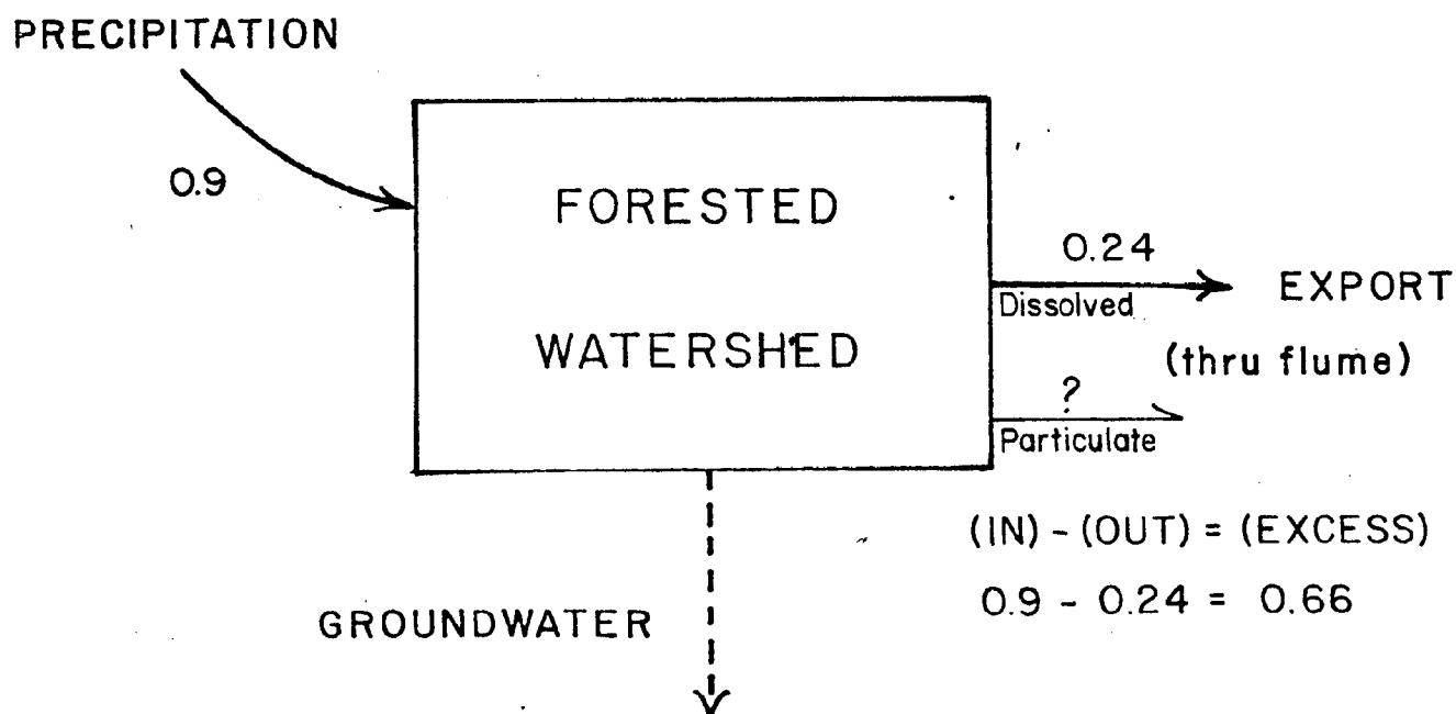
Figure 13. Yearly phosphorus budget for agricultural and forest watersheds at Horn Point
