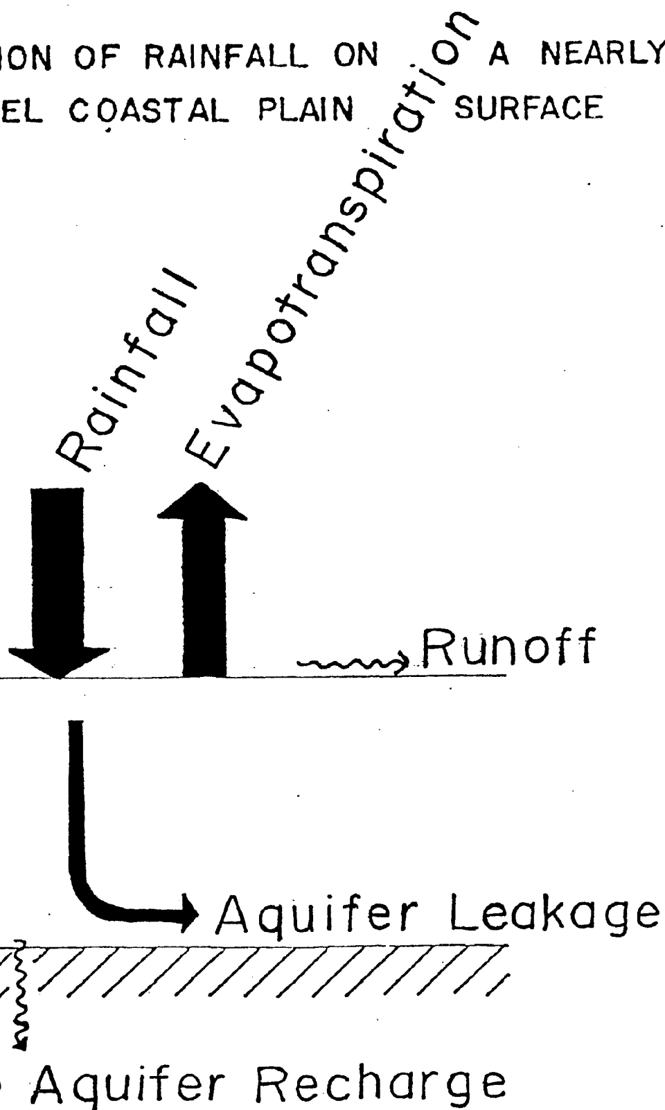
Figure 2. Graphical description of water movement.
