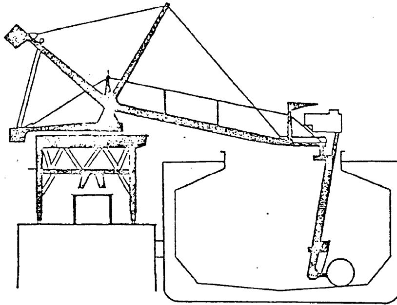
Figure 15: Continuous type ship unloader.
