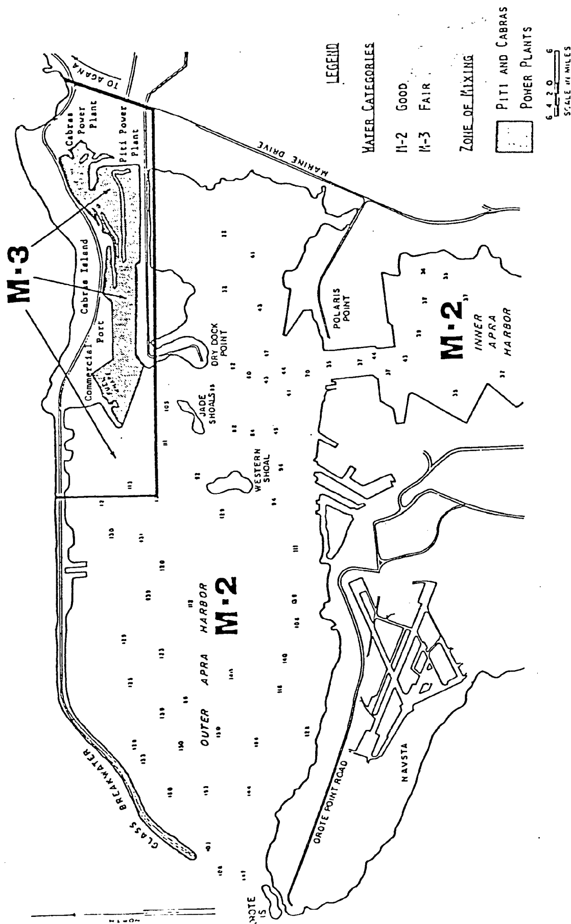
Figure 9: Water Classification and Zone of mixing for Apra Harbor.
