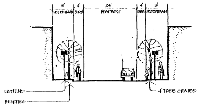
TYPICAL EAST/WEST SECTION FOR A 20' R.O.W. SEGMENT ACDFHIKL
