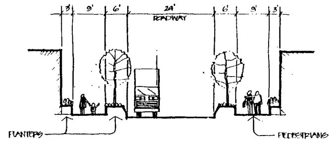
ADIR STREET 60' ROW. TRUCK ROUTE NORTH OF FRANKLIN SEGMENT M
