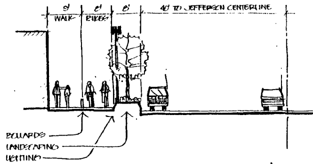
JEFFERSON AVENUE 120' ROW BETWEEN MCLELLITT & THE RAILROAD BRIDGE SEGMENT O
