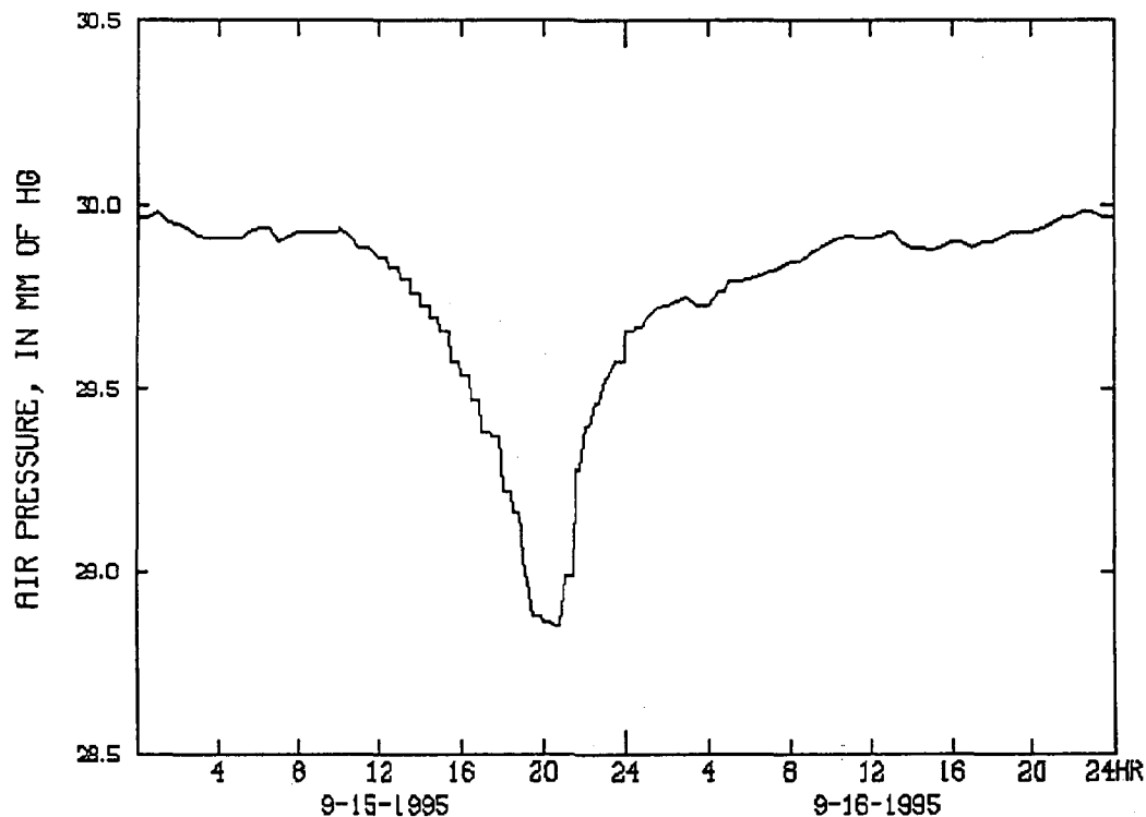
Figure 1-1b. USDA Air Pressure Record from St. Croix.
