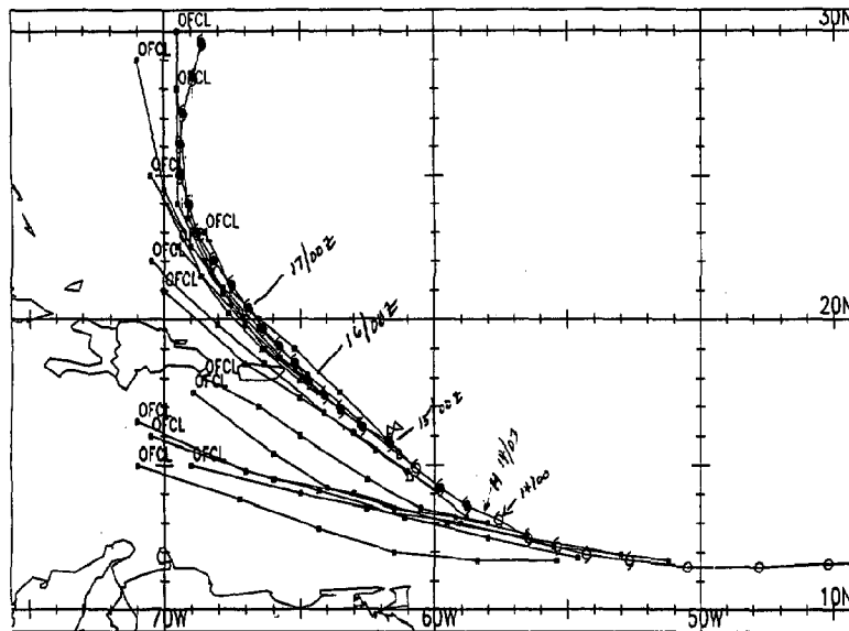
Figure 5-1. Composite of NHC forecast tracks associated with Marilyn. (Chart provided by NHC)
