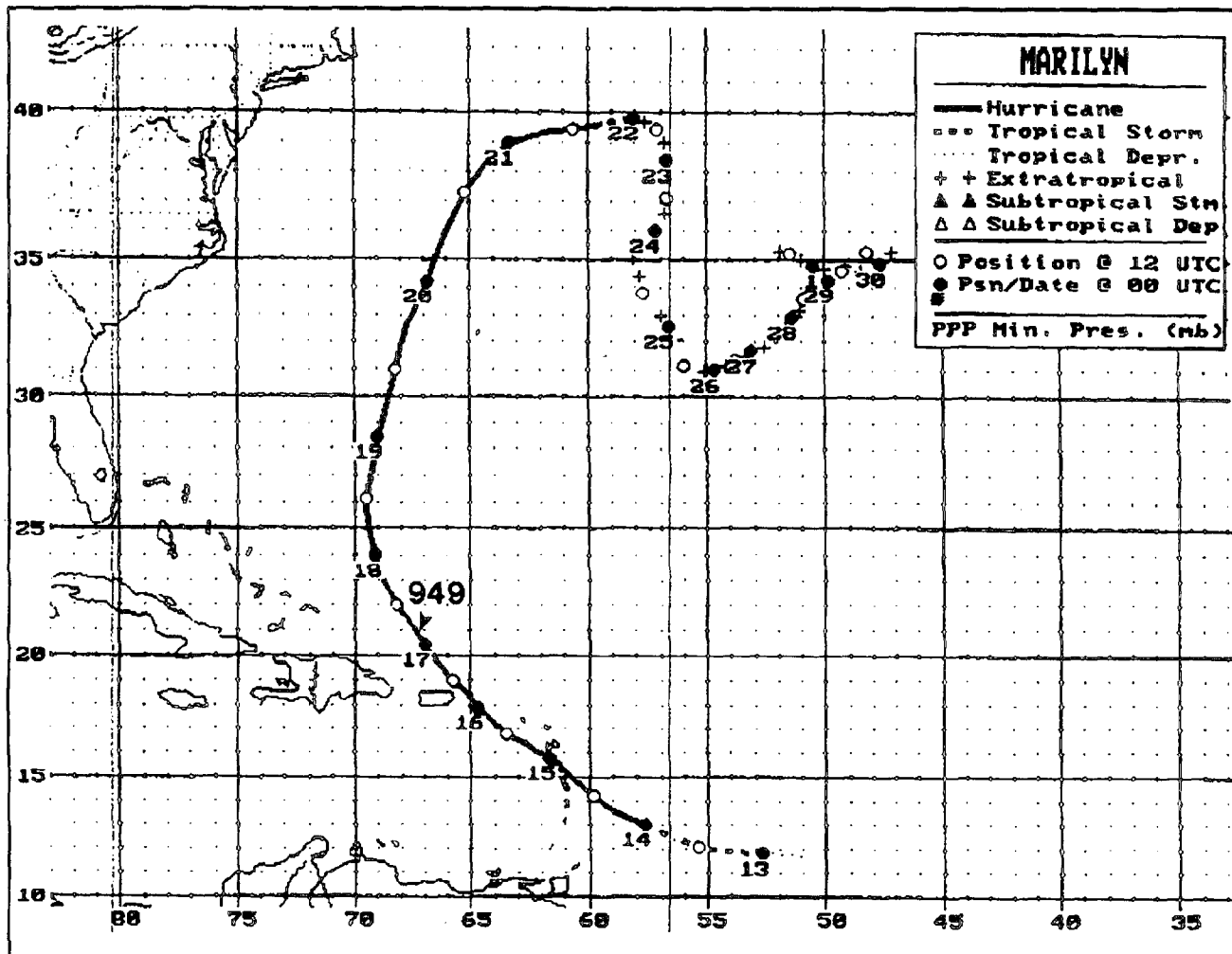
Figure 5-2. NHC's "best" track of Hurricane Marilyn. (Chart provided by NHC)
