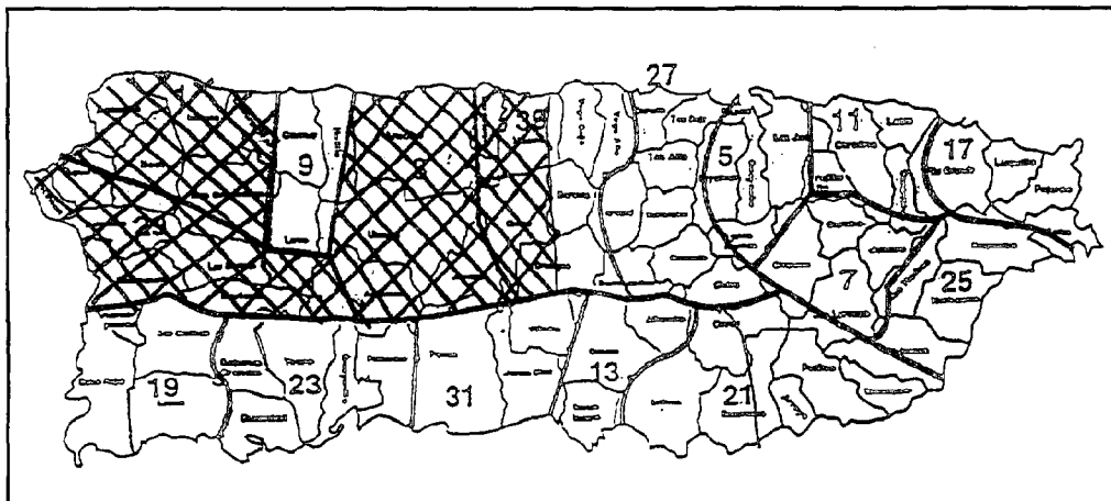
Figure 5-4. Map showing FFW areas effective 9:23 a.m., AST, Saturday, September 16. (Map courtesy of WSFO San Juan)
