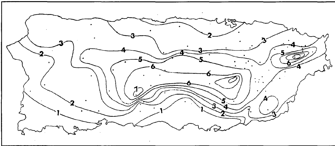
Figure 5-5. Map showing rainfall distribution from Marilyn across Puerto Rico. (Map courtesy of Reggina Garza, using USGS data)
