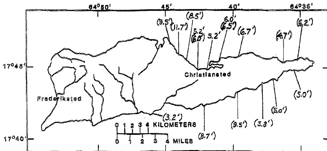
Figure 1-3. USGS Storm Tide Measurements on St. Croix.
