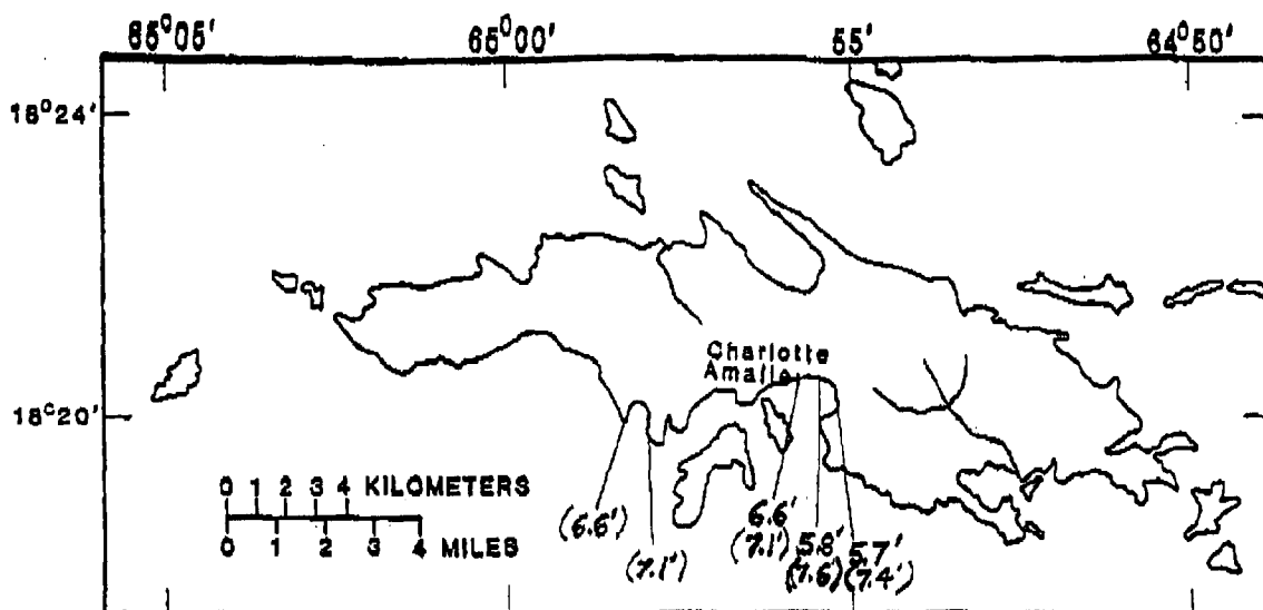
Figure 1-6. USGS Storm Tide Measurements on St. Thomas.
