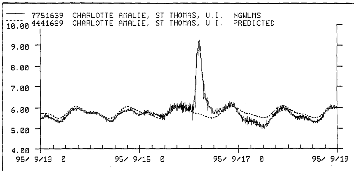
Figure 1-7. NOS Water Level Measurements in Charlotte Amalie Harbor.
