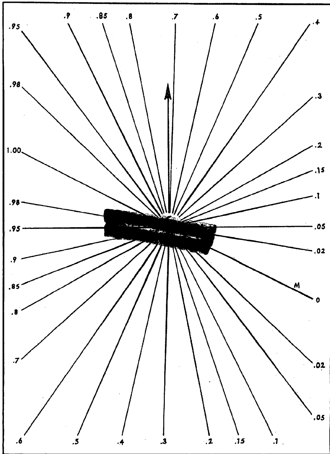
Fig. 25 NOMOGRAM FOR WIND FIELD ASSYMETRY FACTOR
