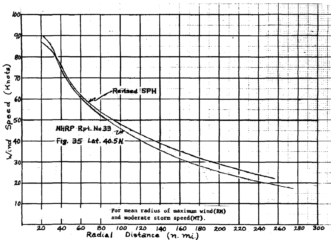
Fig. 18.--COMPARISON OF WIND FIELD PROFILES FOR ZONE 4
