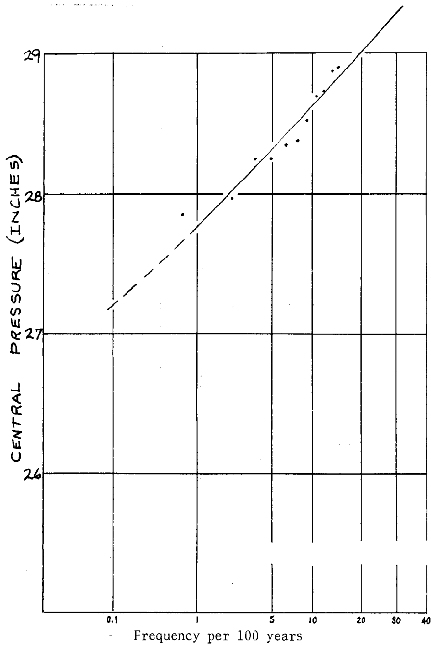
Fig. 6.--CUMULATIVE FREQUENCIES OF HURRICANE CENTRAL PRESSURES(1900-1971) ZONE 4
