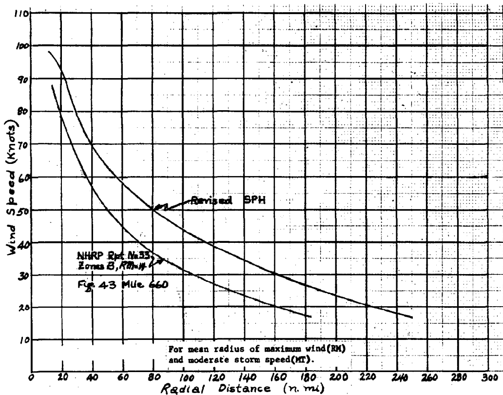
Fig. 20.--COMPARISON OF WIND FIELD PROFILES FOR ZONE B
