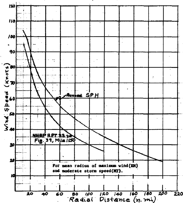
Fig. 19.--COMPARISON OF WIND FIELD PROFILES FOR ZONE A
