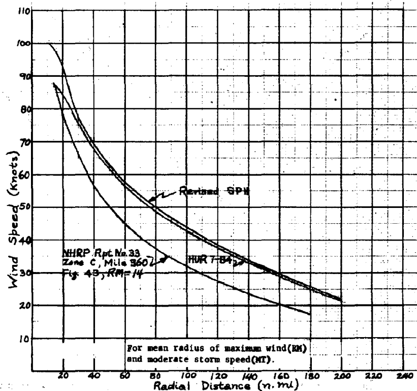
Fig. 21.--COMPARISON OF WIND FIELD PROFILES FOR ZONE C
