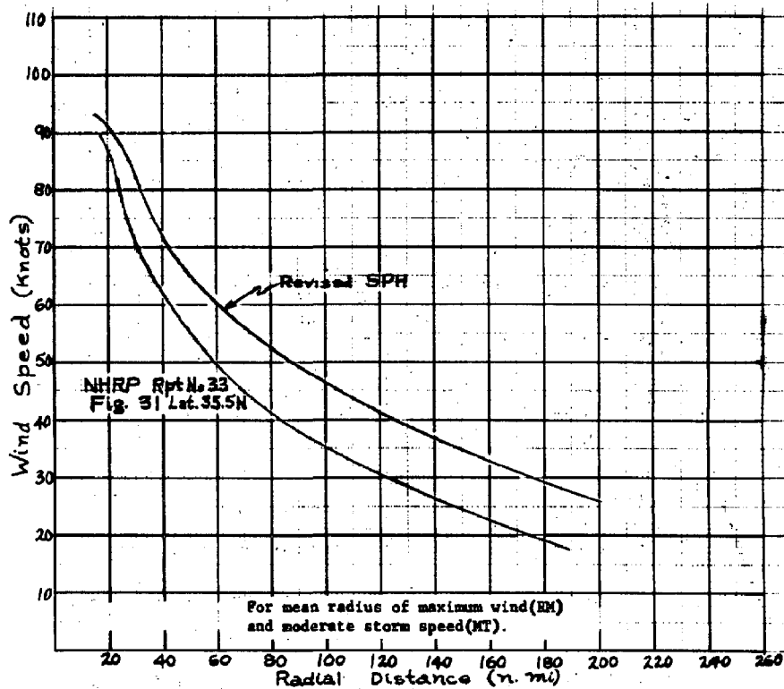
Fig. 17.--COMPARISON OF WIND FIELD PROFILES FOR ZONE 3
