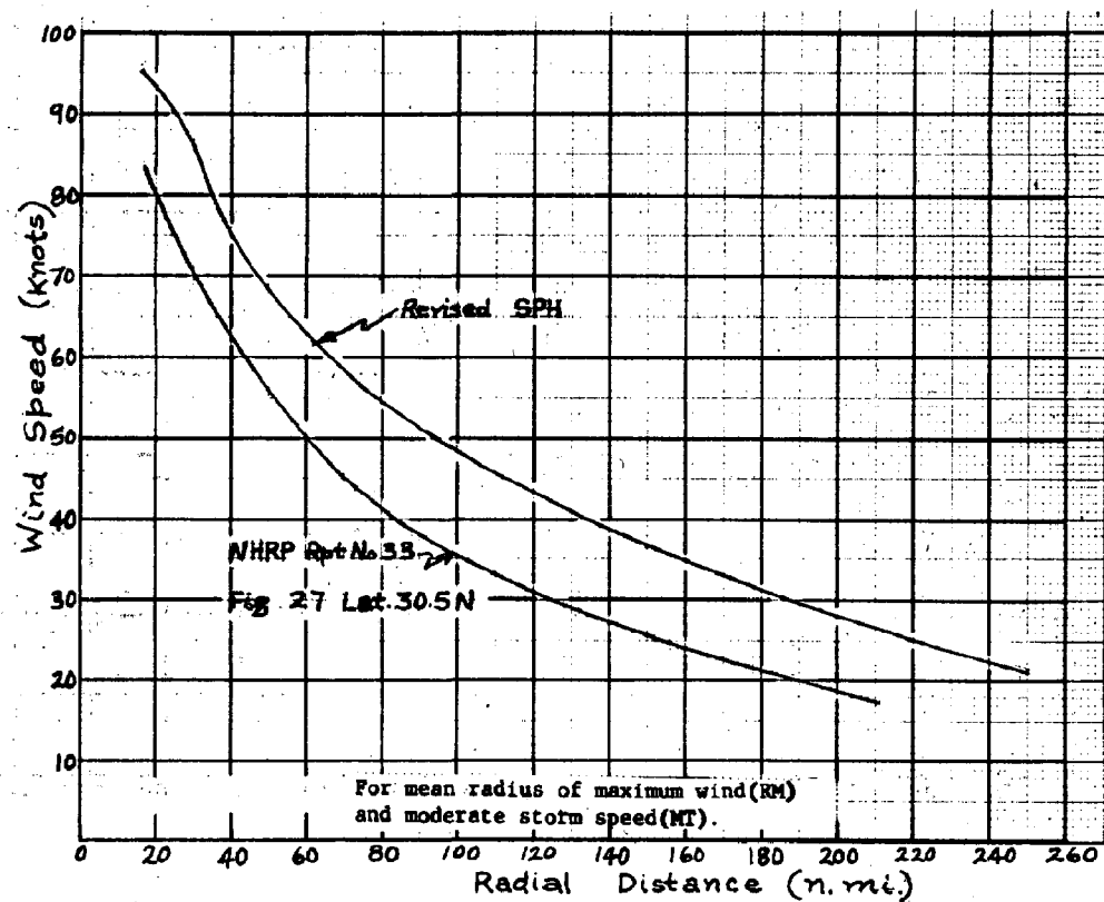
Fig. 16.--COMPARISON OF WIND FIELD PROFILES FOR ZONE 2
