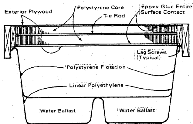
30 WATER-BALLASTED FLOATING DOCK
