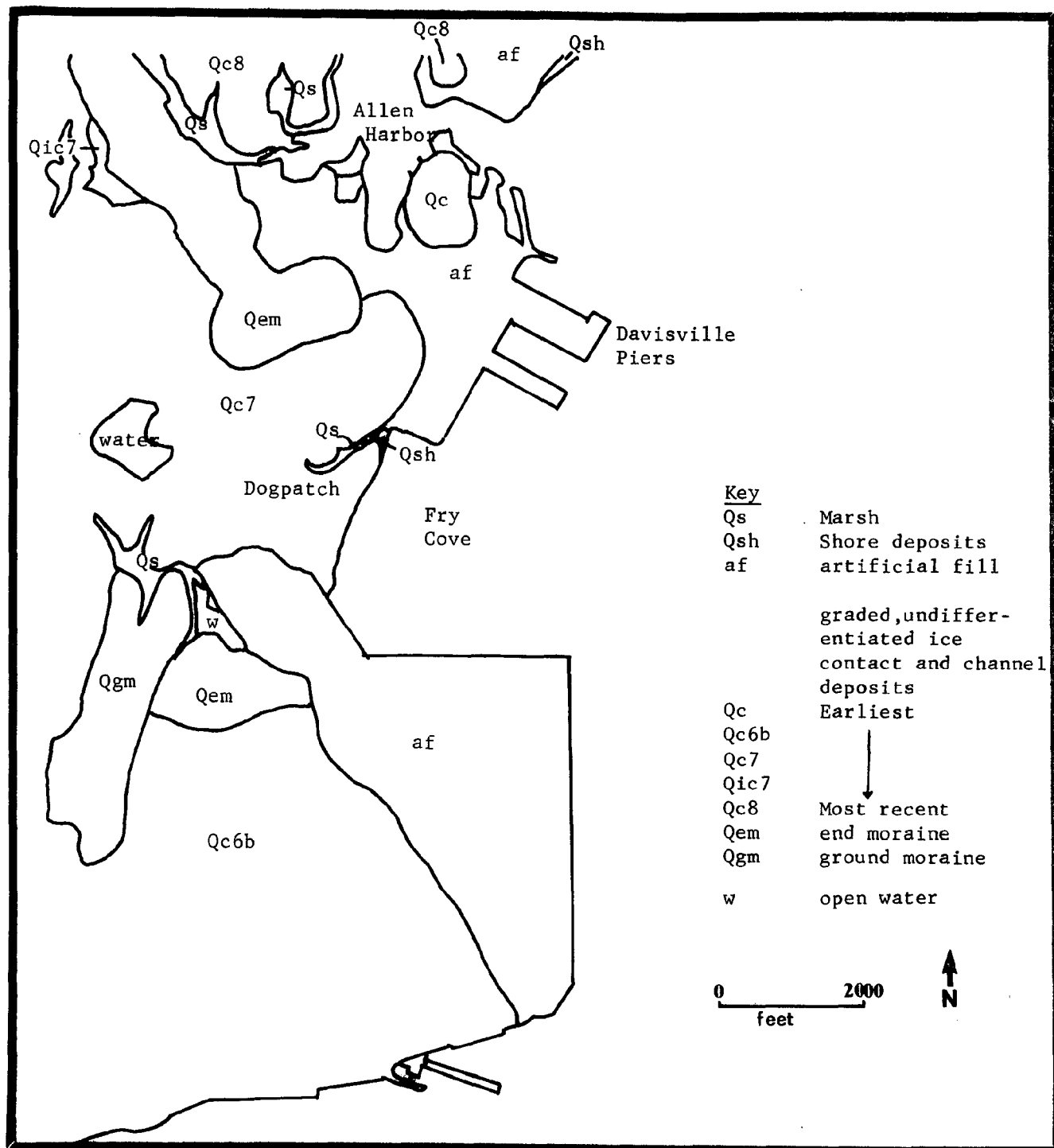
Figure 4-2 Surficial Geology of Davisville Source: J.P. Schafer, 1961. Surficial Geology of the Wickford Quadrangle. U.S. Geological Survey, Washington D.C.
