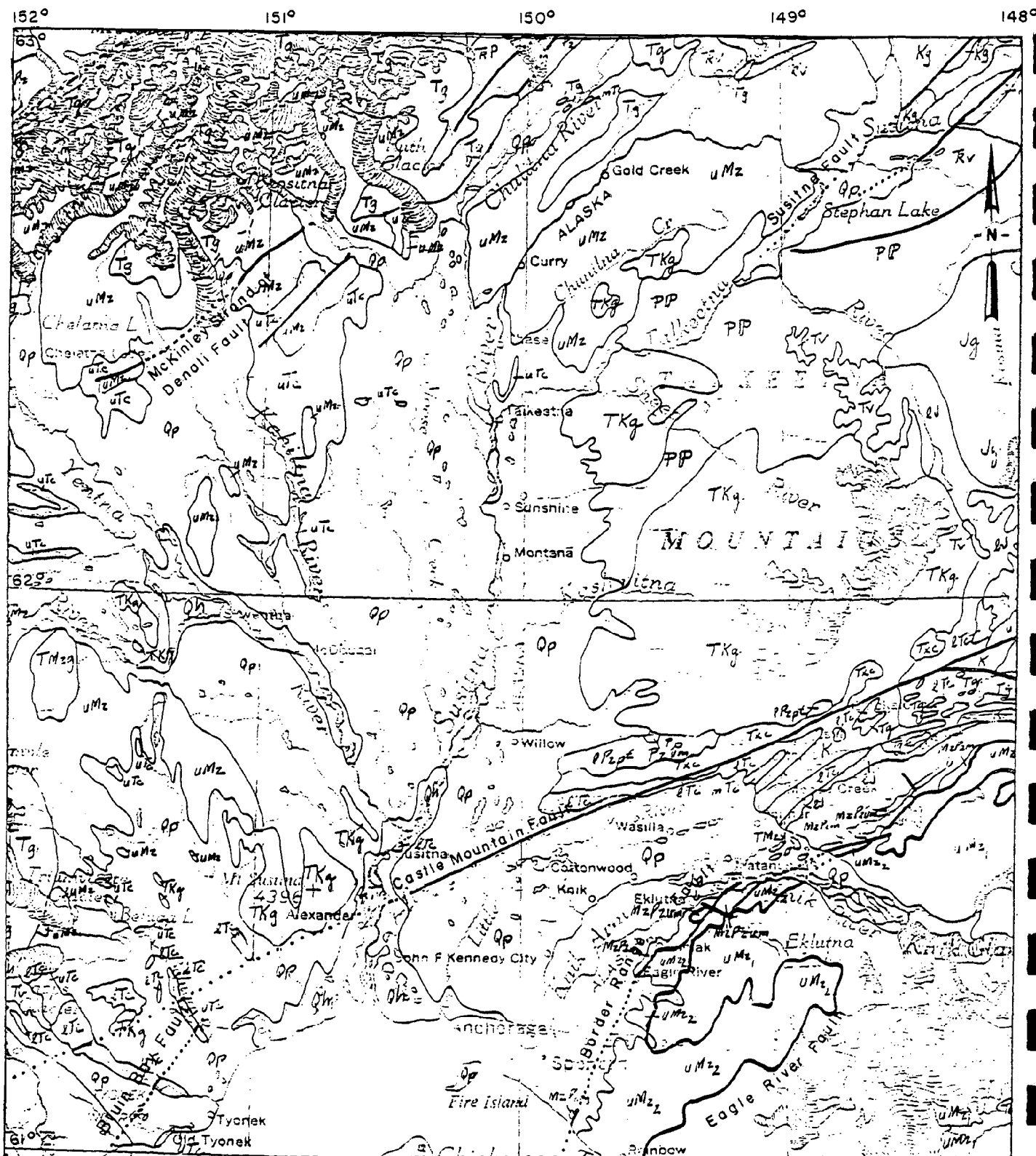
GENERAL GEOLOGIC MAP of MATANUSKA-SUSITNA BOROUGH COASTAL MANAGEMENT DISTRICT
