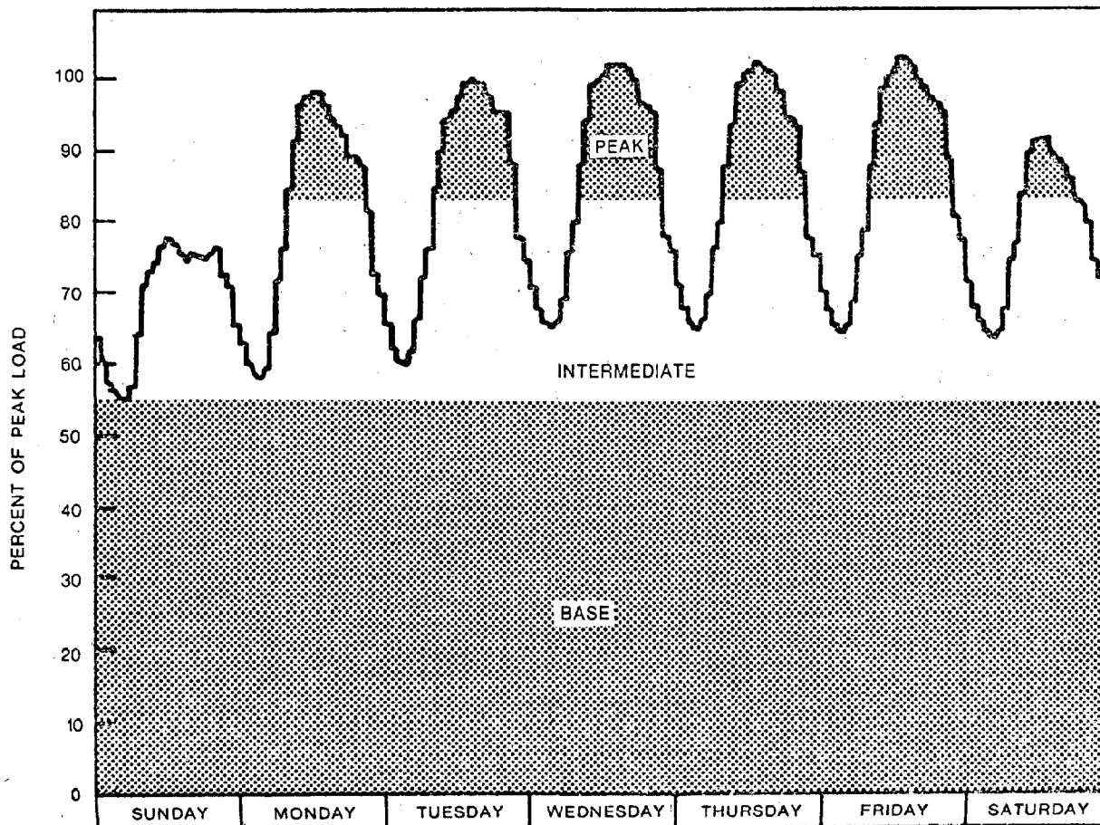
Figure 37 WEEKLY LOAD CURVE
