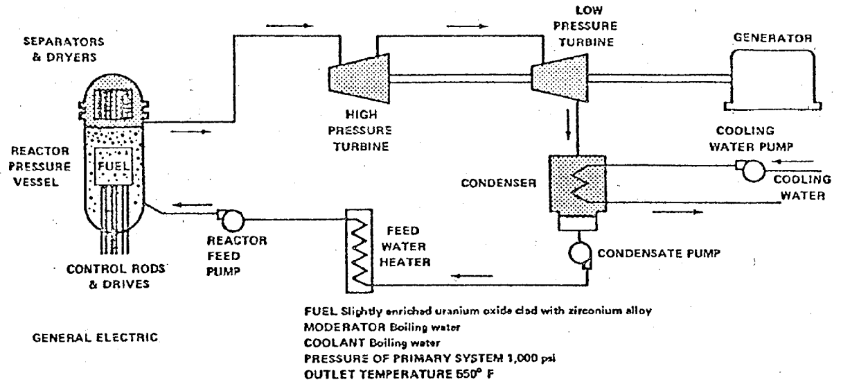
Boiling Water Reactor Power Plant
