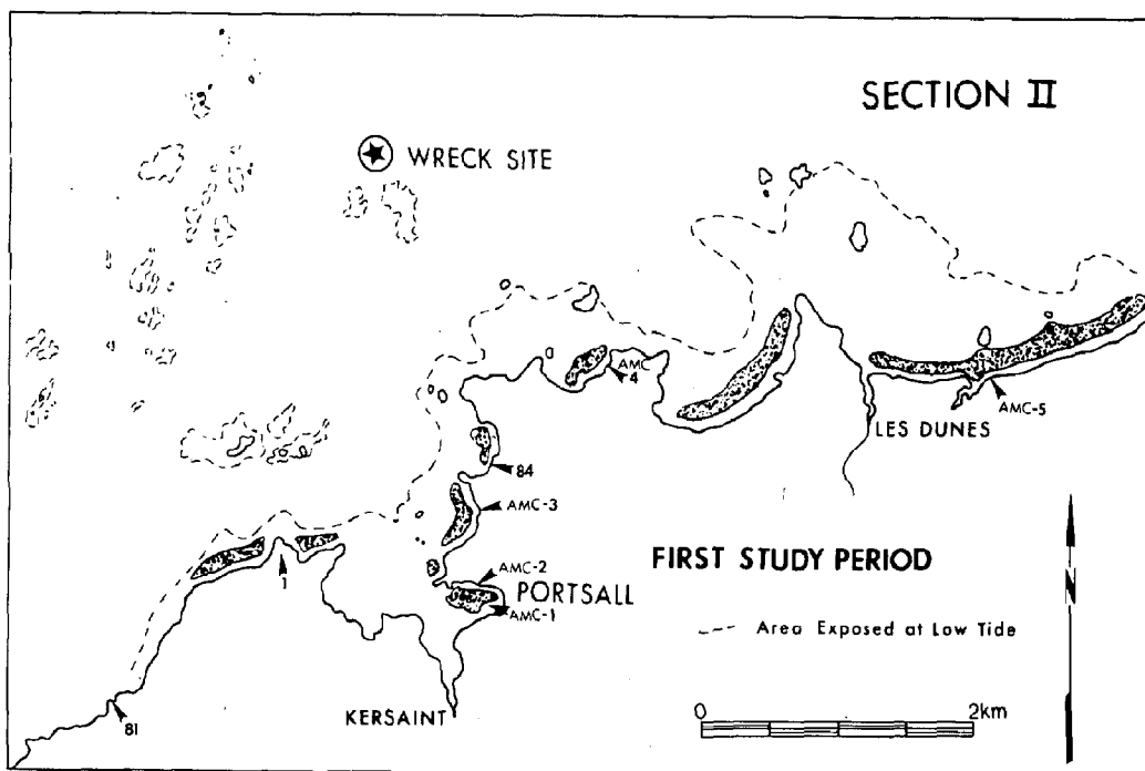
Figure 4-13. Locations of observation stations in Section II, the Port-sall area, during the first study period (March 19 to April 2). Heavy oil accumulations are indicated by the dark-stippled pattern.
