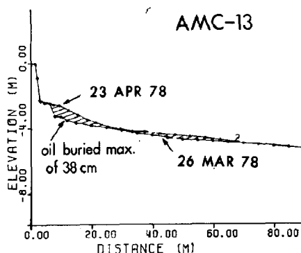
Figure 4-36. Comparison of topographic profiles on March 26 and April 23. Oil was buried to a maximum depth of 38 cm by the deposition of clean sand. Therefore, the beach appeared unoiled.
