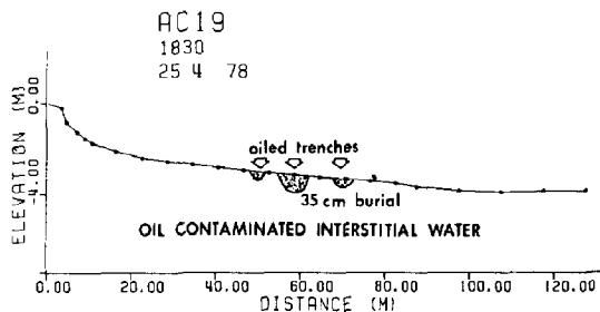
Figure 4-52. Topographic beach profile of station AMC-19 on April 25. Oiled trenches remaining from the clean-up operation are indicated.
