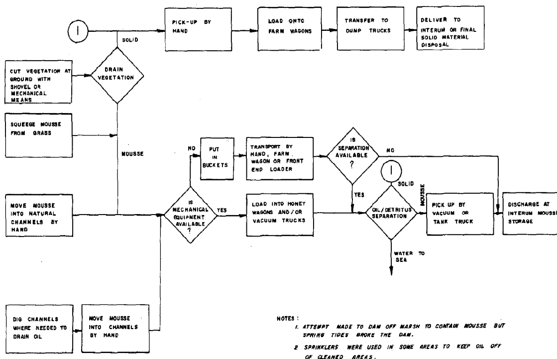
Figure 6-15. Unit process: Cleaning of Ile Grande marsh.
