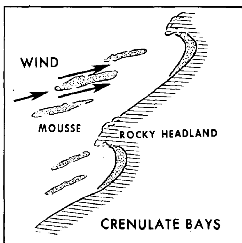
Figure 4-65. Entrapment of oil by crenulate bays. Generally, the southerly section of each bay remained free of oil.
