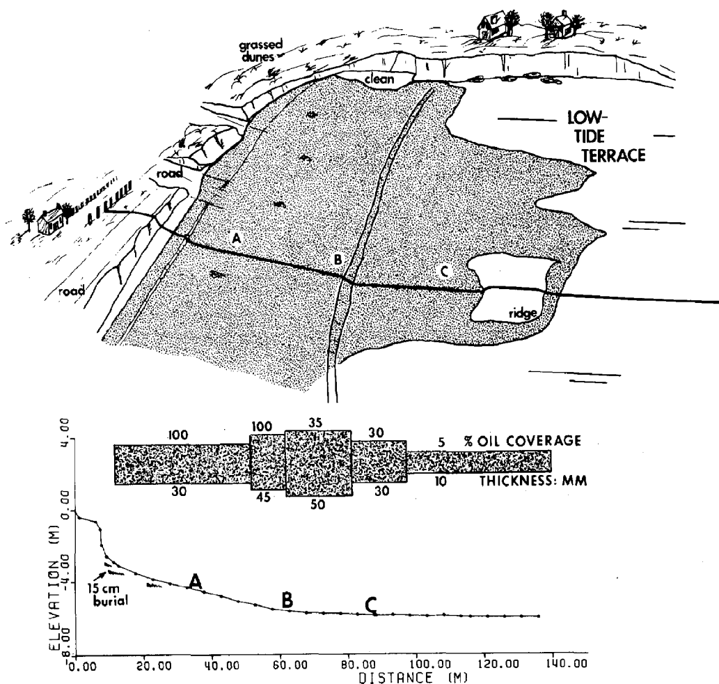
Figure 4-33. Topographic profile and oil coverage at station AMC-12 on March 27. The thickness of the oil coverage line is proportional to actual oil thickness. Heaviest accumulations occurred on the low-tide terrace in a low-relief runnel behind a ridge.
