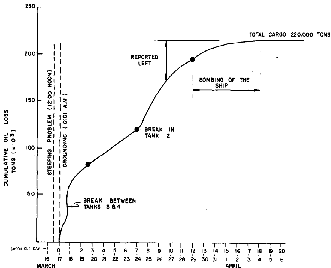
Figure 6-5. Estimated cumulative oil release from Amoco Cadiz spill.
