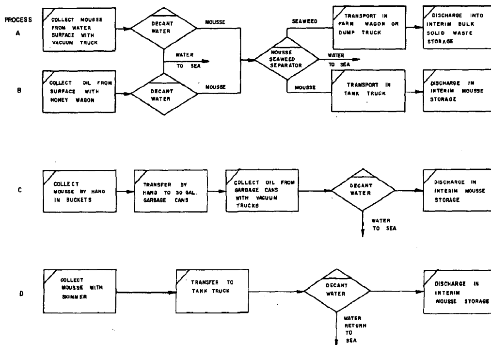
Figure 6-10. Unit process: Removal of mousse from water surface to interim storage.
