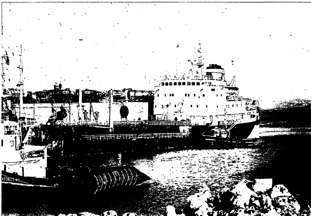
6-20. A small coastal tanker is loaded with the oil/water mousse removed from the water's surface and the beaches. Note the large backlog of trucks waiting to be loaded.
