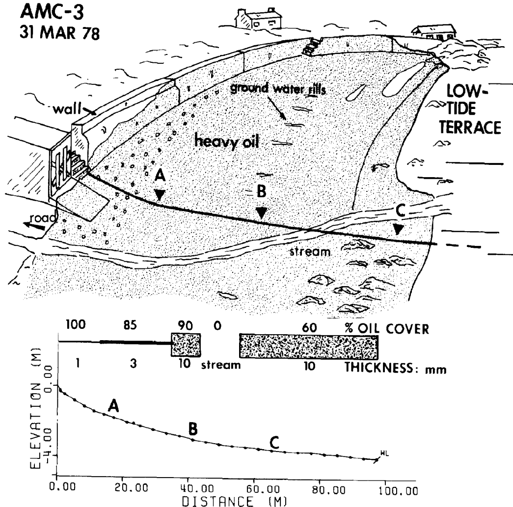
Figure 4-20. Topographic profile and oil coverage at station AMC-3 on March 31. High spring tides of March 25-28 were responsible for spreading oil up the wall behind the beach. Sediment sampling sites A, B, and C are indicated.
