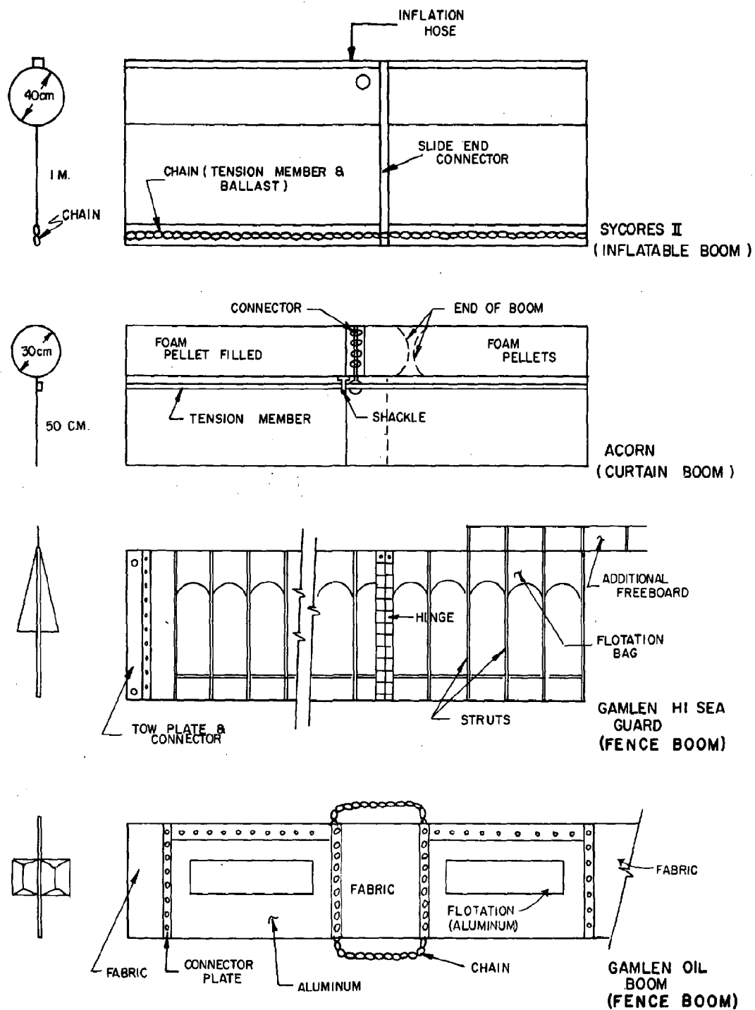
Figure 6-17. Four types of booms used during spill cleanup: (a) Sycores II; (b) Acorn; (c) Gamlen Hi-Sea Boom; and (d) Gamlen small fence boom.
