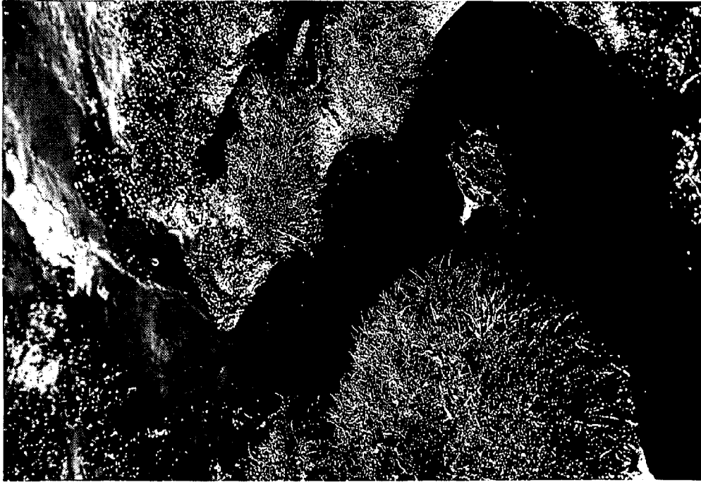
4-3. Mousse in tidal creek at Ile Grande marsh. Photograph was taken at low tide. The mousse flow is caused by late stage drainage of the marsh. (2 April 1978)
