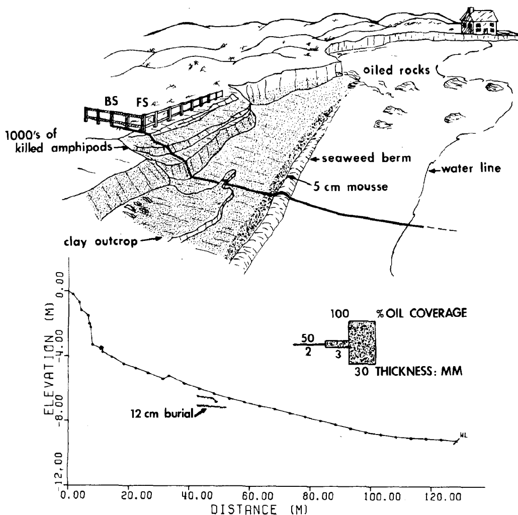
Figure 4-21B. Topographic profile and oil coverage at station AMC-4 on March 31. During the previous week, the shoreline had eroded significantly back, removing most of the oil from the lower beachface and exposing a relict red clay surface. Thousands of dead amphipods ( Talitrus saltator ) littered the dune scarp (Plate 4-27).
