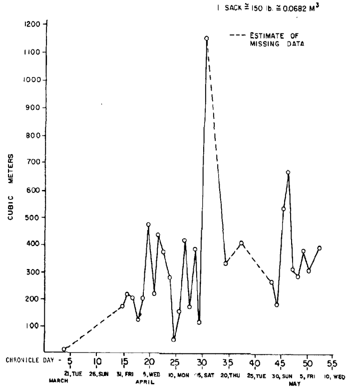
Figure 6-19. Volumes of spilled material bagged on the beach.
