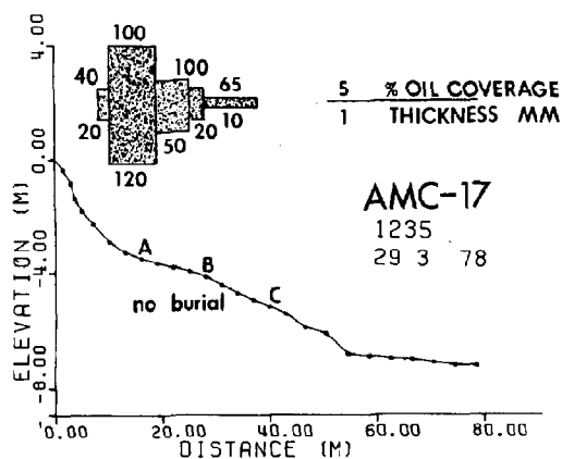
Figure 4-63. Topographic profile and oil coverage for AMC-17 on March 29.
