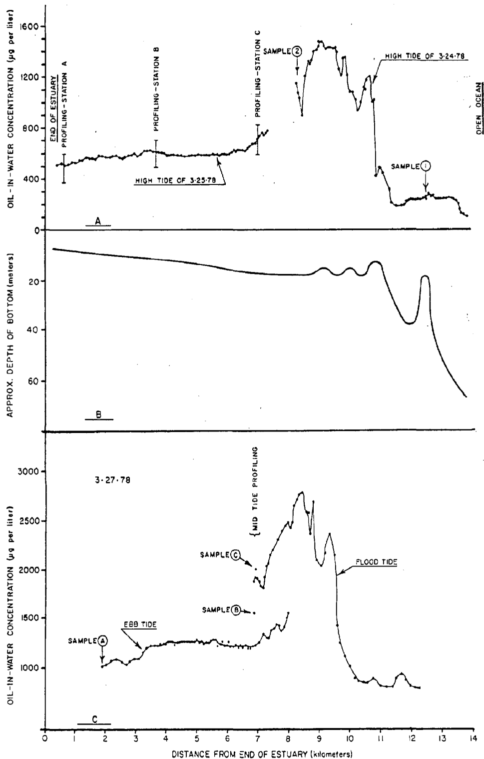
Figure 3-22. Towed underwater fluorometer transects in l'Aber Wrac'h. A: Concentration versus horizontal distance for cruises 1 and 2. B: Approximate water depth. C: Concentration versus horizontal distance for cruise 3. Concentrations determined by fluorescence do not necessarily represent the absolute concentrations of petroleum in water. (ENDECO)
