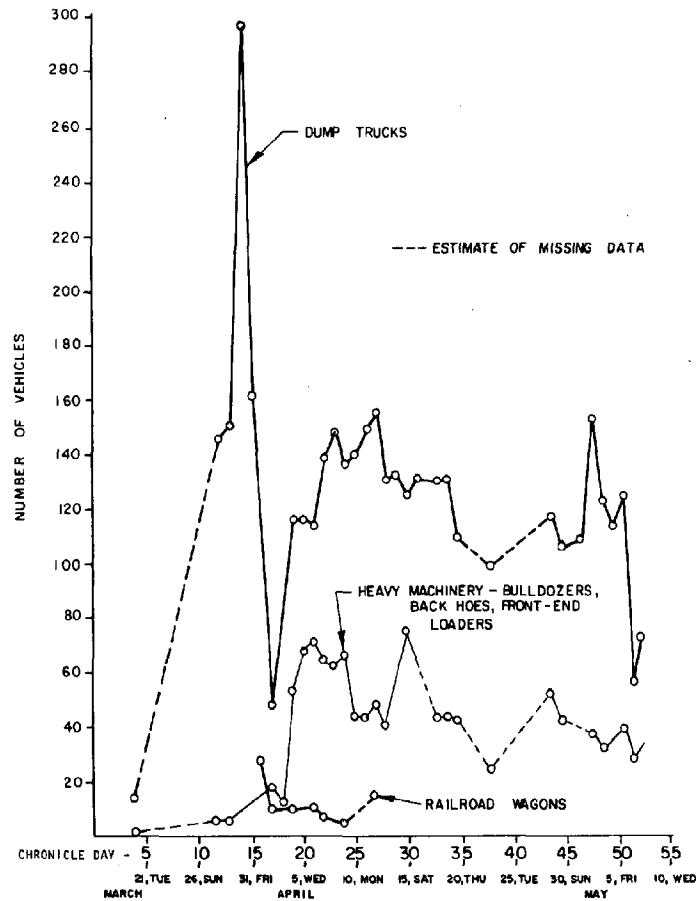
Figure 6-24. Numbers of dump trucks, heavy machinery, and railroad wagons used during spill cleanup.
