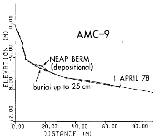
Figure 4-41. Although the beach at AMC-9 appeared clean on April 1, oil had been buried in two layers beneath the surface by formation of the neap berm.
