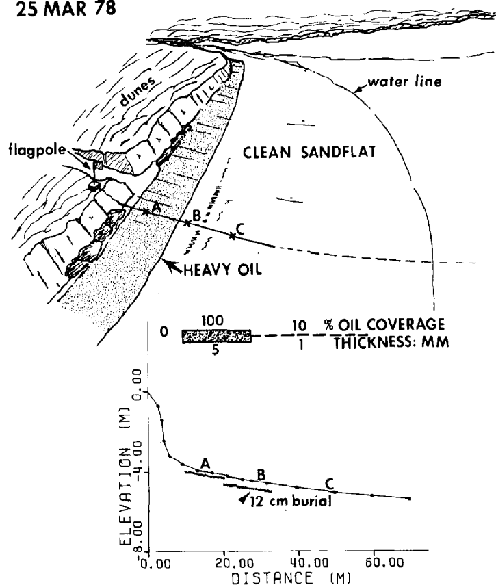
Figure 4-39. Sketch and topographic profile for station AMC-10 on March 25. All oil deposition was along the upper beach face. The total width of oil deposition on similar fine-sand beaches depends on the total quantity of oil within the area. Greater quantities will cover more of the beach face. Two distinct oil layers were buried, illustrating deposition of new sand since initial oil impact.
