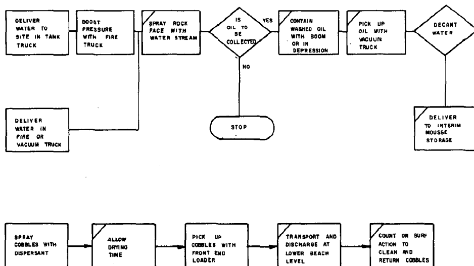
Figure 6-14. Unit process: Cleaning of walls, rockfaces, and cobbles.
