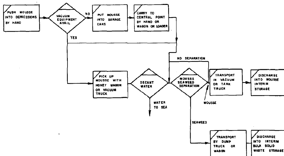
Figure 6-12. Unit process: Removal of mousse from rocky areas to interim storage.
