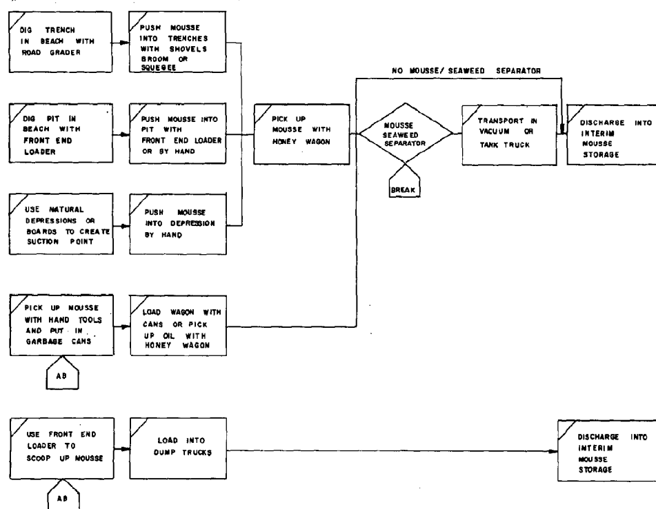
Figure 6-11. Unit process: Removal of stranded mousse from beach to interim storage.
