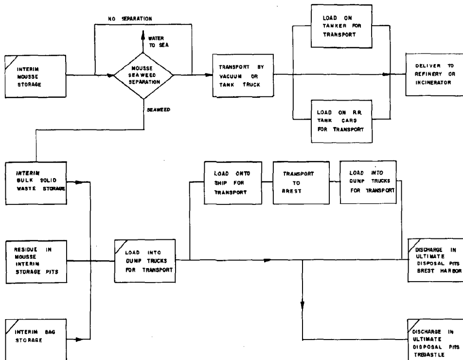
Figure 6-16. Unit process: Movement of mousse and oiled material from interim storage to disposal.
