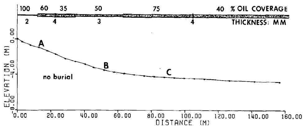
Figure 4-47. Sketch, topographic profile, and oil coverage for station AMC-6 in Roscoff on March 24. On the evening of March 24 approximately 80% of the accumulated oil was removed from the area by natural processes.
