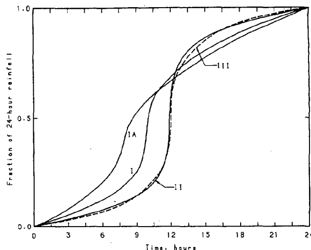
Figure B-1.—SCS 24-hour rainfall distributions.
