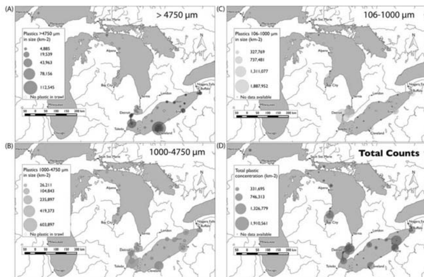
Figure 3. Maps of plastic concentrations across the lakes sampled; magnitude of concentration is depicted by size of circle around trawl location. Note, fiber counts are not included in these figures, as their quantification is error prone. (A) Mapped counts of plastic litter >4,750 \mu\text{m} . (B) Mapped counts of plastic litter 1,000\text{--}4,750 \mu\text{m} . (C) Mapped counts of plastic litter 106\text{--}1,000 \mu\text{m} . (D) Total mapped counts for the stations where all three size classes were quantified.
