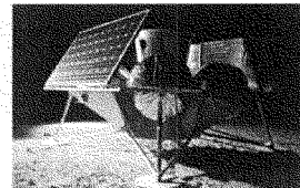
Lunar analogue testing with lander & rover prototypes
