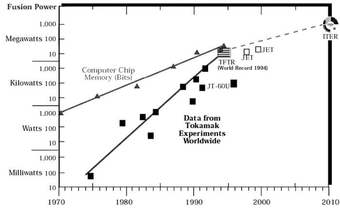
Fusion power produced (red curve) versus year. For comparison, the progress in computer chip memory is also shown, illustrating that fusion power has climbed even more steeply.
