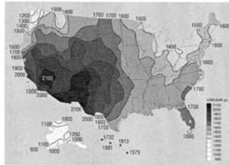
Figure 3: U.S. Insolation
