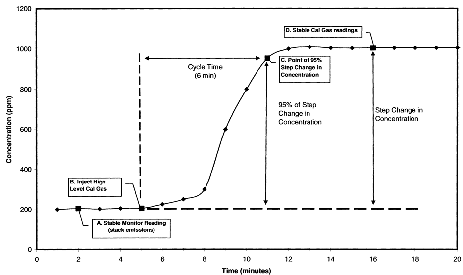
Figure 6a. Upscale Cycle Time Test
