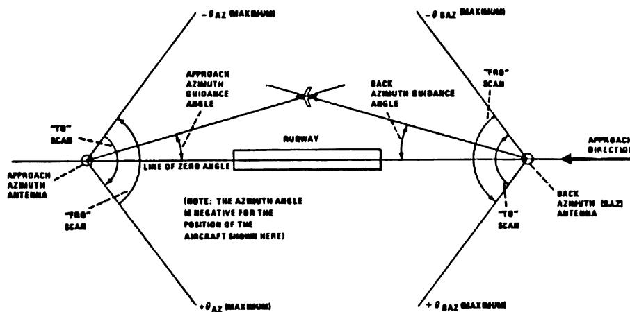
Figure 12. Azimuth Guidance Functions Scanning Conventions
