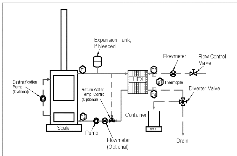
Figure 2. Schematic of Test Equipment Set-up
