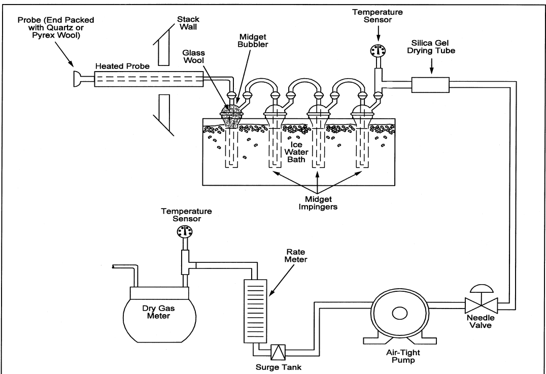
Figure 6-1. Sulfur Dioxide Sampling Train.
