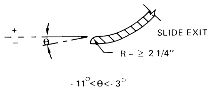
FIG. J RUNWAY EXIT ANGLE \theta
