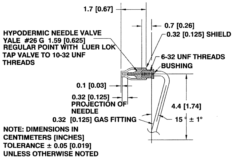
AN EXAMPLE OF A TYPICAL IGNITER FIGURE 6
