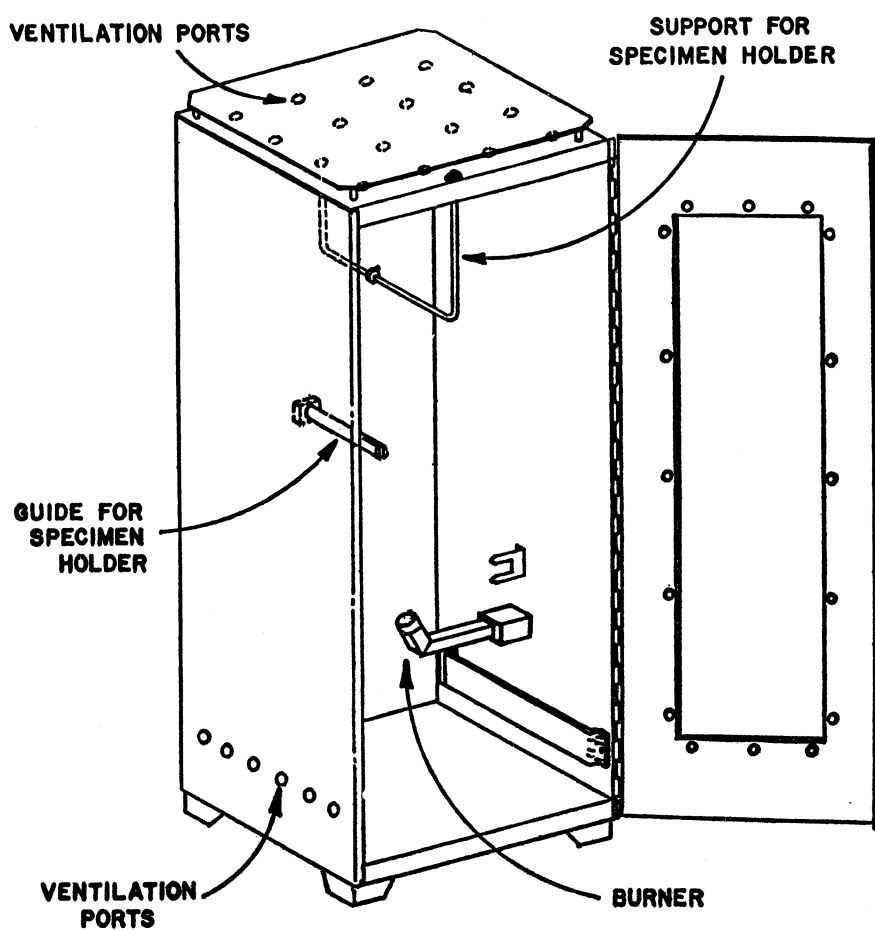
VERTICAL TEST CABINET
