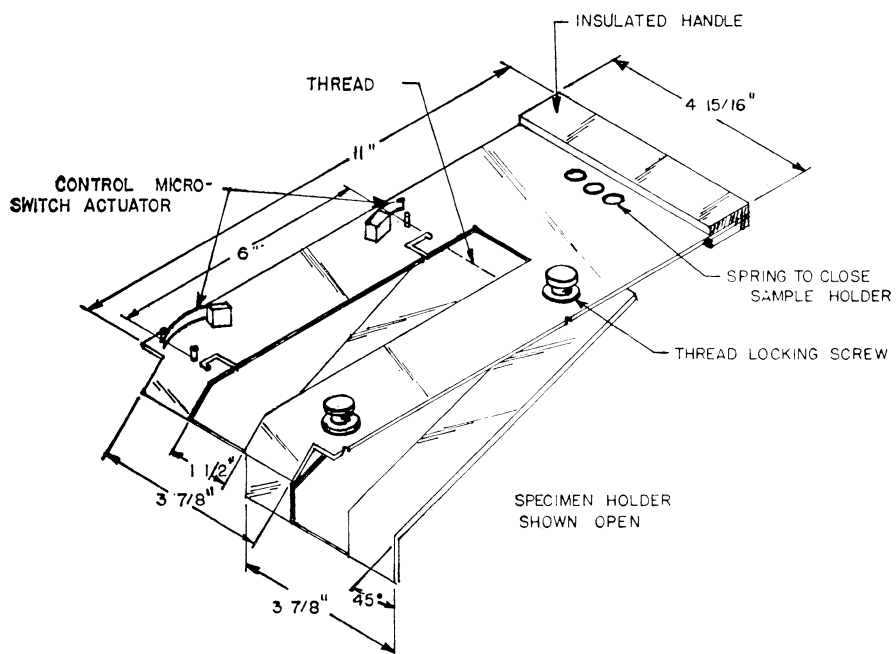
FIGURE 2 —Specimen holder
